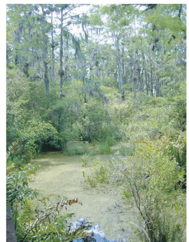
Freshwater swamp in Loxahatchee National Wildlife Refuge.
