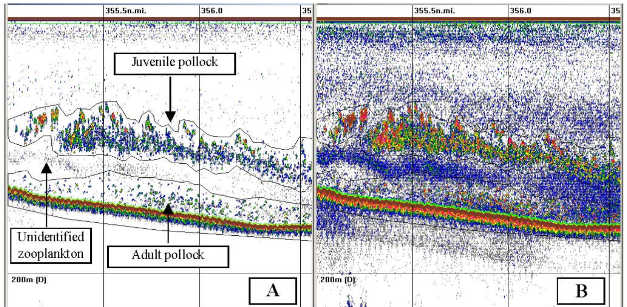
Figure 1.--Example of thresholding on pollock echo sign using (A) the standard s_v threshold of -70 dB and (B) a decreased s_v threshold of -80 dB.. Data were collected during August 2001 off Kodiak Island, Alaska.
