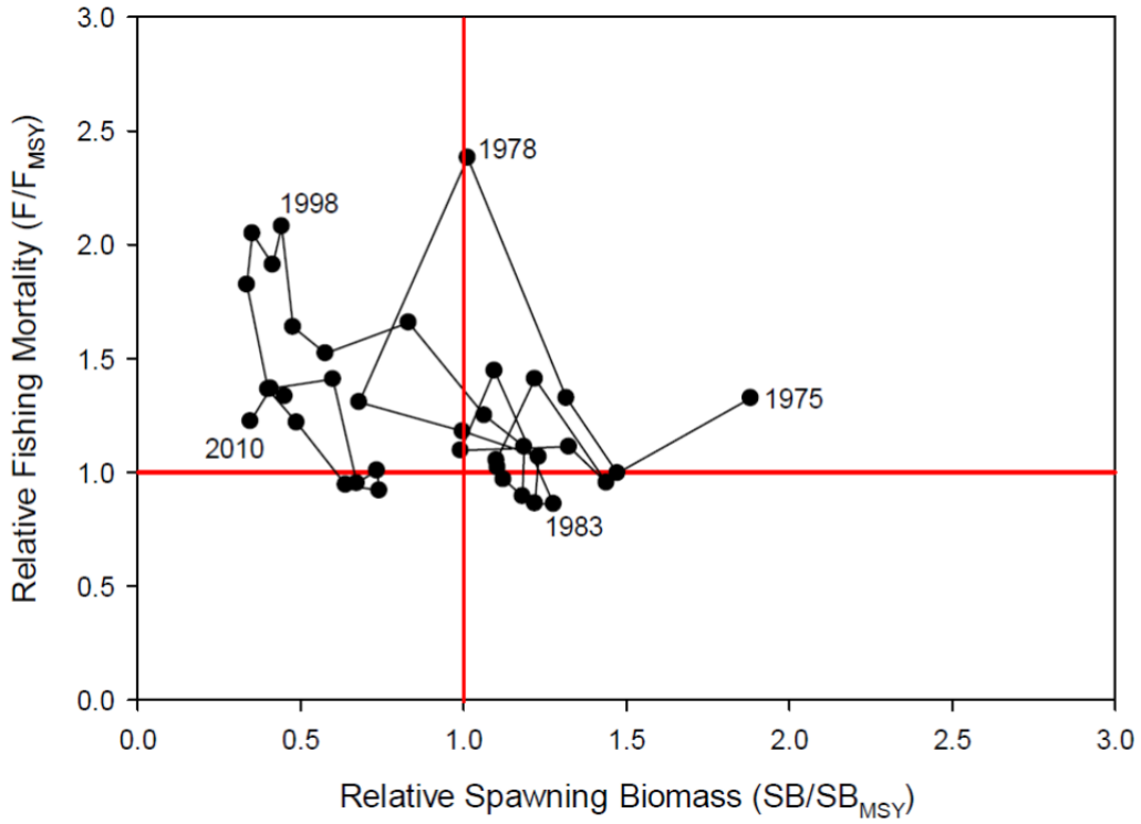
Figure D. Kobe plot of the trends in estimates of relative fishing mortality and relative spawning biomass of Western and Central North Pacific striped marlin ( Kajikia audax ) during 1975-2010.
