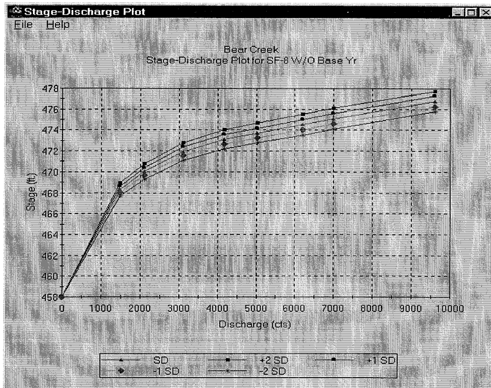
Figure 7. Stage-Discharge Plot
