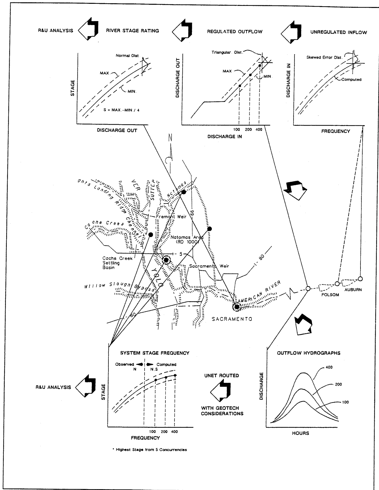
Figure 4 - Schematic of Hydrologic Analysis Components
