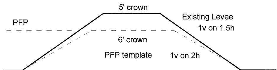
Figure 2. Template for PFP - clay levee
