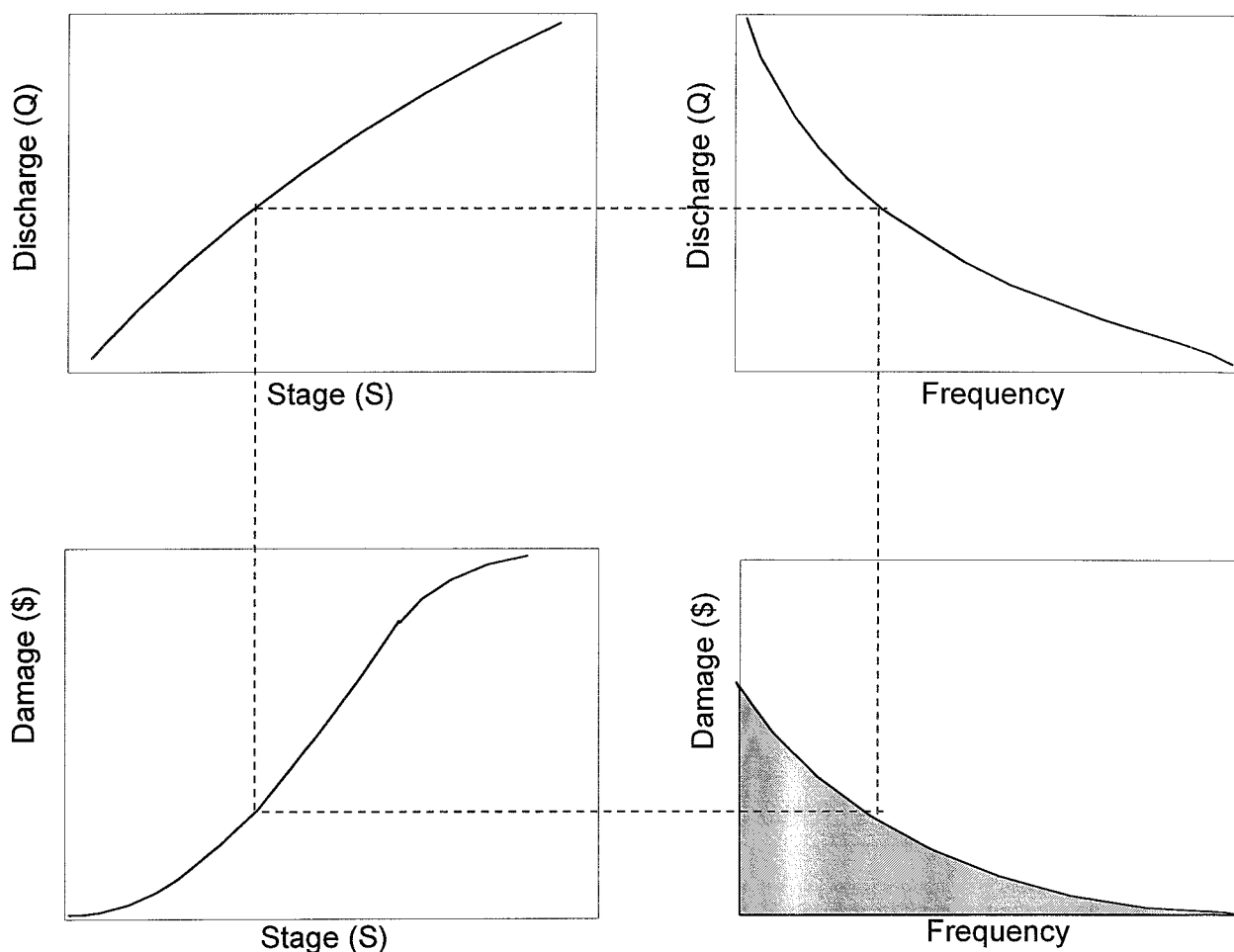
Figure 2: Frequency-Damage Estimation
