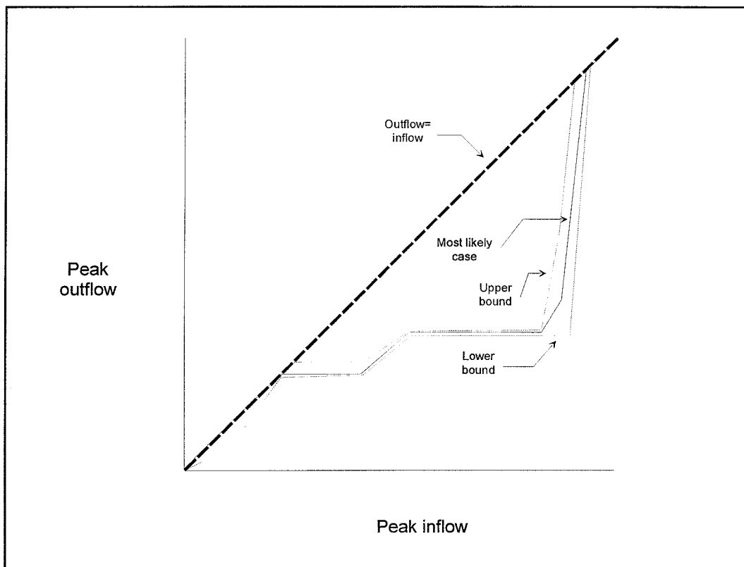
Figure 5 - Example Inflow-Outflow Function with “Confidence Bands”
