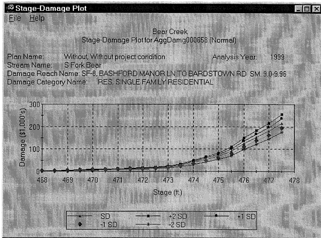
Figure 11. Stage Damage Function with Uncertainty
