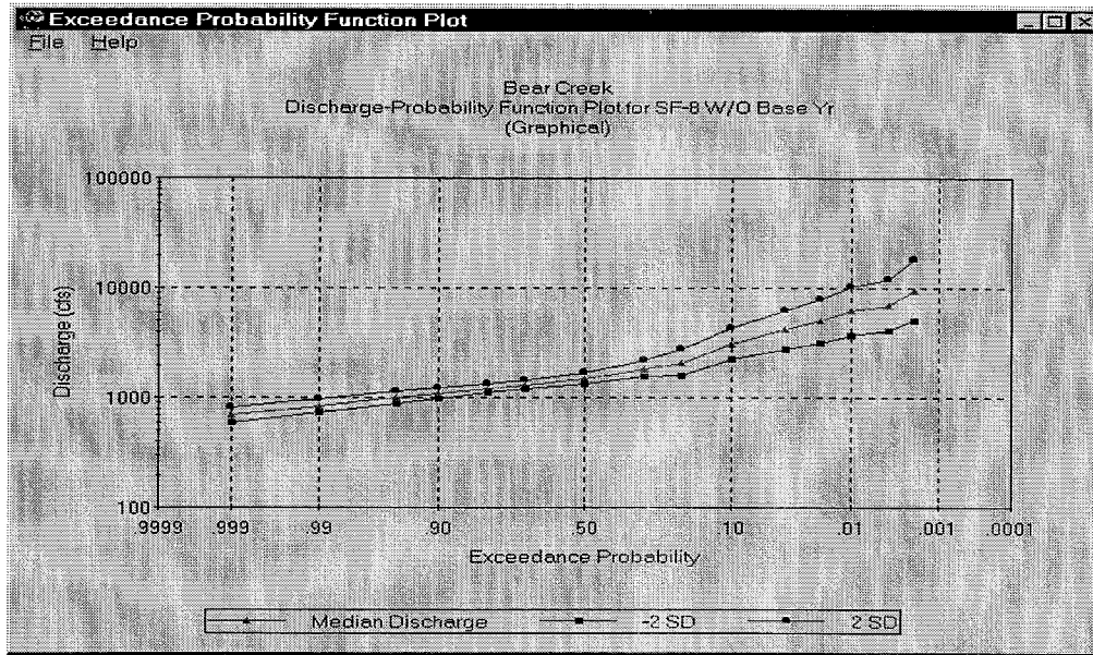
Figure 6. Plot of Exceedance-Probability Function
