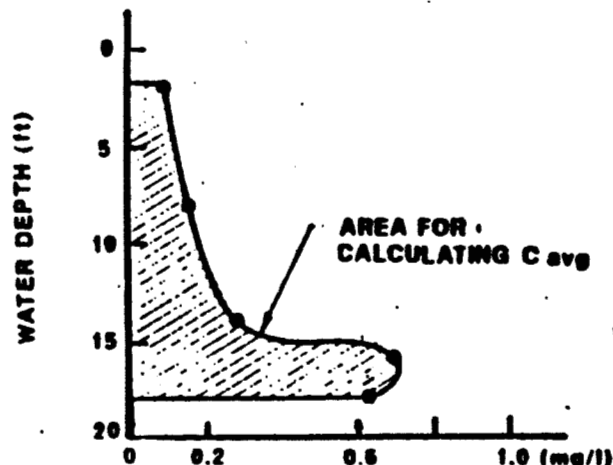
OZONE CONCENTRATION
