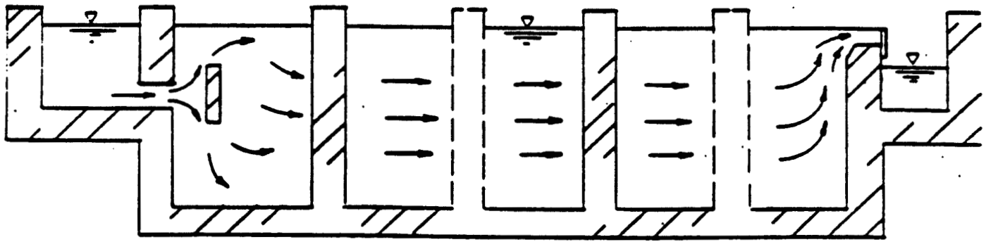
SECTION
