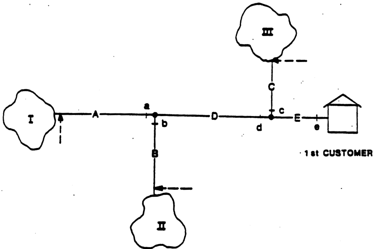
FIGURE 3-3 MULTIPLE COMBINATION POINTS FOR INDIVIDUALLY DISINFECTED SURFACE SOURCES
