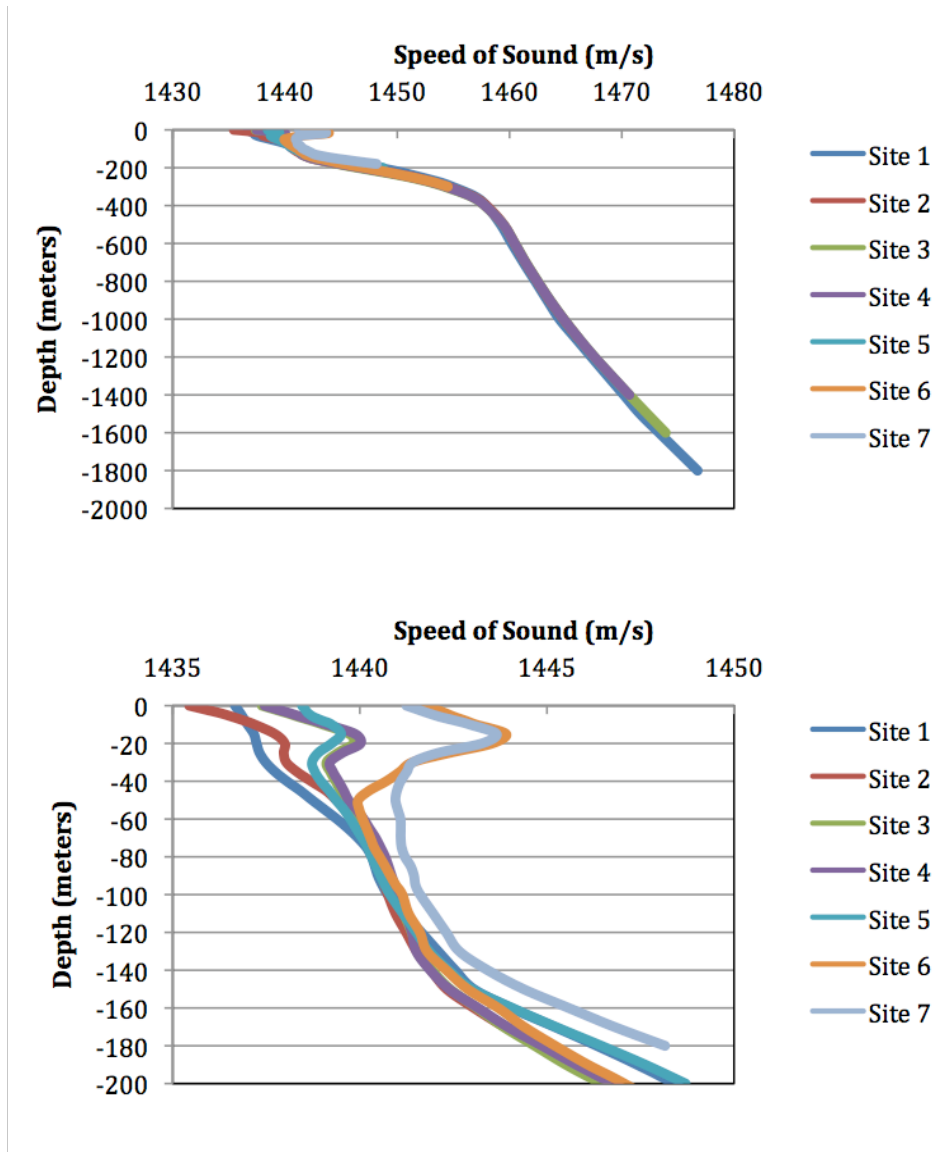
FIGURE 5. The sound velocity profiles used for each modeling site are shown above. The top panel shows the full depth of the profile. Because there is very little variation at depth, the bottom panel shows the upper 200 meters of each profile.
