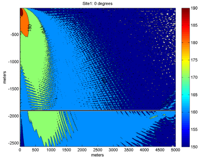
Figure 7.1. Transmission Loss along 0 degree radial (fore-aft), contoured into 10 dB steps.
