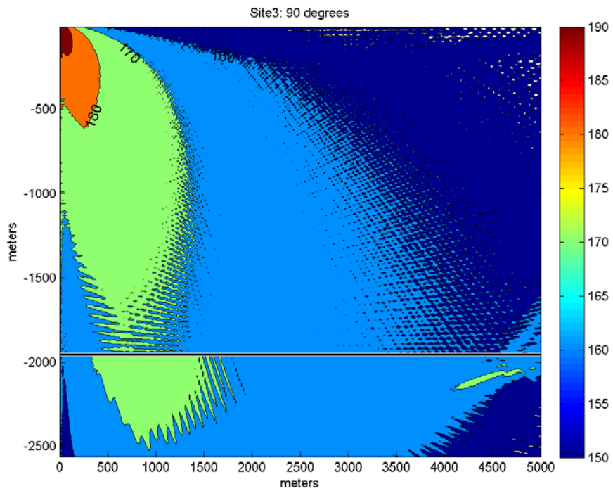
Figure 9.2. Transmission Loss along 90° radial (athwartship), contoured into 10 dB steps.
