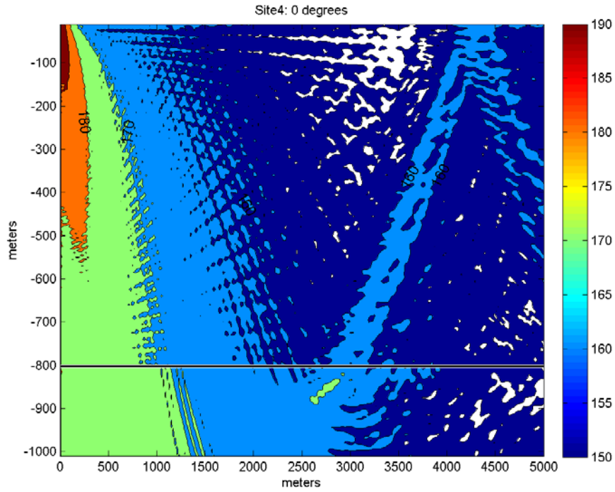
Figure 10.1. Transmission Loss along 0 degree radial (fore-aft), contoured into 10 dB steps.
