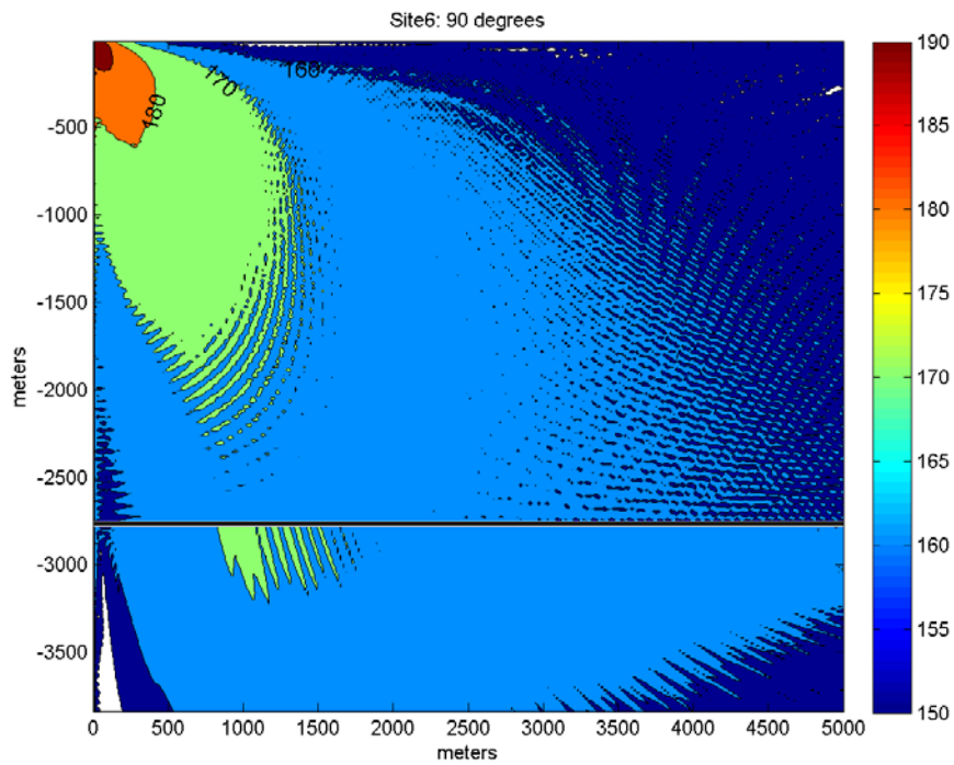
Figure 12.2. Transmission Loss along 90° radial (athwartship), contoured into 10 dB steps.
