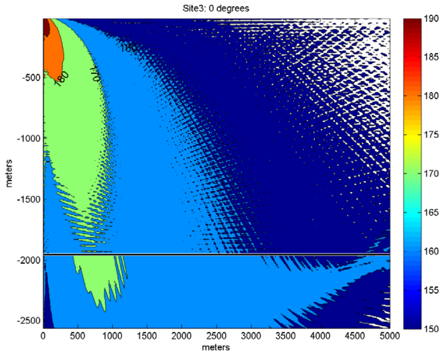
Figure 9.1. Transmission Loss along 0 degree radial (fore-aft), contoured into 10 dB steps.
