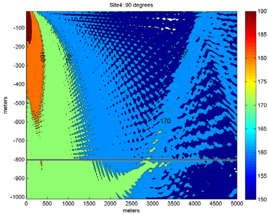
Figure 10.2. Transmission Loss along 90° radial (athwartship), contoured into 10 dB steps.
