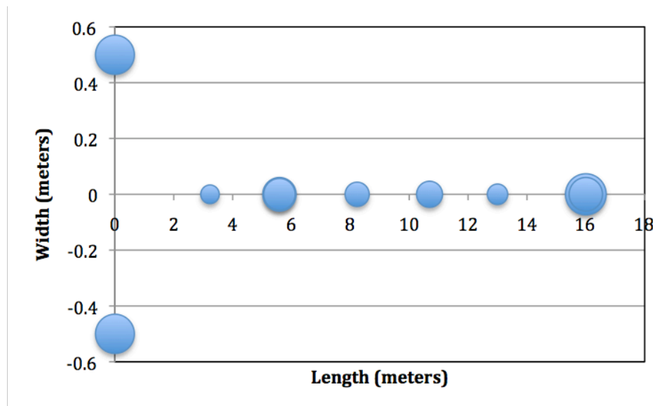
FIGURE 1. A graphical representation of the R/V Langseth 1830 cu. in. airgun array configuration. The size of the marker is proportional to the cube root of the airgun volume.
