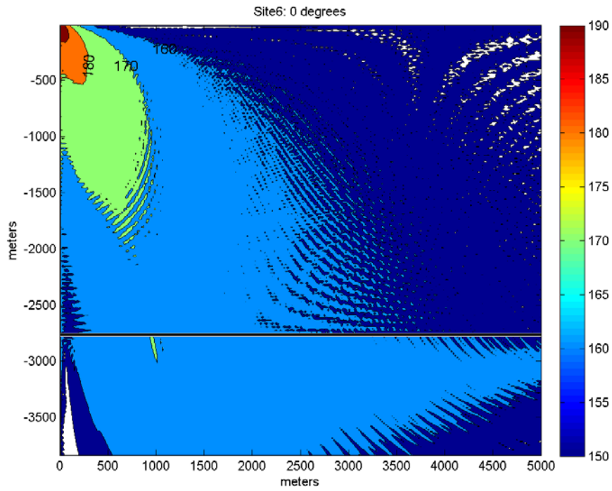
Figure 12.1. Transmission Loss along 0 degree radial (fore-aft), contoured into 10 dB steps.
