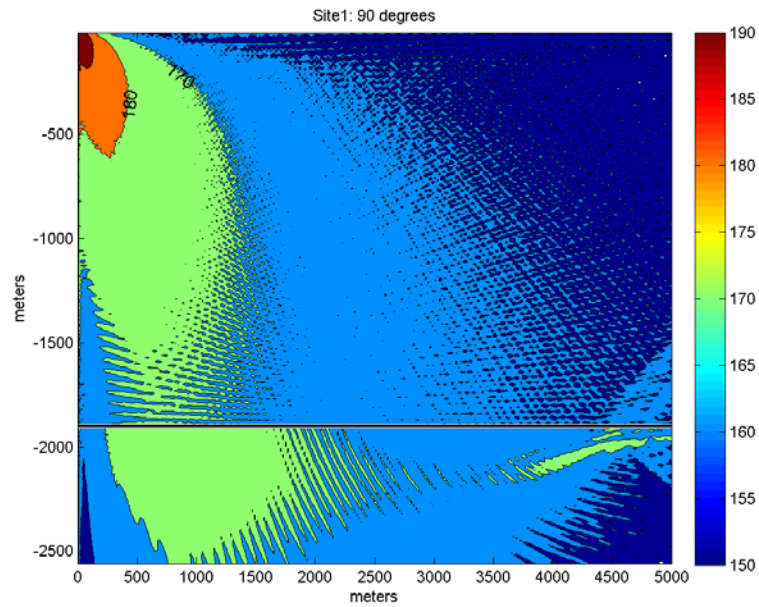
Figure 7.2. Transmission Loss along 90° radial (athwartship), contoured into 10 dB steps.
