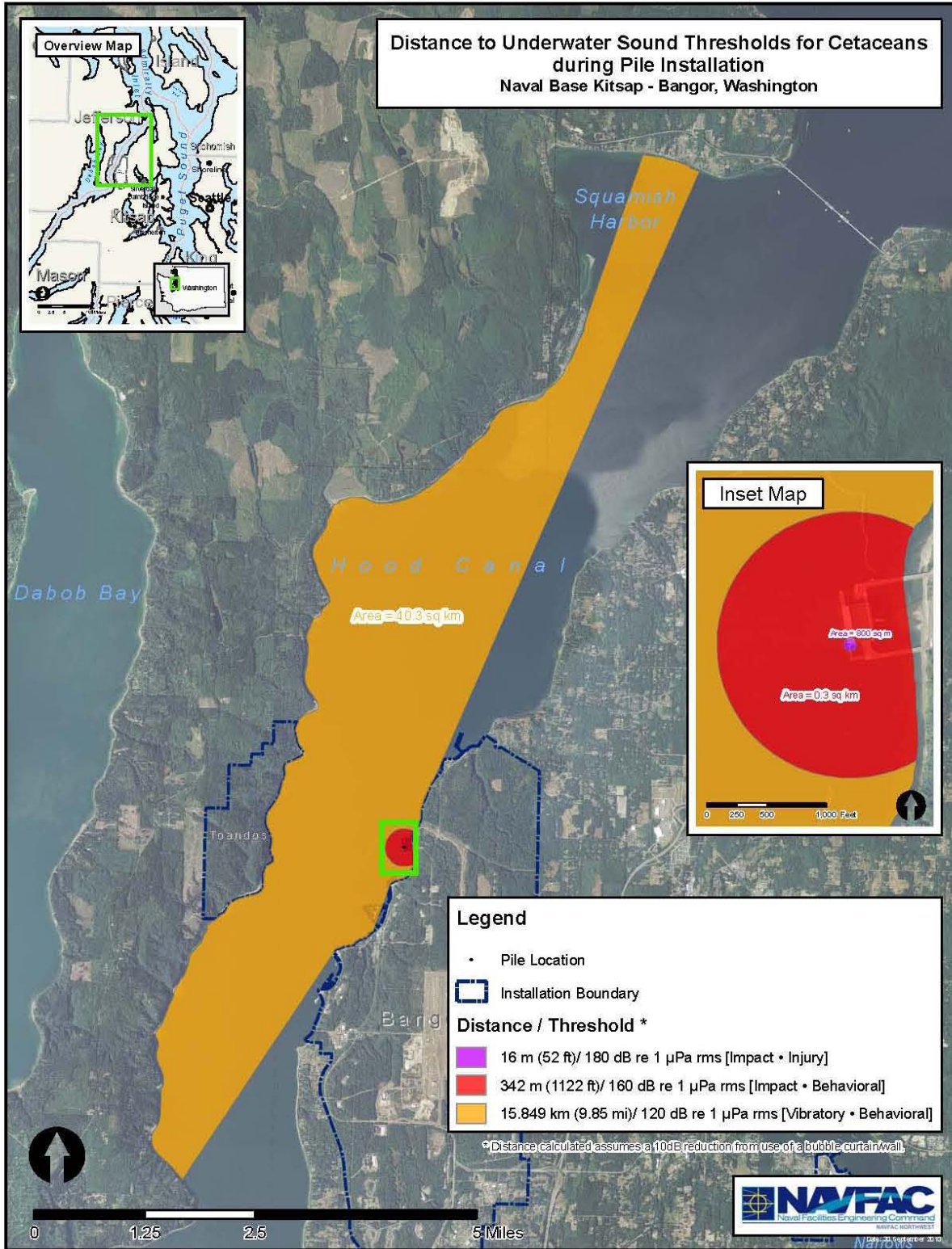
Figure 6-1 Distance(s) (m) to Underwater Sound Thresholds for Cetaceans from Impact & Vibratory Pile Driving During Pile Installation
