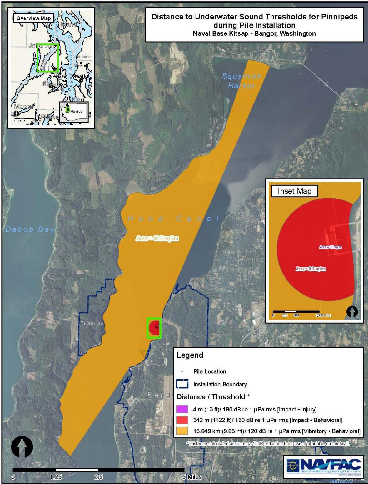
Figure 6-2 Distance(s) (m) to Underwater Sound Thresholds for Pinnipeds from Impact & Vibratory Pile Driving During Pile Installation
