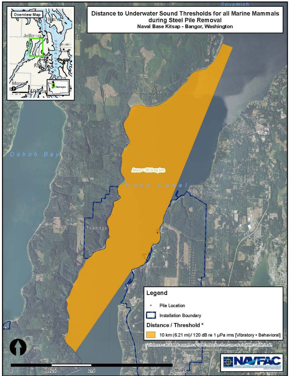
Figure 6-3 Distance(s) (m) to Underwater Sound Thresholds for all Marine Mammals from Vibratory Pile Driving During Steel Pile Removal
