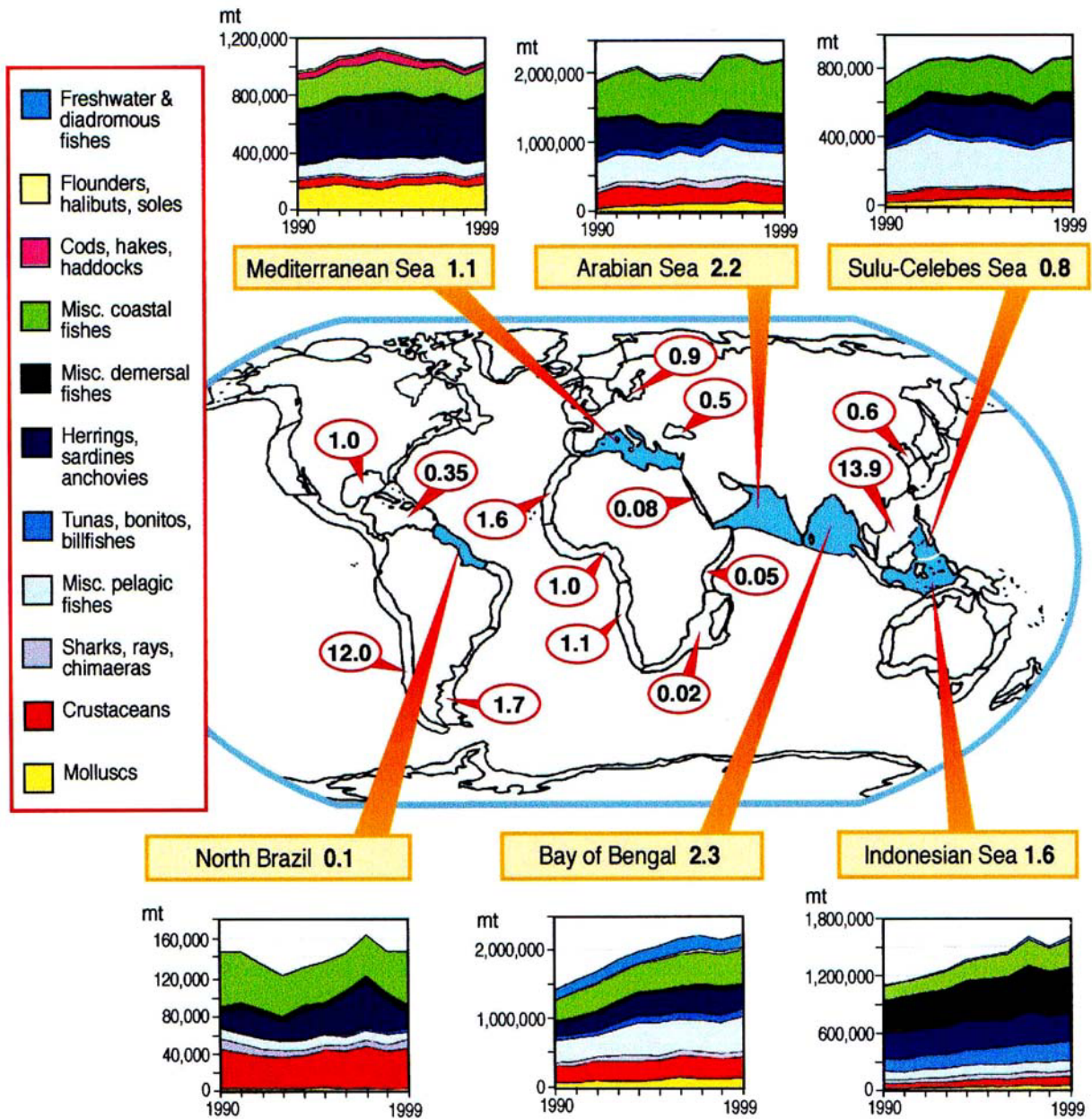
Figure 7. Decadal trends (1990-1999) in biomass yields (mmt) of the six candidate LMEs for precautionary approach actions to preclude total fish biomass reductions. (Value after LME name represents 1999 biomass yield level. Data are based on FAO statistics, as reported to the FAO by official national sources, in Garibaldi and Limongelli (2003). Unfortunately, fisheries effort data are not available for trend analyses. Reproduced with permission from FAO.)
