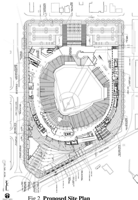
Fig 2 Proposed Site Plan
