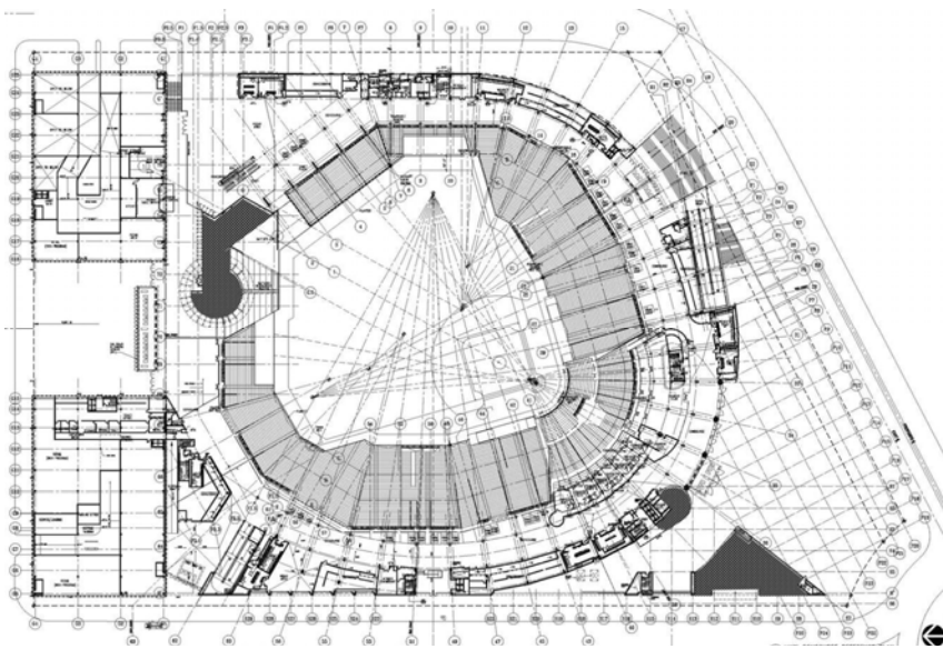
Fig 16 Base Plan and Opt 1 & 2 Preferred Uses – Main Concourse Level
