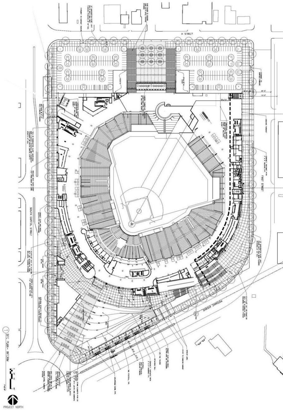
Fig 4 Proposed Site Plan
