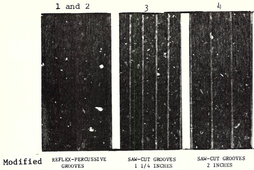
FIGURE 4. VARIOUS TEST SECTIONS OF THE 300-FOOT ASPHALTIC CONCRETE TEST BED (EACH SECTION IS 40 FEET LONG)
