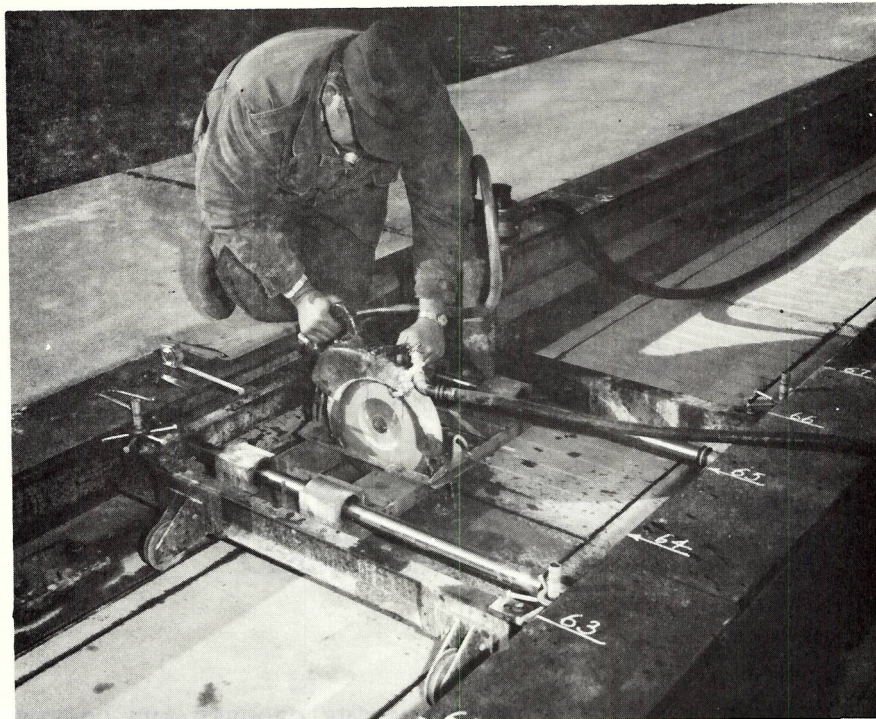
FIGURE 7. MACHINE FOR INSTALLING SAW-CUT GROOVES IN THE TEST SECTIONS
