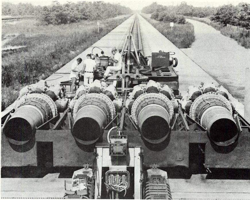
FIGURE 1. JET-POWERED PUSHER CAR FOR PROVIDING PRESELECTED SPEEDS TO TEST EQUIPMENT
