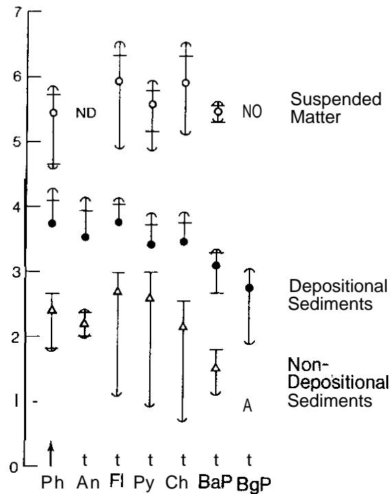
FIGURE 12.-- Measured partition coefficients. Open circles represent the log of the mean K_p measured for particulate:dissolved data, solid circles are depositional sediments:porewater, and open triangles for nondepositional sediments:pore water. The straight horizontal lines represent 1 standard deviation and the curved symbols are the values of the maximum and minimum K_p s measured for each compound. Overlapping information between the deposi- t&mat and nondepositional data were eliminated for clarity.
