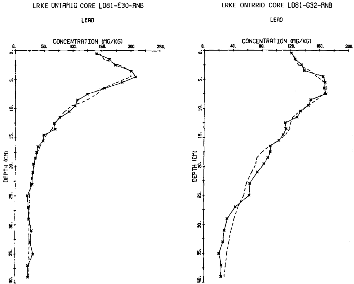
FIGURE 38.--Vertical distribution of stable lead in the Lake Ontario cores. The solid lines connect data points, while the dashed lines are the distributions predicted on the basis of lead atmospheric emissions inventories and the steady-state mixing model. The sedimentation rate is fixed in each case by the lead-210 data. Recent decreases in the use of leaded gasoline are reflected both in the emissions inventory and in sediment lead profiles. The excellent quality of the model fits encourages use of refined models to treat distributions of contaminants with more poorly known loadings and more complex sedimentary behavior. (Data of R. Rossmann/K. Johansen; model of J. Robbins.)
