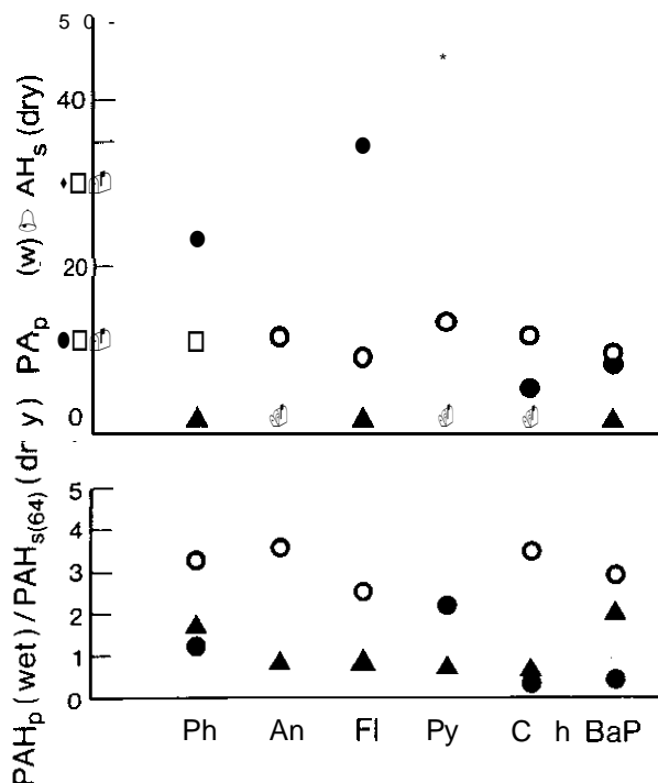
FIGURE 51.--Top: ratio of Pontoporia hoyi PAH to sediment PAH (● = 24-m station; ○ = 45-m station; ▲ = 60-m station). Bottom: same ratio; sediment corrected for 64 \mu\text{m} grain size.
