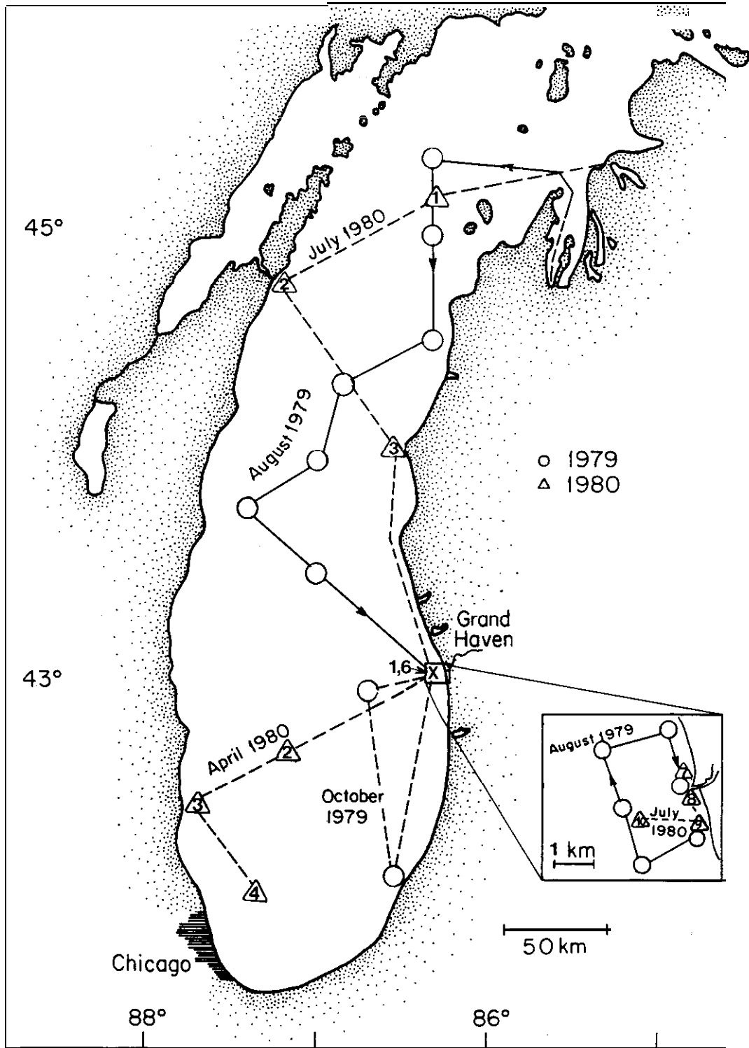
FIGURE 2.--Cruise tracks and sampling stations occupied in 1979 and 1980 for collection of microlayer and subsurface water from Lake Michigan. The solid arrows connecting the circles indicate that air sampling results are available for this cruise. The numbered stations refer to figures 3-5.
