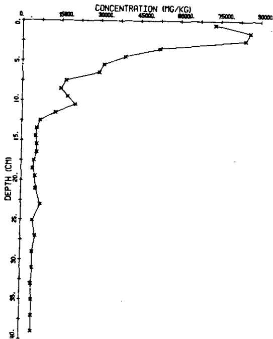
FIGURE 35.--Vertical distribution of inorganic carbon and calcium in the Lake Ontario cores. These strongly varying constituents constitute a significant mass of the sediments. Proper modeling of sedimentation, reworking, and geochronology must include a treatment of such profiles. (Data of R. Bourbonniere/R. Rossmann.)
