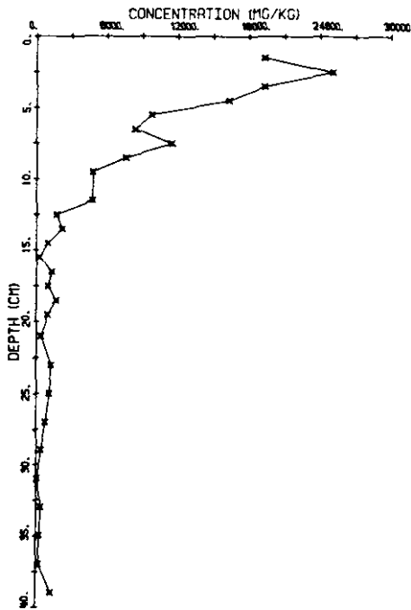
LAKE ONTARIO CORE L081-E30-RNB
