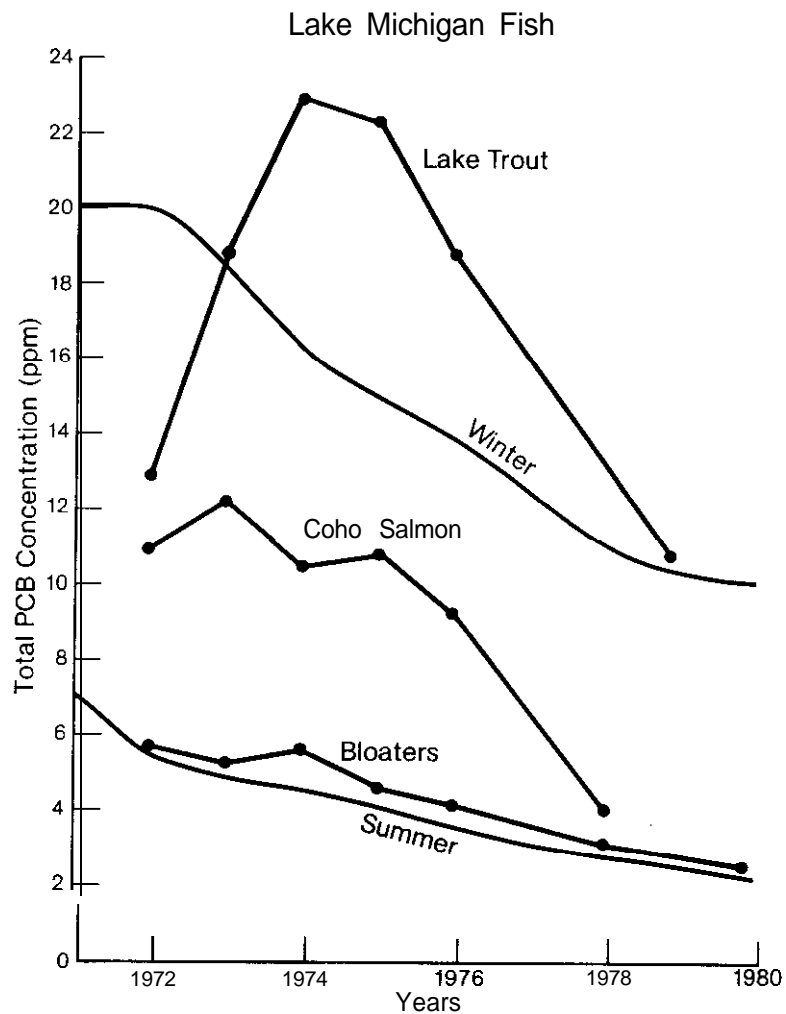
FIGURE 66.--Total PCBs in Lake Michigan fish . Data are from Konasevich et al. (1978) and IJC (1979) . The model outputs for biota from the runs illustrated in figures 1A and 2B are shown as smooth curves.
