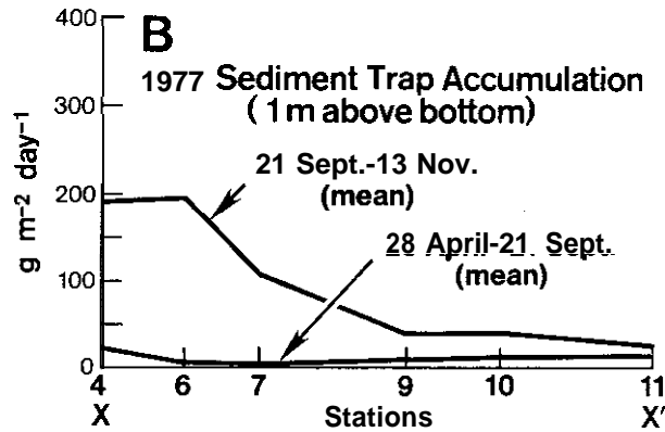
FIGURE 26.--Seasonal sediment trap accumulation rates at 1 m off the bottom for 1977 (A). Transect of mean nonstorm (April-September) and storm (September-November) particle fluxes (B). Transect X to X' shown in upper left of figure 26(A). Units are g\ m^{-2}\ day^{-1} (from Chambers and Eadie, 1981).
