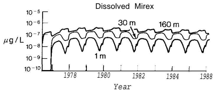
FIGURE 60.--Simulation of dissolved mirex.
