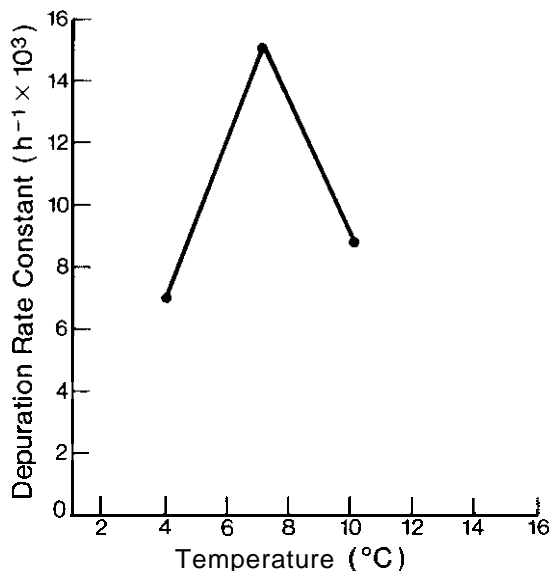
FIGURE 44.--Temperature variation of the depuration rate constants for anthracene by Pontoporeia hoyi .
