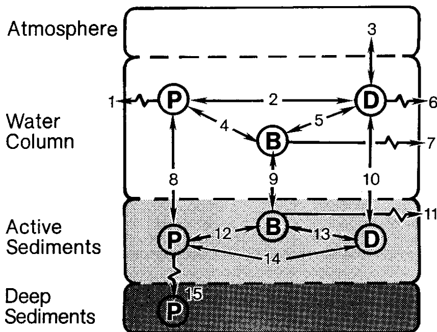
FIGURE 1.-- Conceptualized toxic system model. P represents particle phase, D represents dissolved phase, and B is an abbreviated food web. The 15 process arrows are: photolysis (1 and 6), sorption (2 and 14), air-water exchange (3), grazing and fecal pellet generation (4), filtering (5), biological decomposition (7 and 11), settling and resuspension (8), food web dynamics (9), advective and diffusive mixing (10), benthos-sediment interactions (12 and 13), and burial and bioturbation (15).
