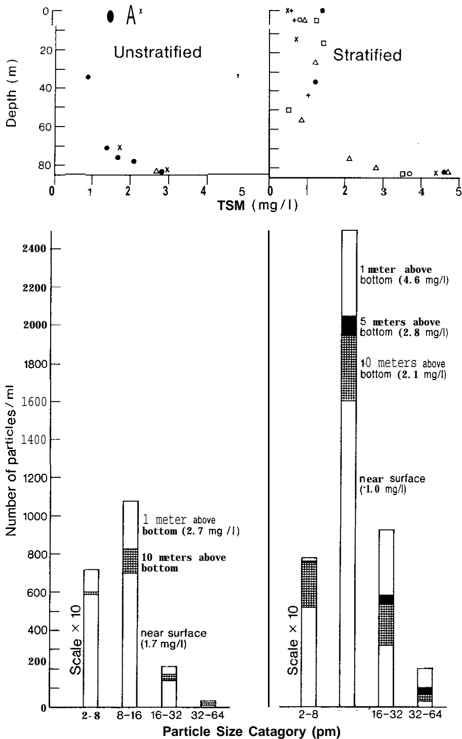
FIGURE 28.--Composite profiles of total suspended matter for the unstratified (A) and stratified (B) periods at station 7/8. (For location, see figure 22.1 The unstratified composite represents three sets and the stratified composite represents five sets of samples. Characteristic particle-size distribution profiles for the unstratified (C) and stratified (D) periods at the same location. Size data were determined on a HIAC® instrument. The number of particles at each depth (within each size category) are cumulative. In all cases, the samples collected near the surface had the smallest number of particles per milliliter, while the sample from 1m above the bottom had the greatest number (from Eadie et al., 1982c).
