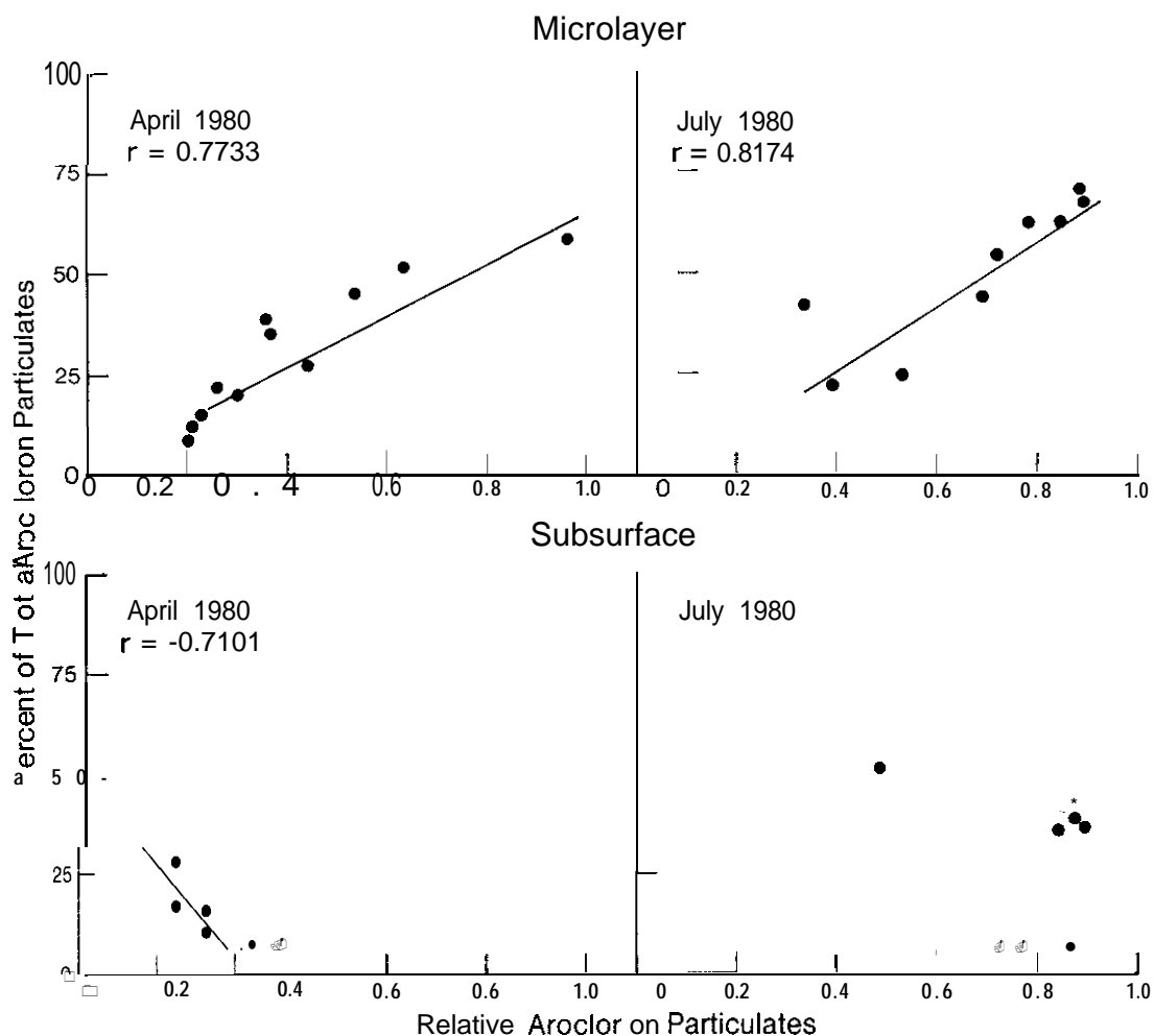
FIGURE 4.--Correlation between the amount of total PCB associated with the particulates in the microlayer samples from April 1980 and July 1980 versus the percentage of the total amount of the PCB on the particles that was measured as Aroclor® 1242.
