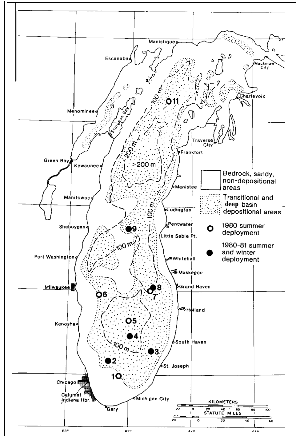
FIGURE 22.--Station locations during the suspended particulate flux study in 1980-81, and their relation to depositional areas (after Cahill, 1981.1)
