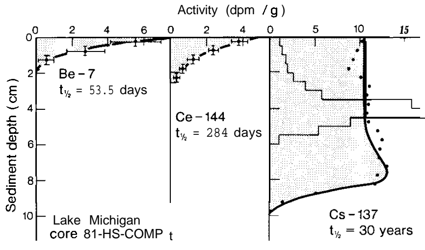
FIGURE 33.--Distribution of beryllium-7, cerium-144, and cesium-137 in a high sedimentation rate core from Lake Michigan. While cesium-137 appears uniformly mixed, the two short-lived isotopes are not. The uniform mixing model can only apply to processes occurring on time scales of decades. (Data and model of J. Robbins.)
