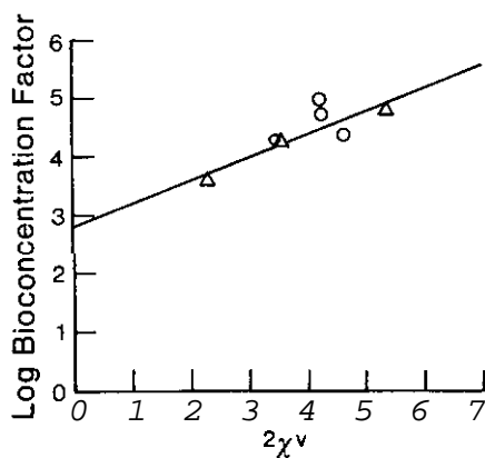
FIGURE 53.--Log bioconcentration factor for PAH in Pontoporeia hoyi versus the second order molecular connectivity term ( 2\chi^v ).
