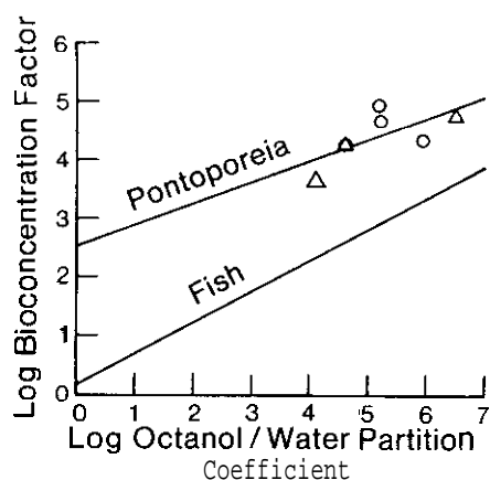
FIGURE 52.--Log of bioconcentration factor for PAH in Pontoporeia hoyi versus log octanol water partition coefficient compared with the similar relationship for fish from (Kenaga and Goring, 1979).
