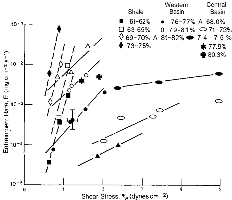
FIGURE 19.--Entrainment rates for three sediment types at various water contents as a function of applied shear stress (from Fukuda, 19781).
