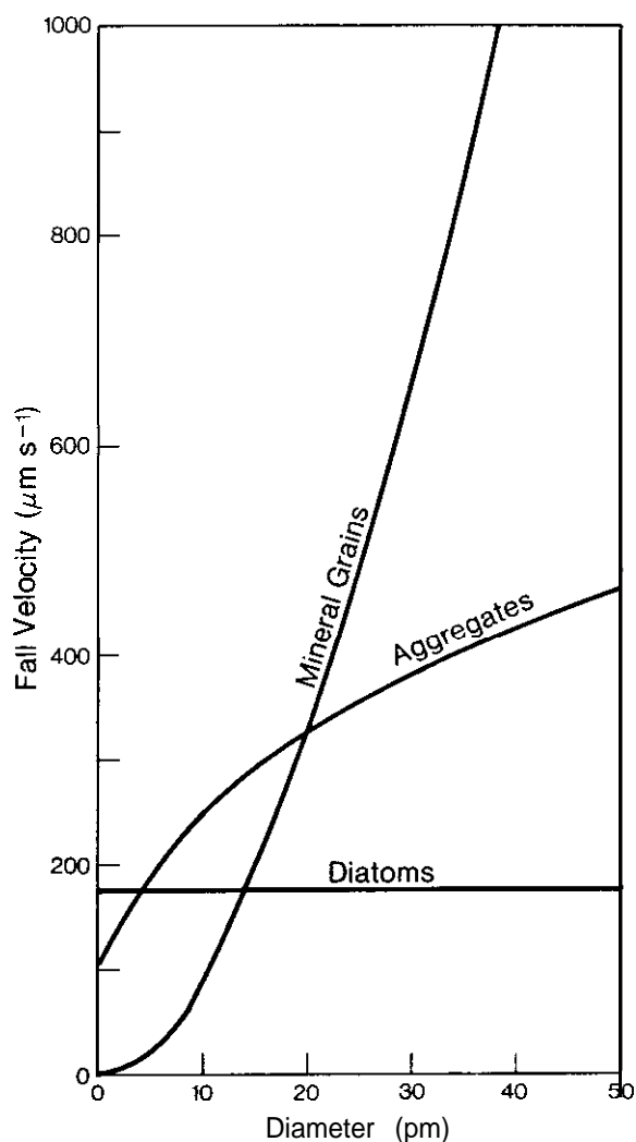
FIGURE 17.--Fall velocity as a function of particle size (from Hawley, 1982b).
