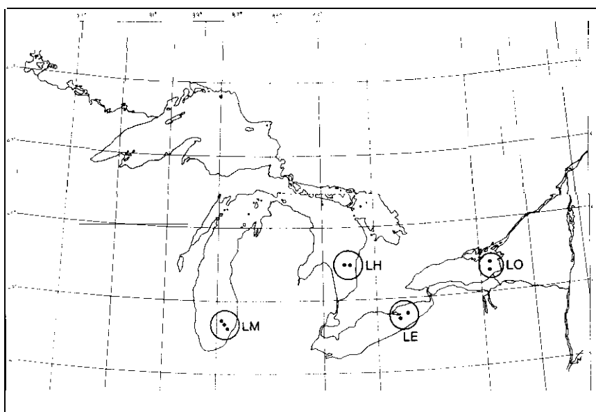
FIGURE 30.--Locations of cores collected in 1981 (Lake Ontario, CSS Limnos; other lakes, R/V Roger R. Simons).
