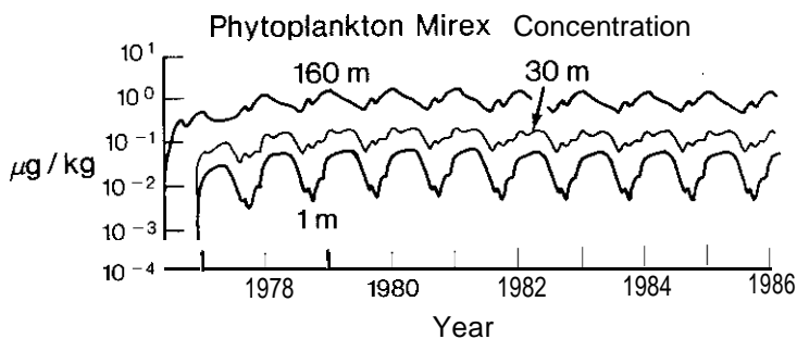
FIGURE 56.- Simulation of phytoplankton mirex.
