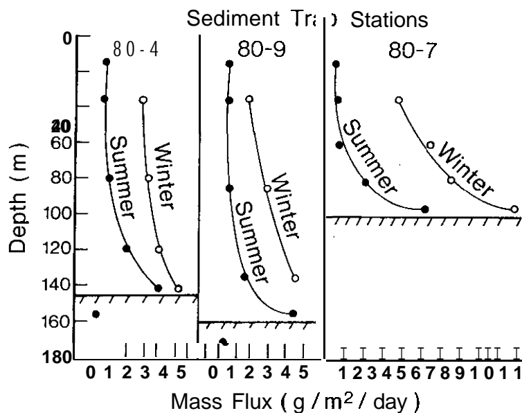
FIGURE 27.--Particle mass flux profiles from three trap profiles in Lake Michigan. (See figure 22.1 Summer profiles represent the period mid-June through mid-November; winter profiles represent the period mid-November through mid-June. Sediment accumulation rates are from local cores measured by Edgington and Robbins (1976) (from Eadie et al., 1982c).
