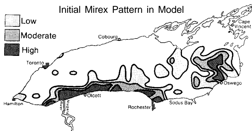
FIGURE 69.--Initial distribution of sedimentary mirex, based on the data in Holdrinet et al. (1978).
