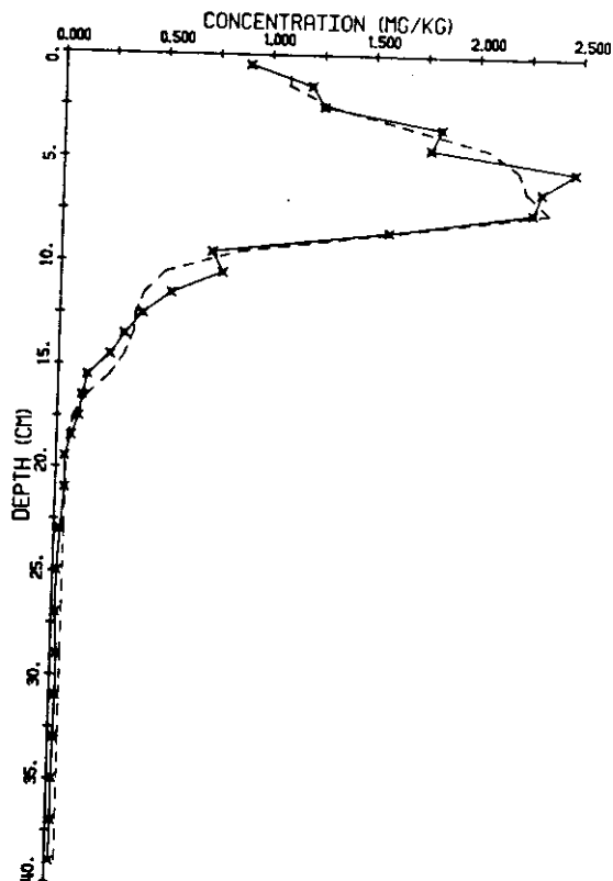
FIGURE 39.--Vertical distribution of mercury in the two Lake Ontario cores. As the flux to this area is not known, it is inferred from the high sedimentation core (G32), assuming no remobilization. The dashed line in the left panel is the flux expected in core E30 using that from G32. The agreement with experimental results implies limited mobility of mercury in these sediments. (Data of R. Rossmann/K. Johansen; model of J. Robbins.)
