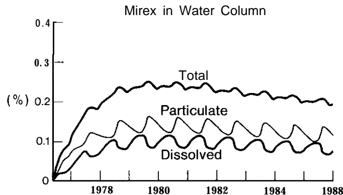
FIGURE 61.--Model approximation of percent total of water column mirex relative to sediments.
