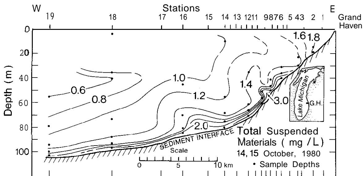
FIGURE 29.--Total suspended matter contours (mg L -1 ) during an upwelling event. A comparison with transparency and temperature profiles shows suspended materials being transported up the slope into the nearshore area then lakeward in the epilimnion. Water samples were collected at each dot (from Bell and Eadie, 1982).
