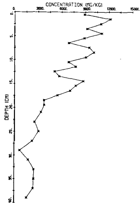
LAKE ONTARIO CORE L081-G32-RNB
