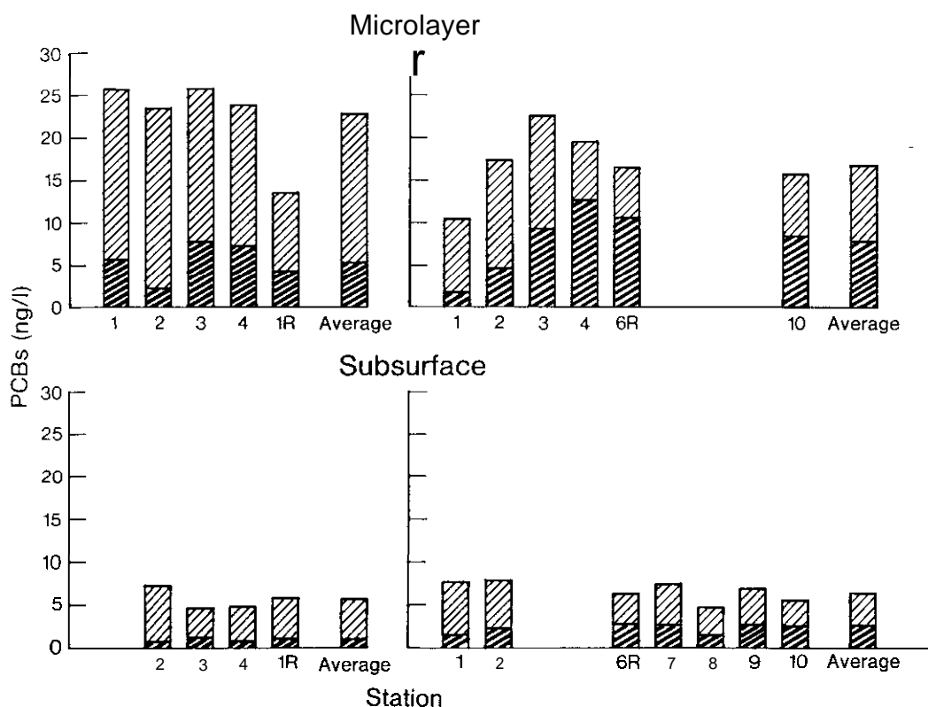
FIGURE 3.--The particulate and dissolved distributions of total PCB in samples of surface microlayer and subsurface water from Lake Michigan. The station numbers refer to the stations identified in figure 2.
