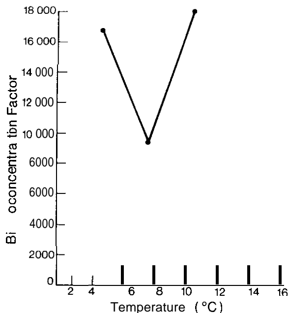
FIGURE 45.--Temperature variation of the predicted bioconcentration factor for anthracene by Pontoporeia hoyi .
