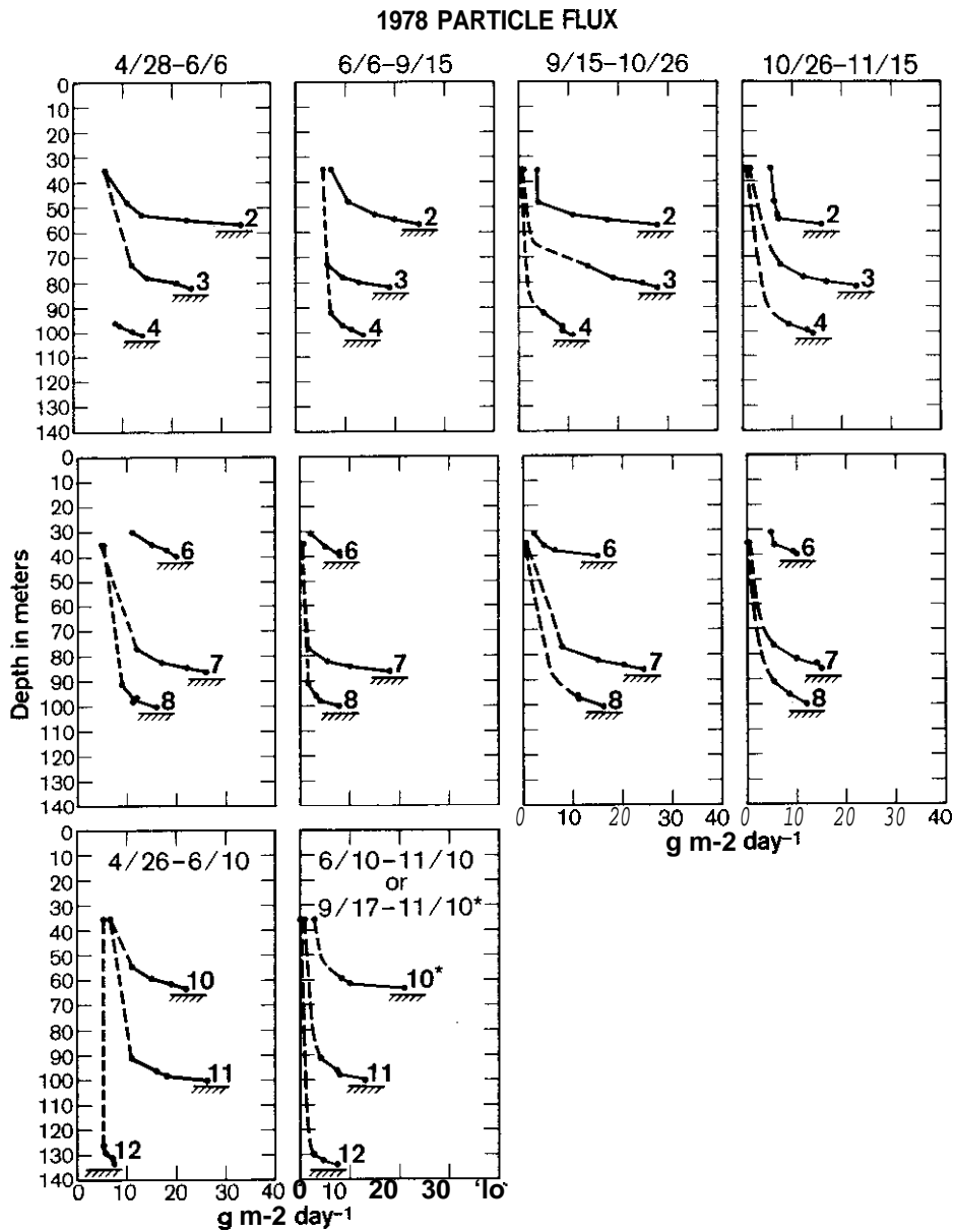
FIGURE 25.--Particle flux profiles of the 1978 sediment trap data. Units are g\ m^{-2}\ day^{-1} . The numbers correspond to 1978 station locations. (See figure 22.1 The profiles are nearly exponential, with a resuspension scale length of approximately 6 m (from Chambers and Fadie, 1981).
