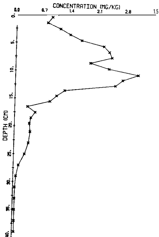
FIGURE 39.--Vertical distribution of mercury in the two Lake Ontario cores. As the flux to this area is not known, it is inferred from the high sedimentation core (G32), assuming no remobilization. The dashed line in the left panel is the flux expected in core E30 using that from G32. The agreement with experimental results implies limited mobility of mercury in these sediments. (Data of R. Rossmann/K. Johansen; model of J. Robbins.)
