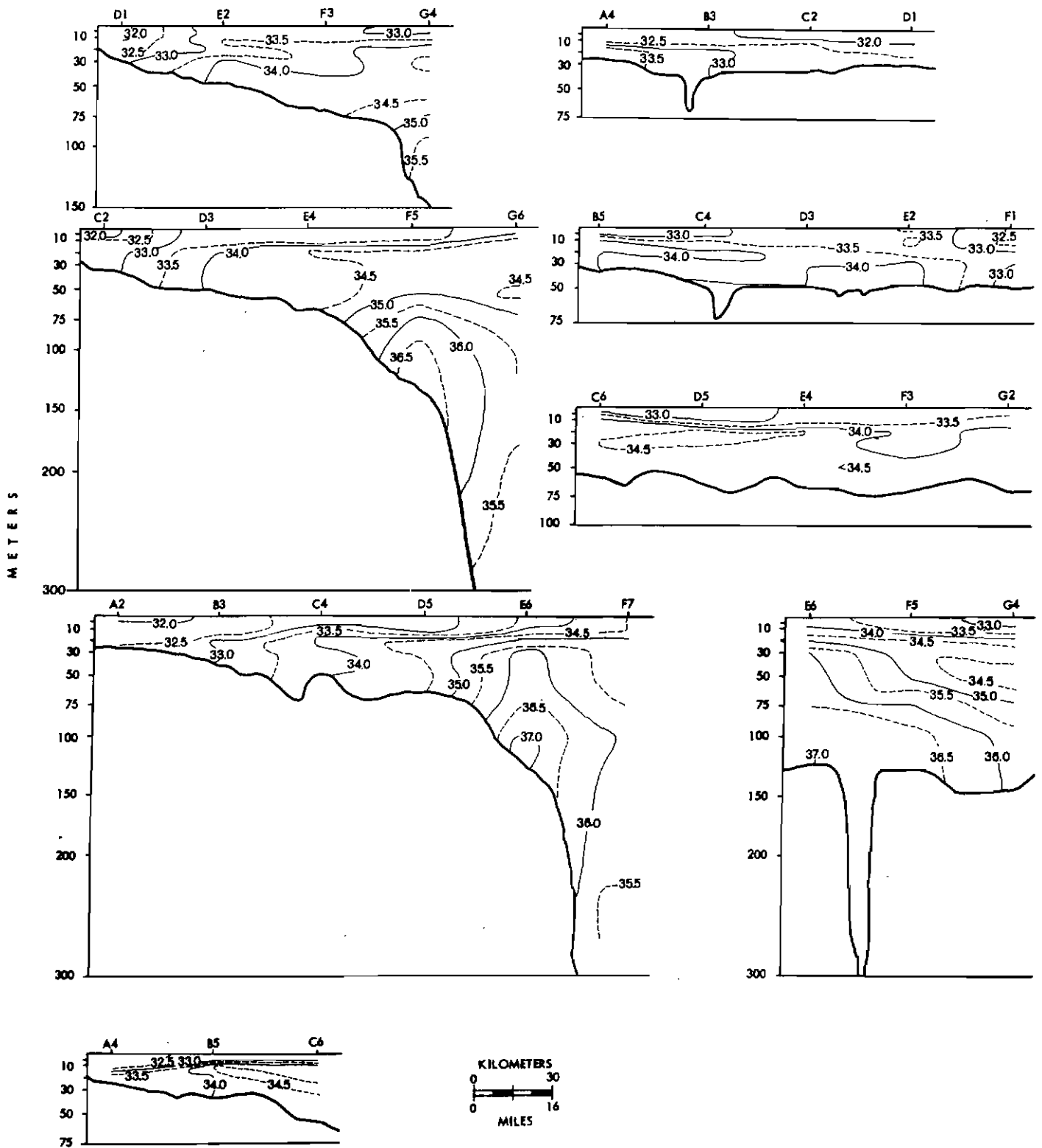
Figure 55. Vertical profiles of salinity August 1975.
