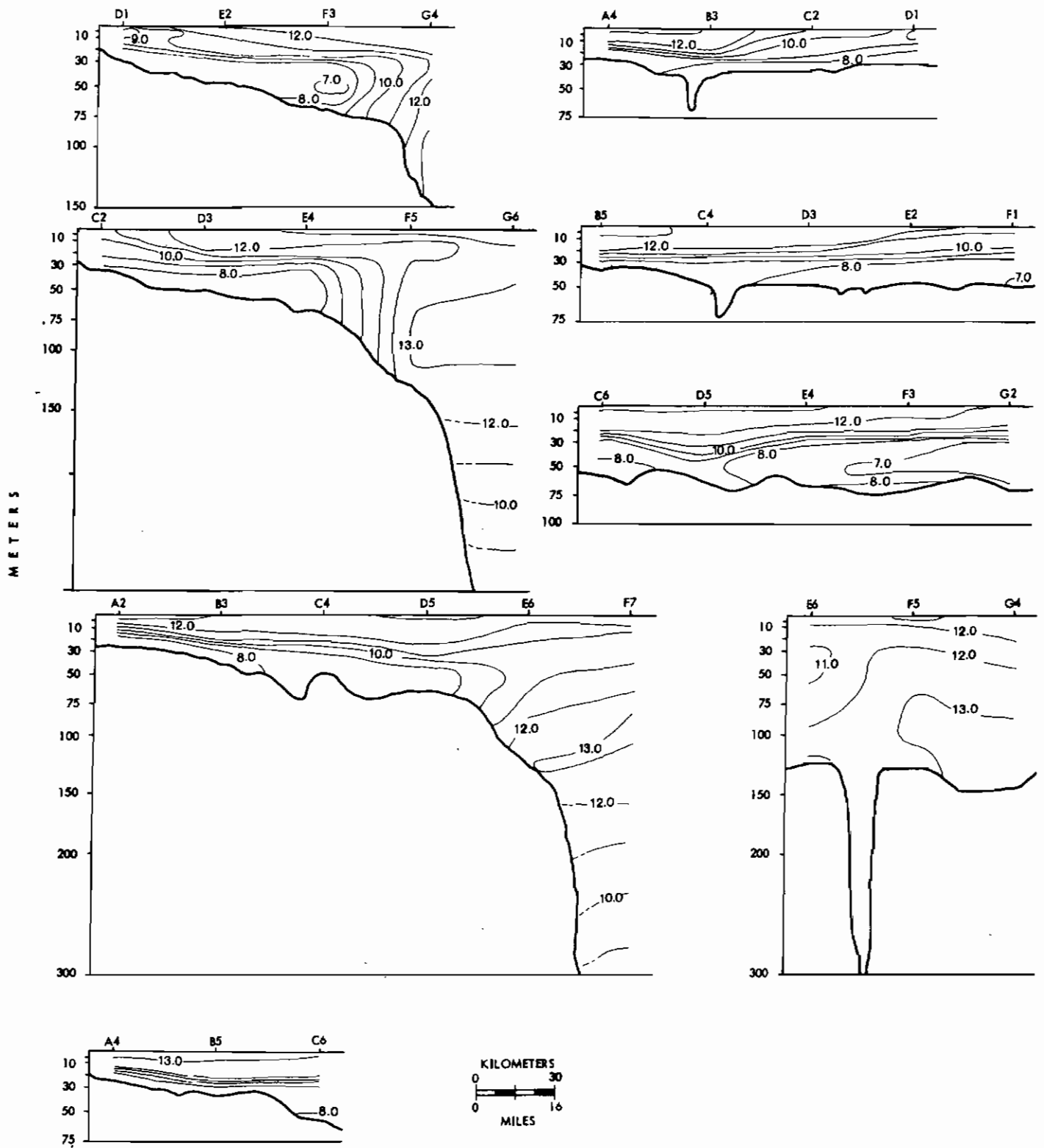
Figure 29. Vertical profiles of water temperature May 1976.
