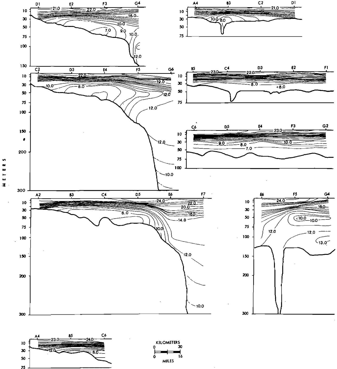
Figure 25. Vertical profiles of water temperature August 1975.
