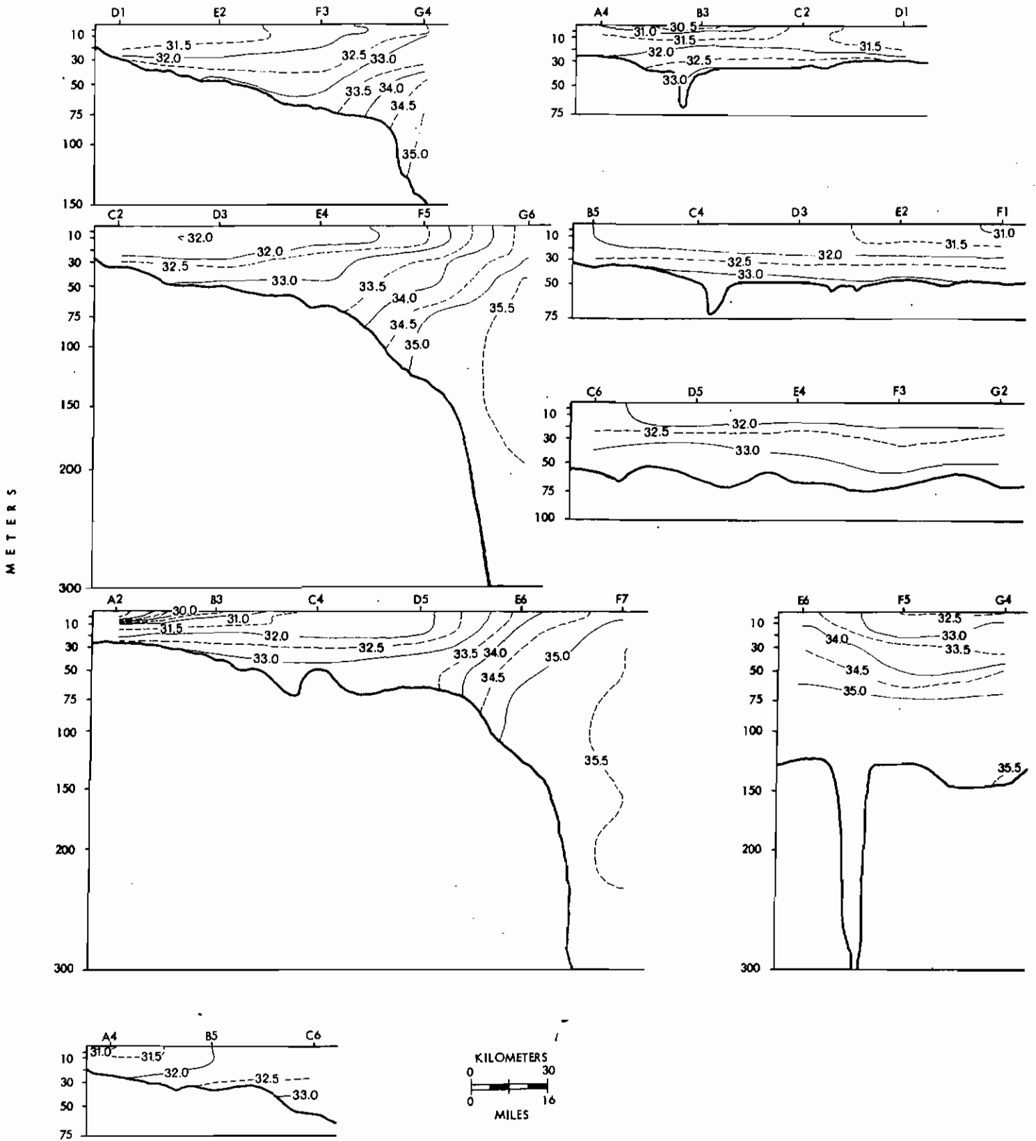
Figure 61. Vertical profiles of salinity June 1976.
