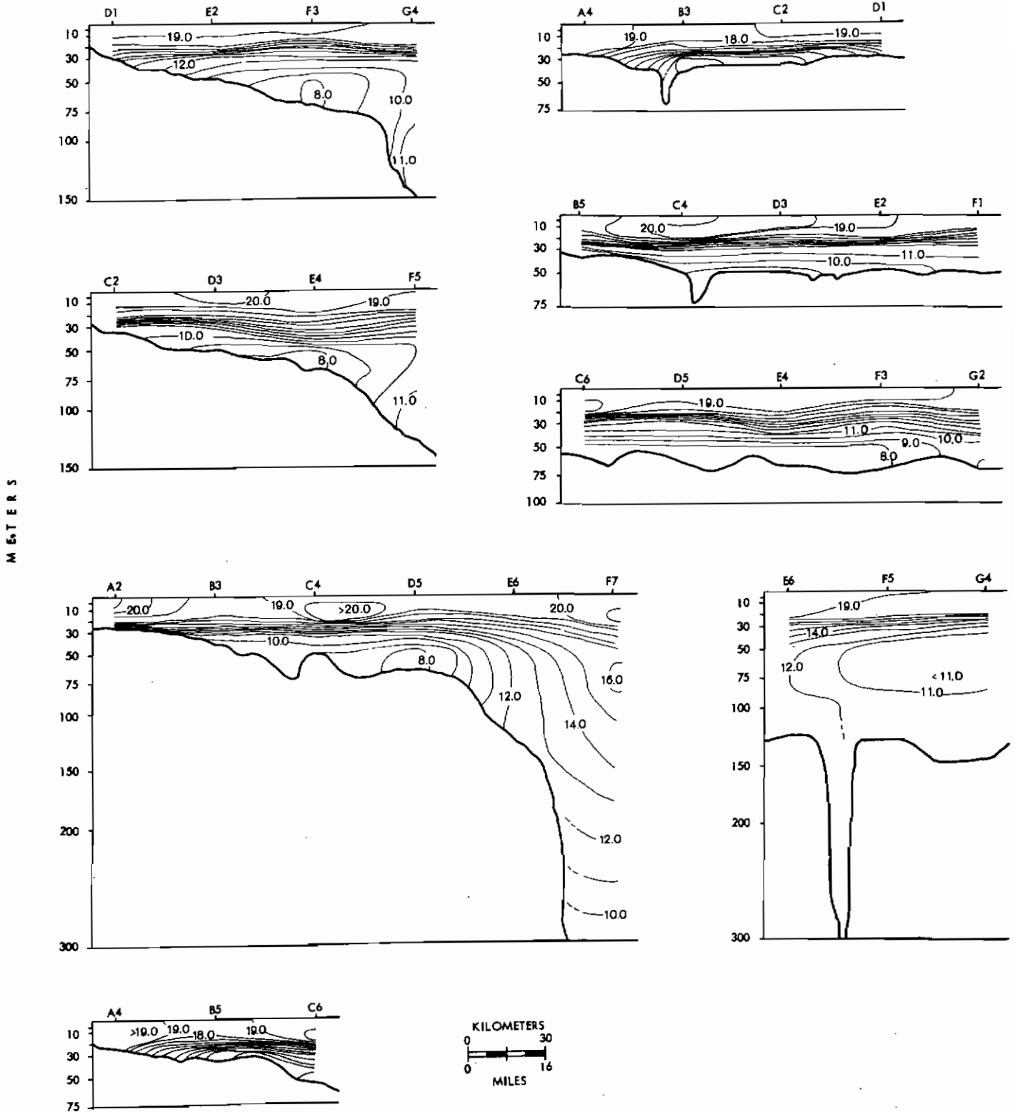
Figure 27. Vertical profiles of water temperature September 1975.
