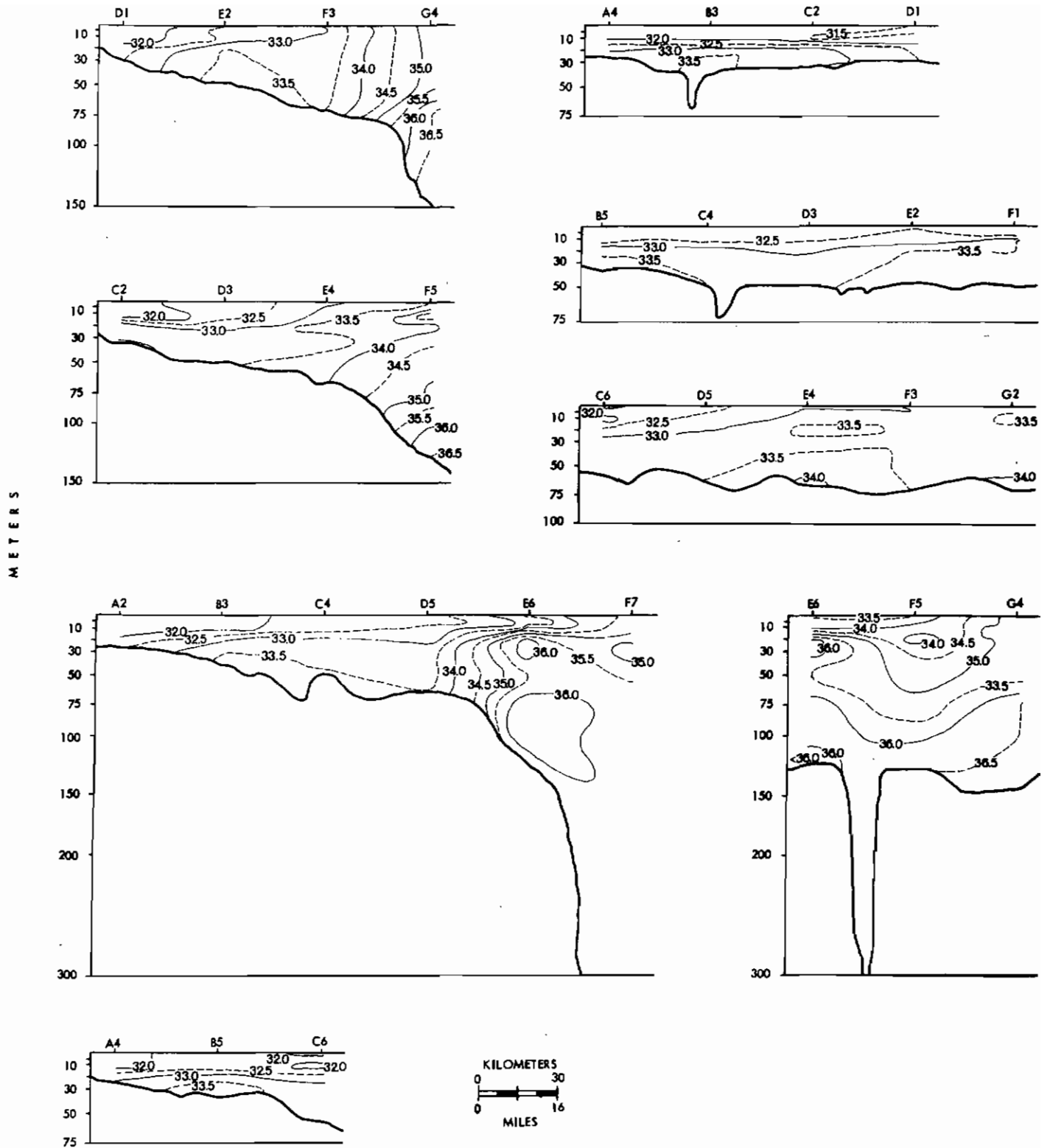
Figure 51. Vertical profiles of salinity June 1975.
