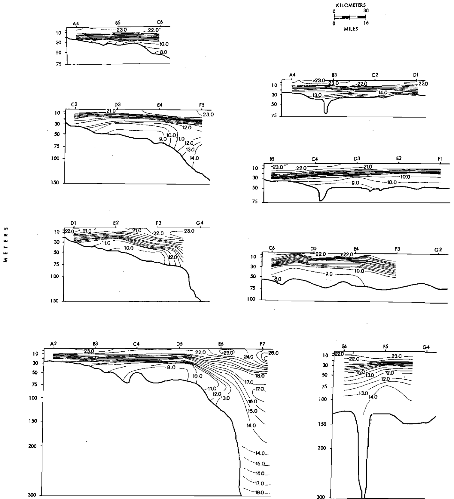
Figure 5. Vertical profiles of water temperature August 1974.
