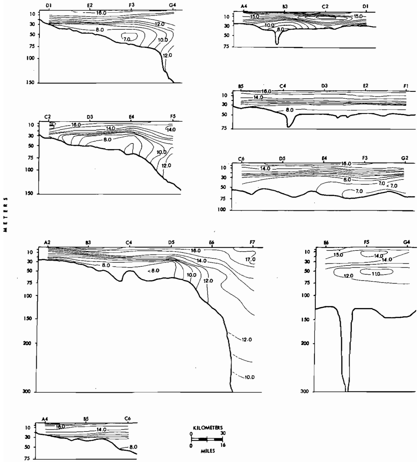
Figure 31. Vertical profiles of water temperature June 1976.
