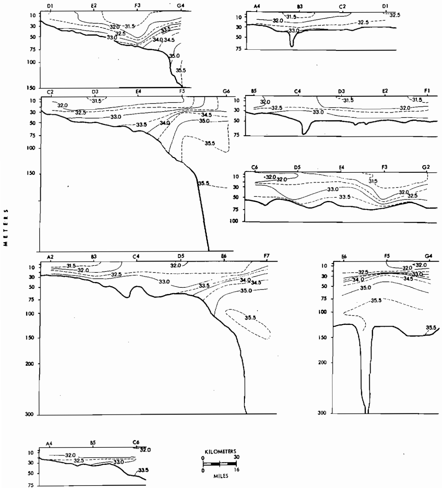
Figure 59. Vertical profiles of salinity May 1976.
