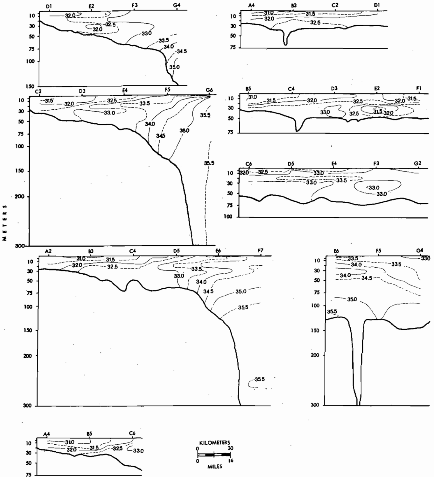
Figure 53. Vertical profiles of salinity July 1975.
