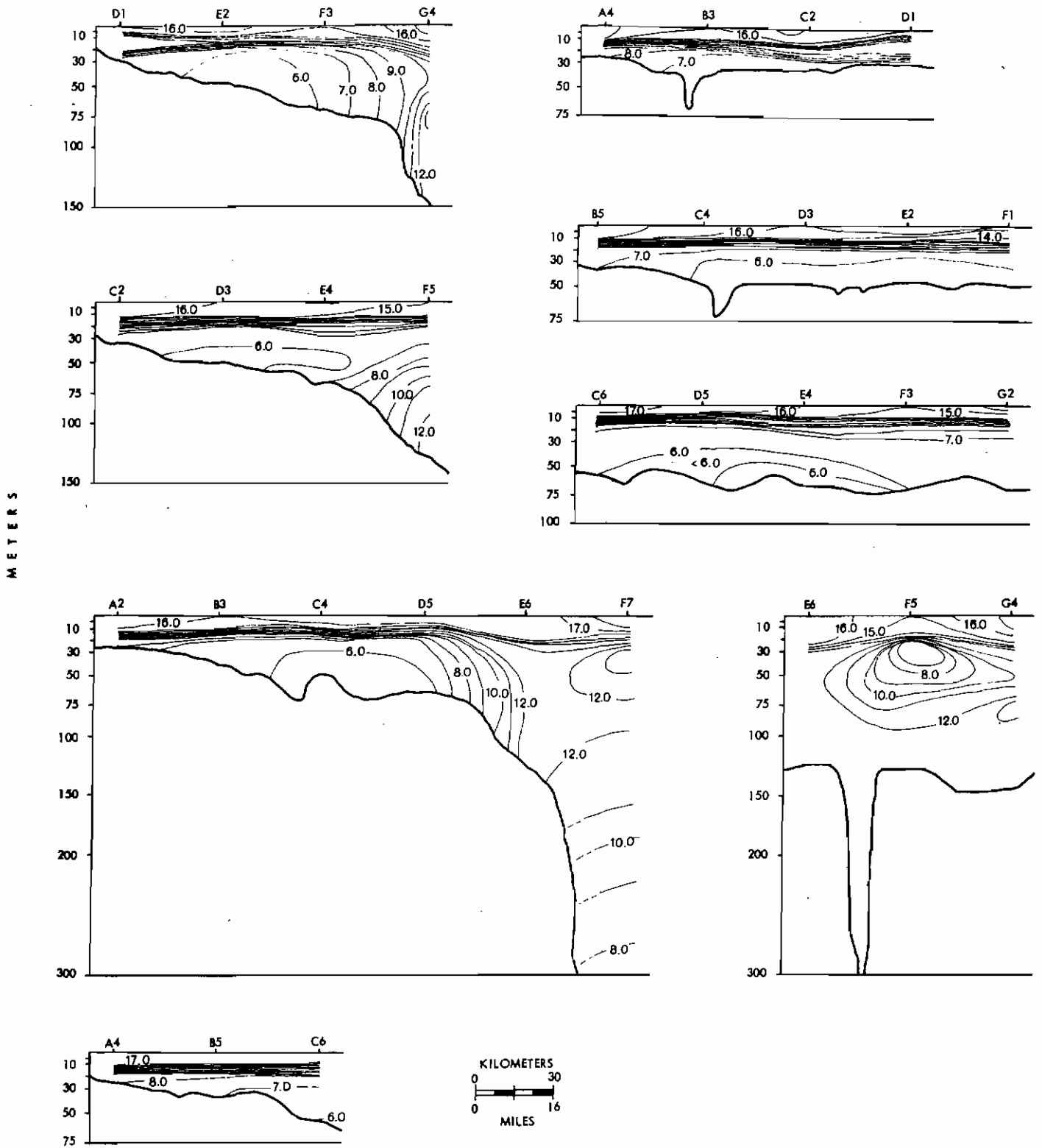
Figure 21. Vertical profiles of water temperature June 1975.
