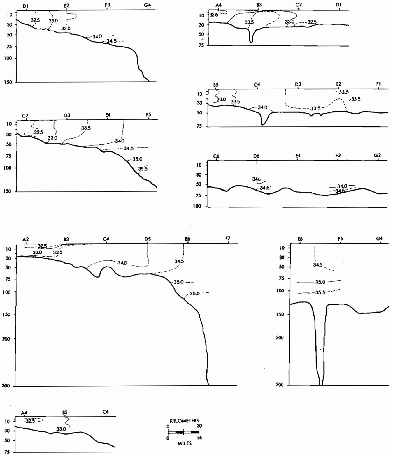
Figure 41. Vertical profiles of salinity November 1974.
