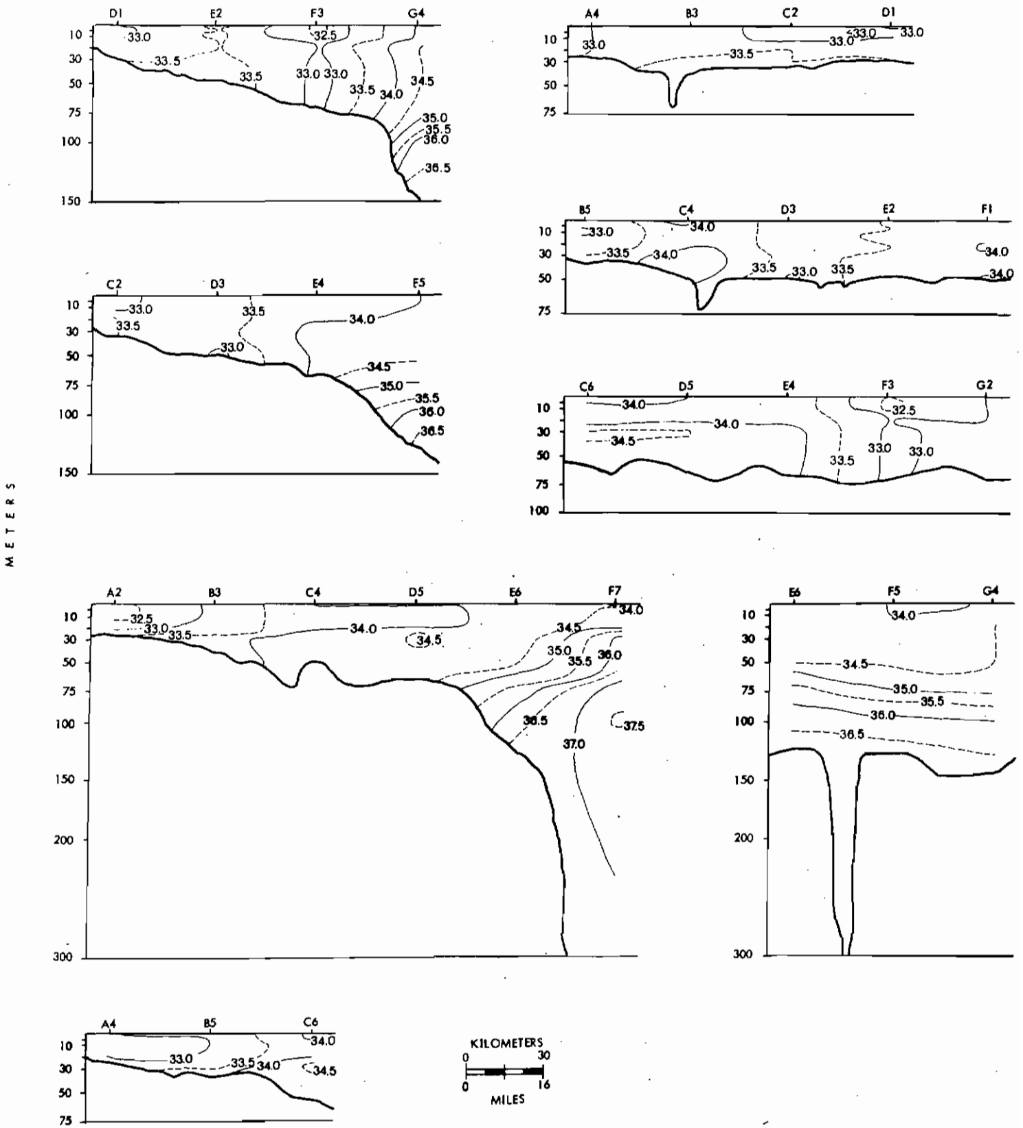
Figure 57. Vertical profiles of salinity September 1975.
