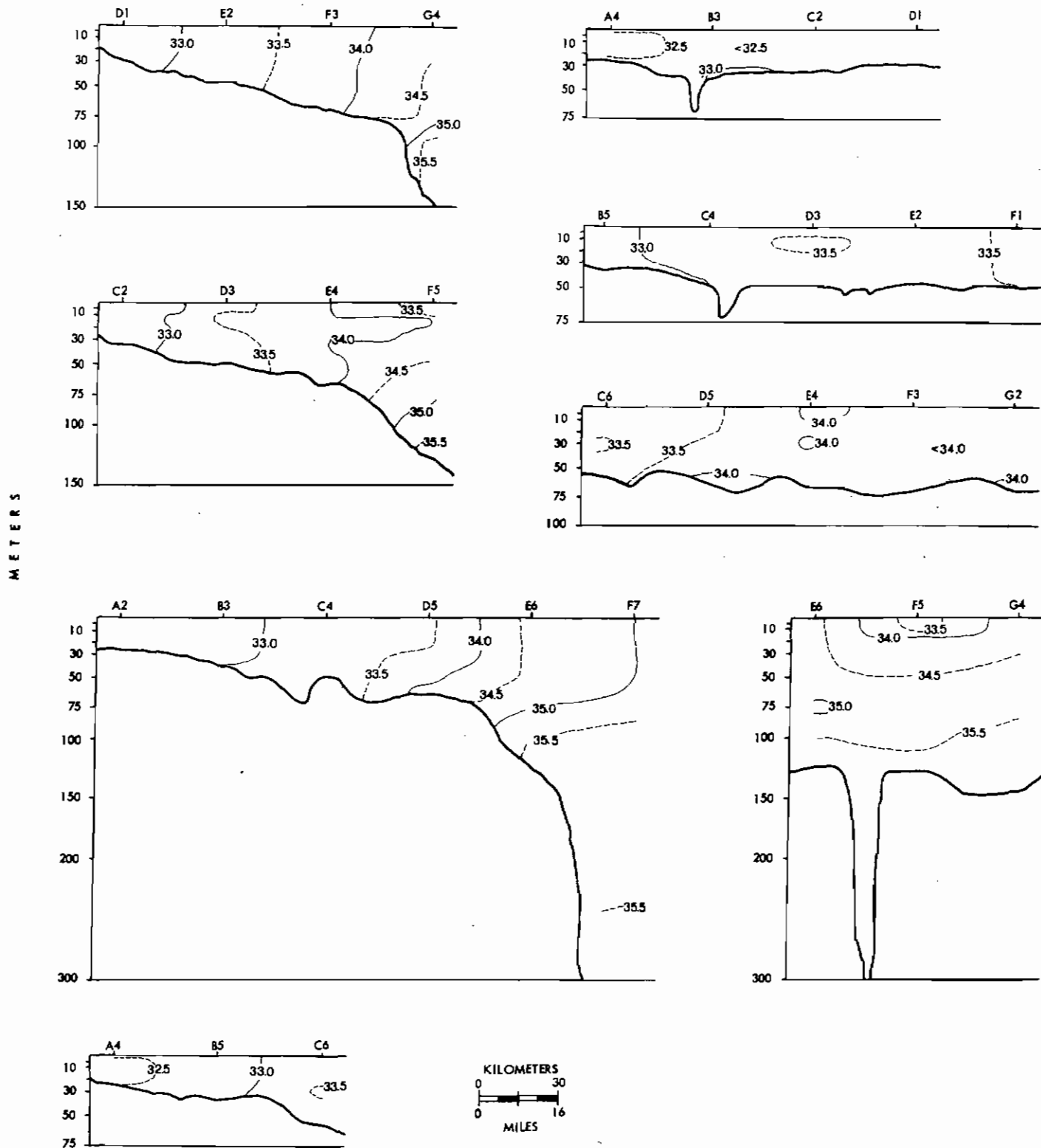
Figure 39. Vertical profiles of salinity October 1974.
