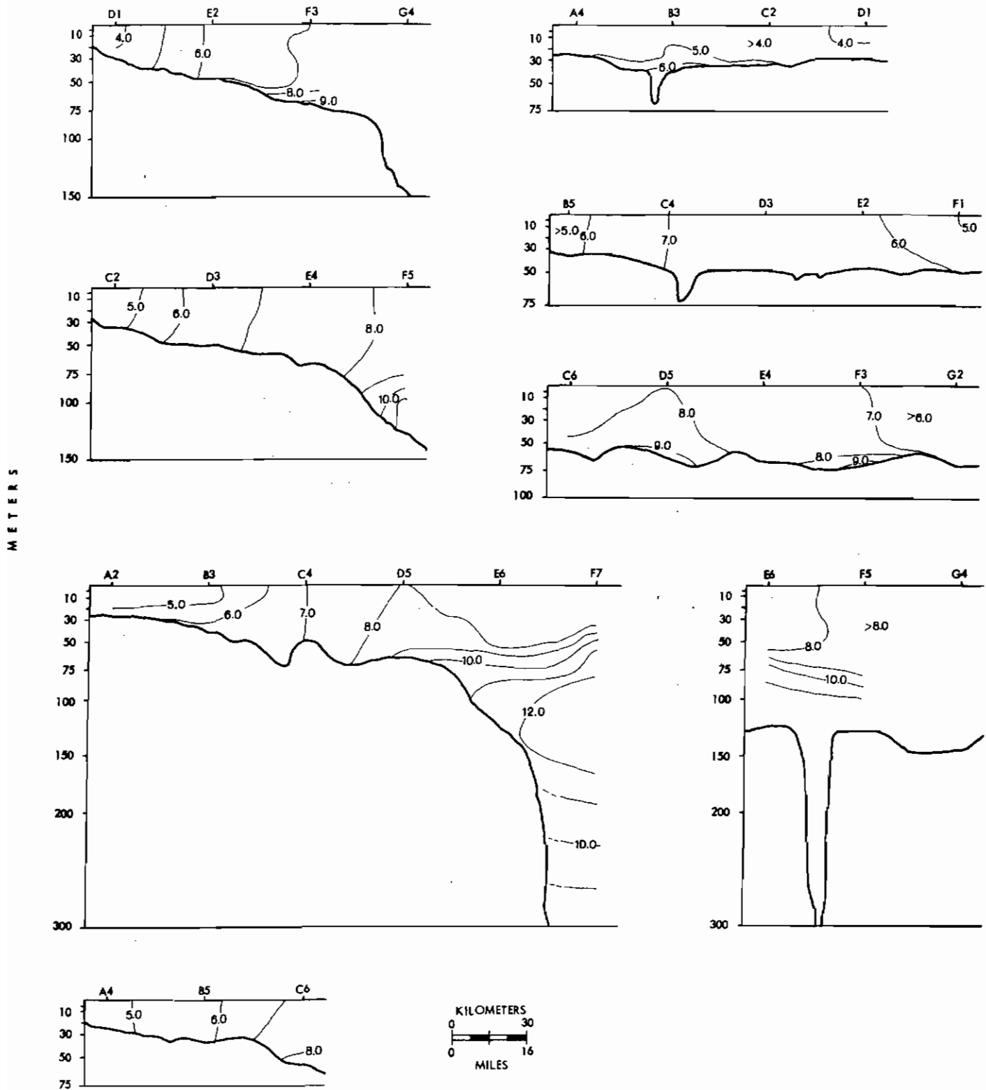
Figure 15. Vertical profiles of water temperature March 1975.
