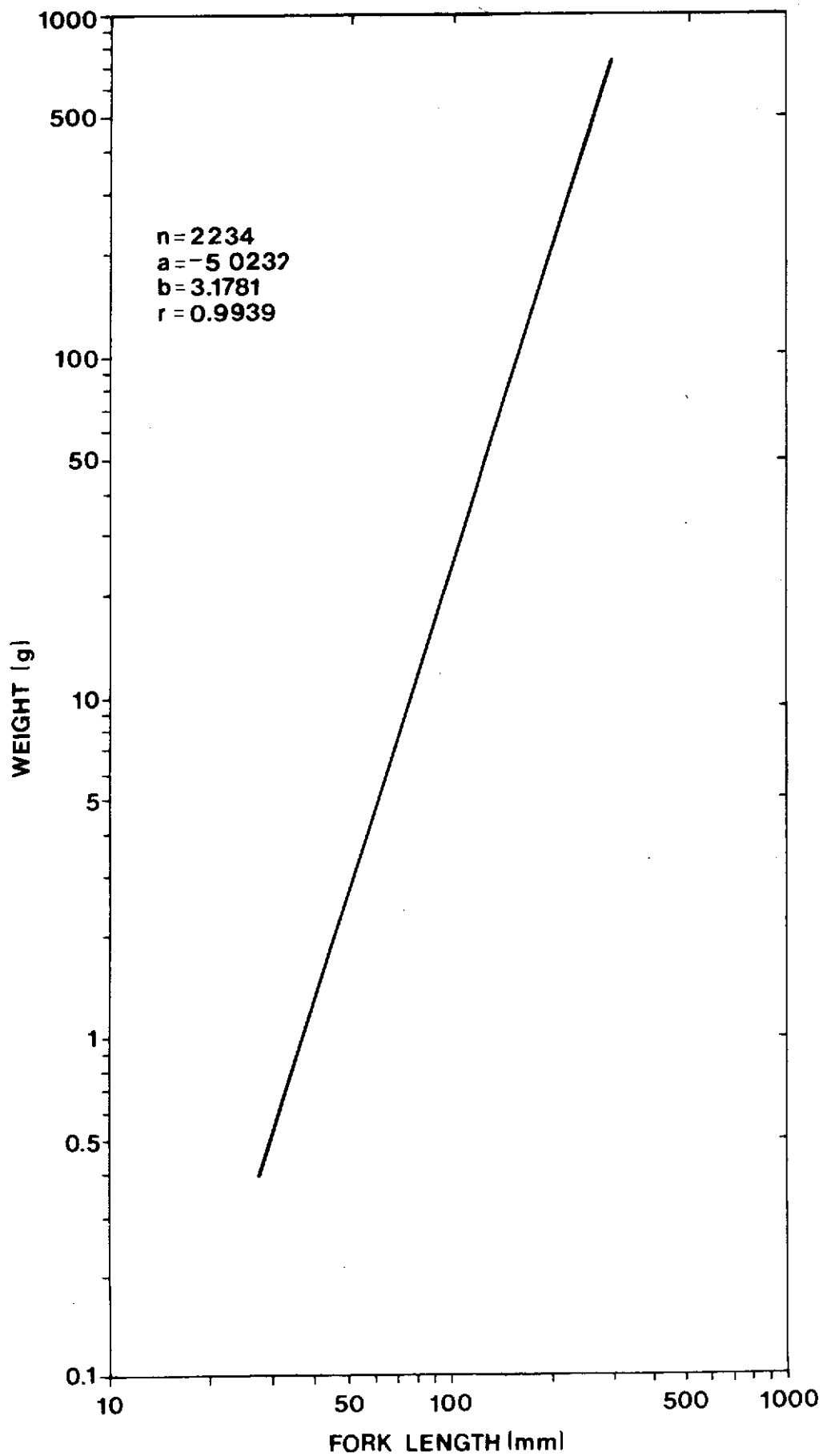
Figure 7. Length-weight relationship of scup, Stenotomus chrysops , collected in the New York Bight, June 1974 to June 1975.
