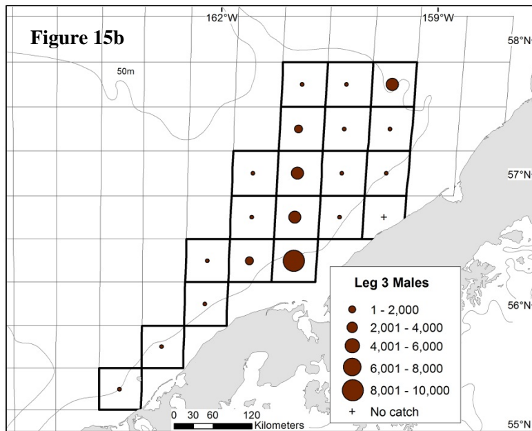
Figure 15. Total density (number \text{nmi}^{-2} ) of male red king crab ( Paralithodes camtschaticus ) at each station sampled during (a) Leg 1 (4 - 22 June 2012) and (b) Leg 3 (29 July to 2 August) in the Bristol Bay District.
