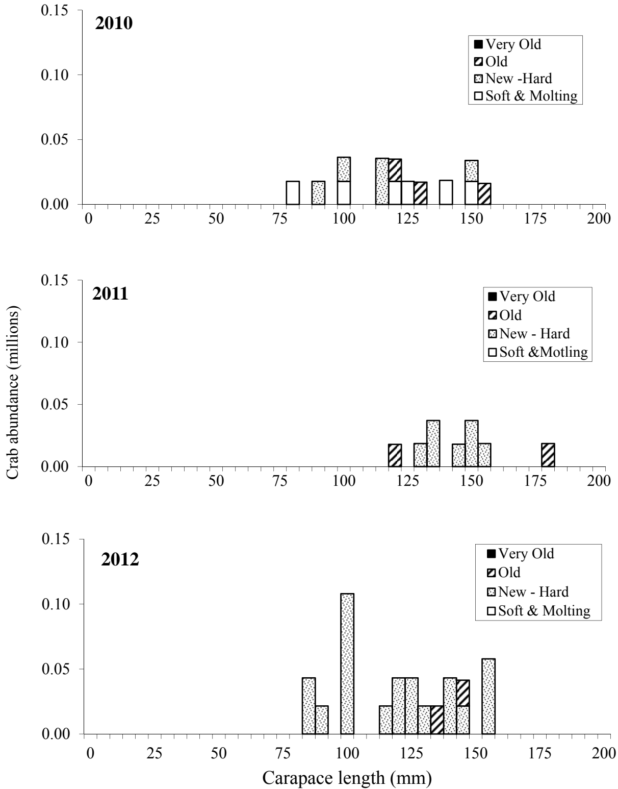
Figure 28. Size-frequency by shell condition of Pribilof District male blue king crab ( Paralithodes platypus ) by 5 mm length classes, 2010-2012.
