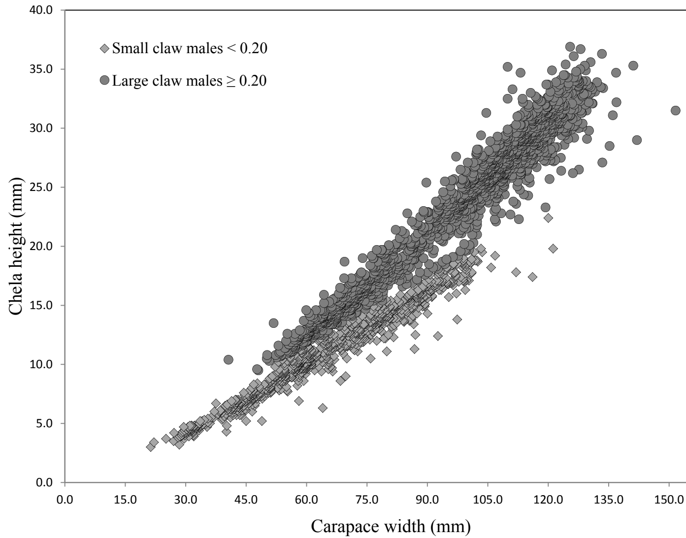
Figure 49. Male snow crab ( Chionoecetes opilio ) chela height versus carapace width measurements collected during the 2009 and 2011 National Marine Fisheries Service eastern Bering Sea bottom trawl surveys.
