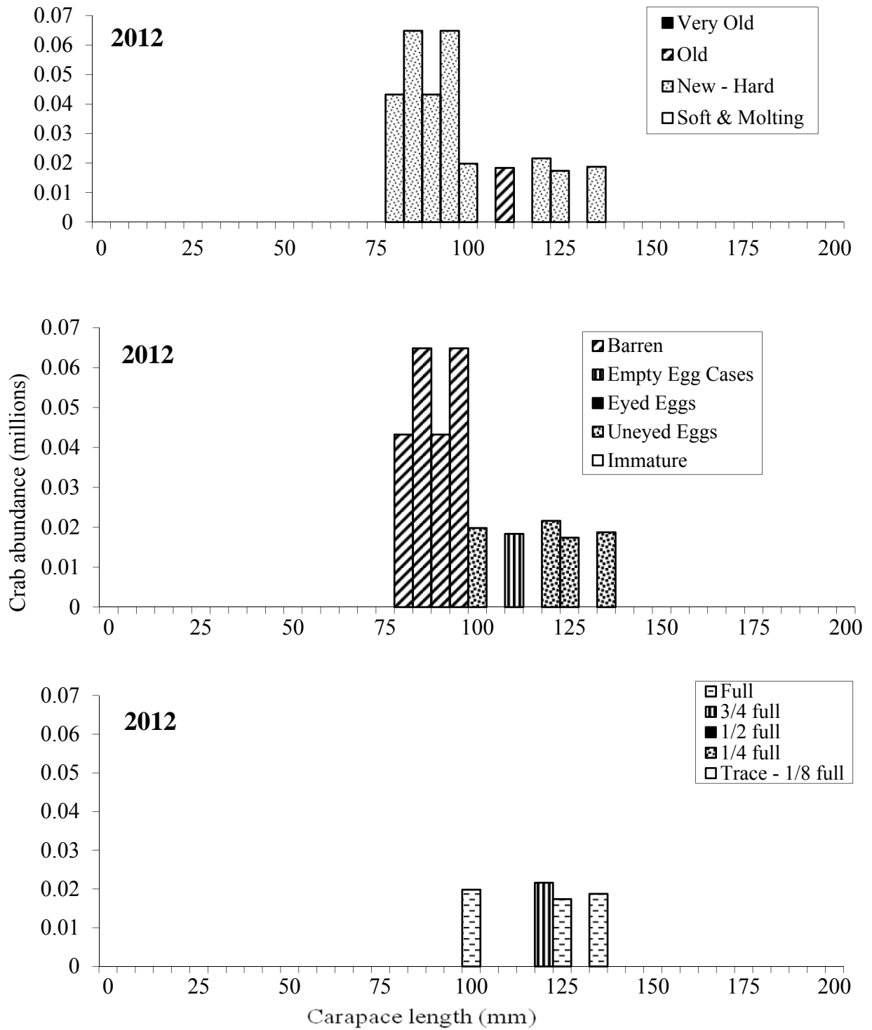
Figure 30. Size-frequency by shell condition, egg condition, and clutch fullness of Pribilof District female blue king crab ( Paralithodes platypus ) by 5 mm length classes in 2012.
