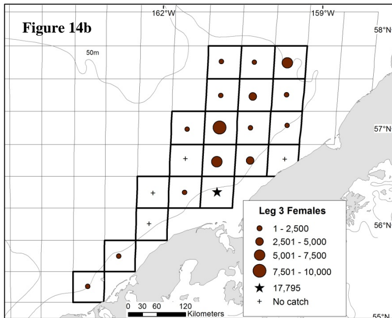
Figure 14. Total density (number \text{nmi}^{-2} ) of female red king crab ( Paralithodes camtschaticus ) at each station sampled during (a) Leg 1 (4 - 22 June 2012) and (b) Leg 3 (29 July to 2 August) in the Bristol Bay District.
