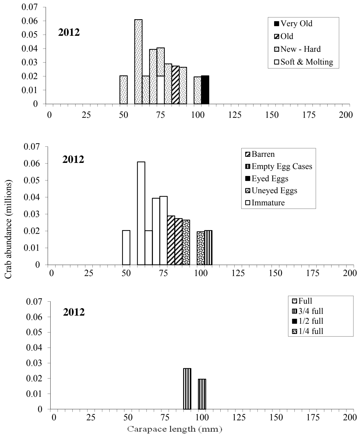
Figure 36. Size-frequency by shell condition, egg condition, and clutch size of St. Matthew Island Section female blue king crab ( Paralithodes platypus ) by 5 mm length classes in 2012.
