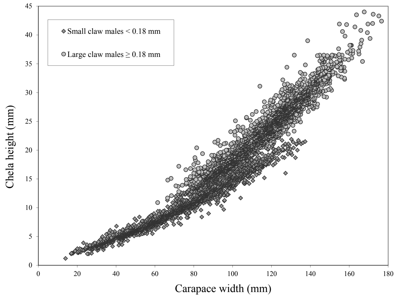
Figure 40. Male Tanner crab ( Chionoecetes bairdi ) chela height versus carapace width measurements collected on the 2008, 2010, and 2012 National Marine Fisheries Service eastern Bering Sea bottom trawl surveys.
