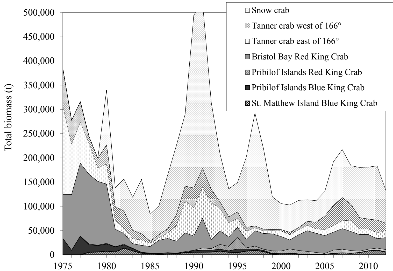
Figure 7. Historical mature male biomass for six commercial species caught on National Marine Fisheries Service eastern Bering Sea bottom trawl surveys.
