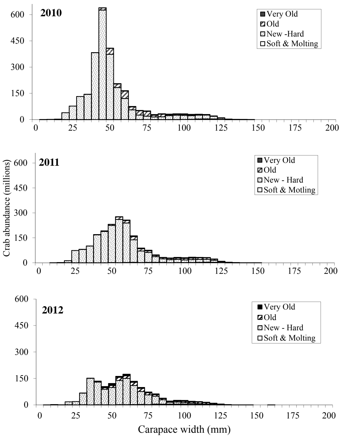
Figure 50. Size-frequency by shell condition of male snow crab ( Chionoecetes opilio ) by 5 mm width classes of all districts combined, 2010-2012.
