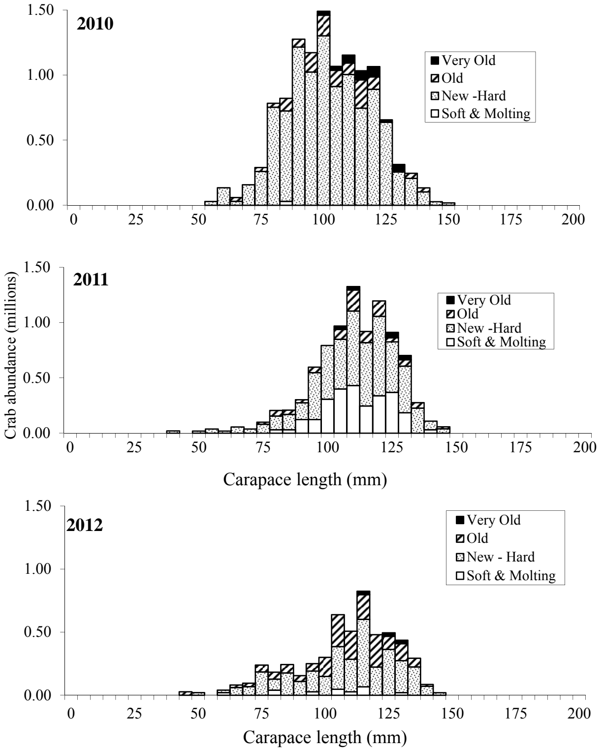
Figure 34. Size-frequency by shell condition of St. Matthew Island Section male blue king crab ( Paralithodes platypus ) by 5 mm length classes, 2010-2012.
