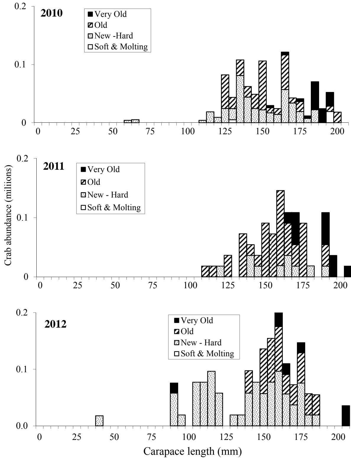
Figure 22. Size-frequency by shell condition of Pribilof District male red king crab ( Paralithodes camtschaticus ) by 5 mm length classes, 2010-2012.
