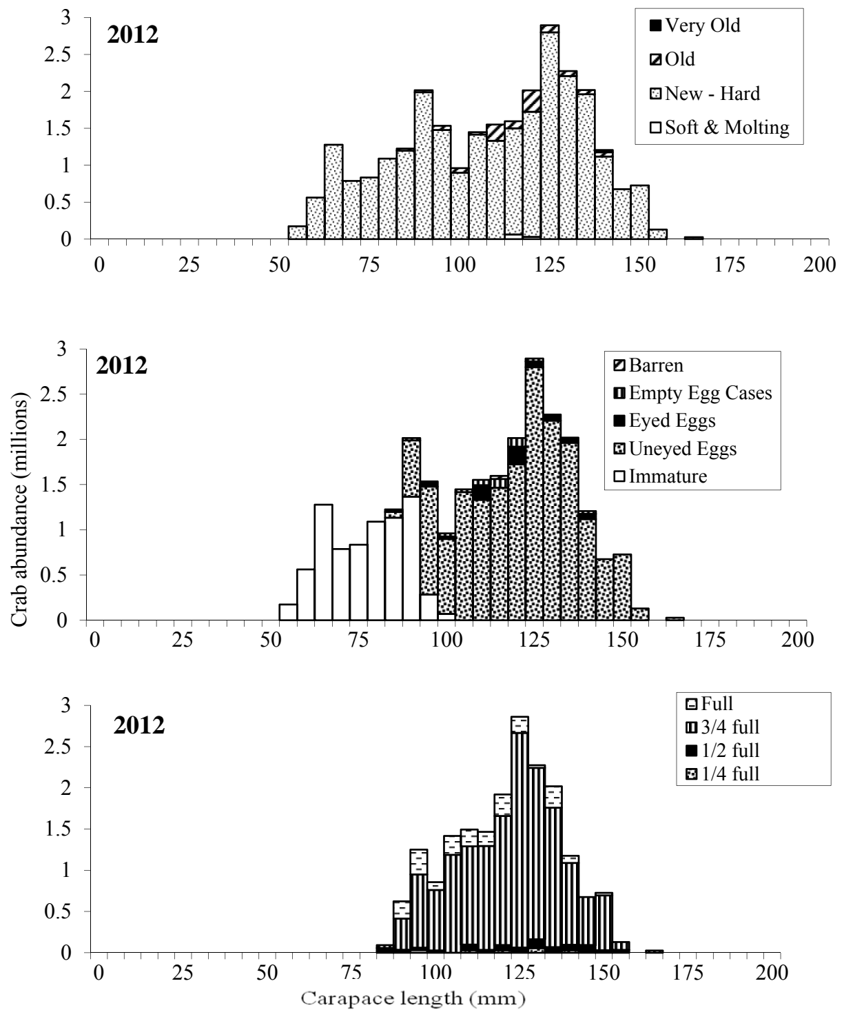
Figure 16. Size-frequency by shell condition, egg condition, and clutch fullness of Bristol Bay District female red king crab ( Paralithodes camtschaticus ) by 5 mm length classes in 2012.
