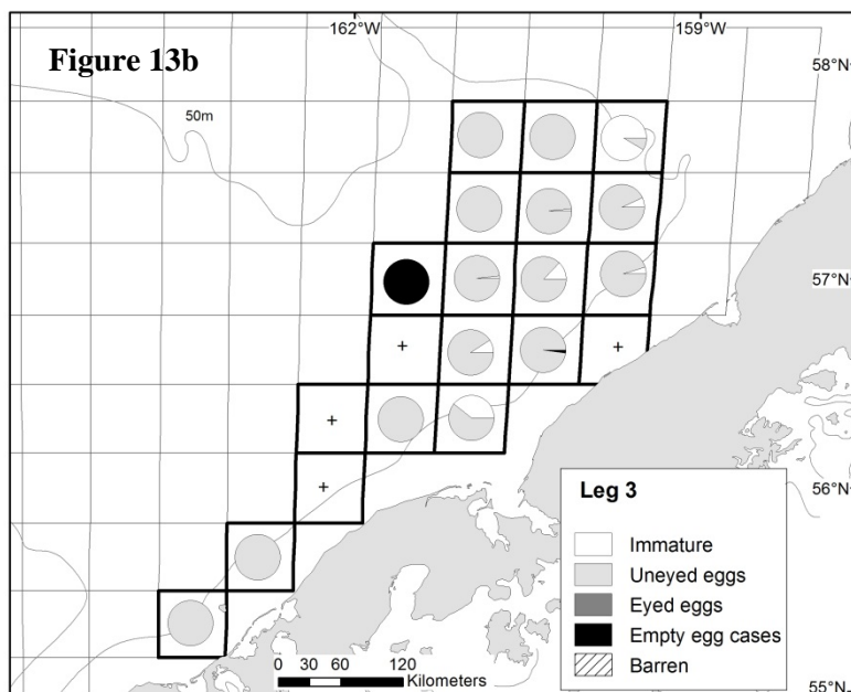
Figure 13. Distribution and egg condition of female red king crab ( Paralithodes camtschaticus ) caught (a) Leg 1 (4 - 22 June 2012) and (b) Leg 3 (29 July to 2 August) in the Bristol Bay District. Outline depicts the 20 stations resampled in late July on Leg 3.
