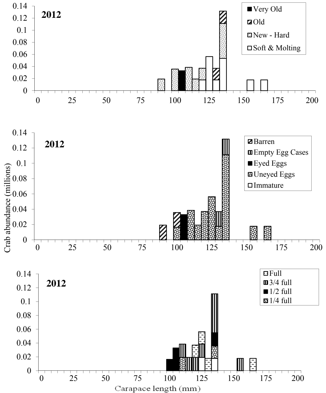
Figure 24. Size-frequency by shell condition, egg condition, and clutch fullness of Pribilof District female red king crab ( Paralithodes camtschaticus ) by 5 mm length classes in 2012.
