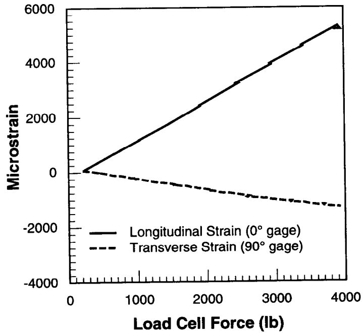
Figure 9. Blade skin strains at station 134 for Phase 1 loading.
