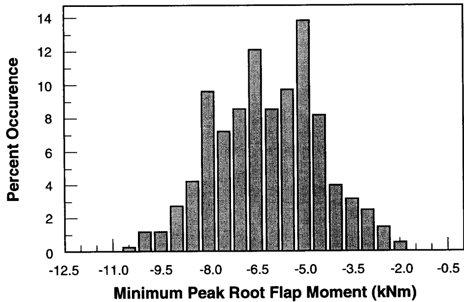
Figure 2. Root flap bending moments, measured maximum peaks.
