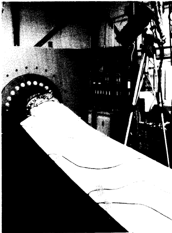
Figure 35. The shearography system viewing the root section of the blade.
