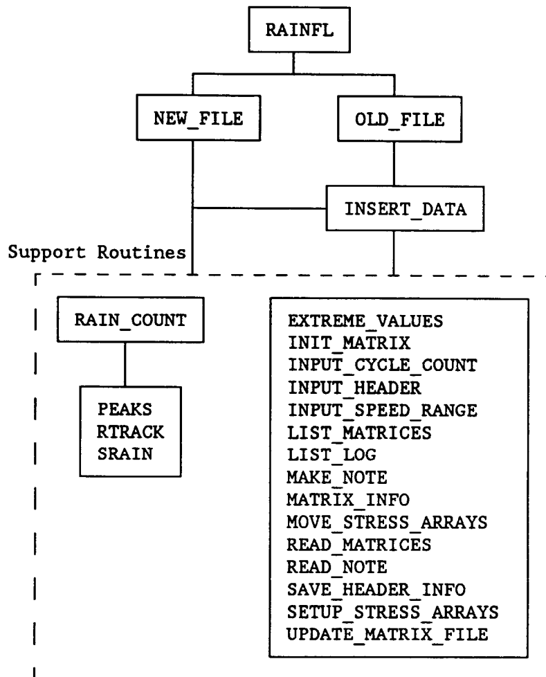
Hierarchy of Rainflow Subroutines
