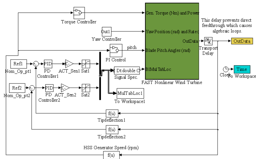
Figure 4. Dynamic simulation environment: FAST with augmented pitch and microtab control systems
