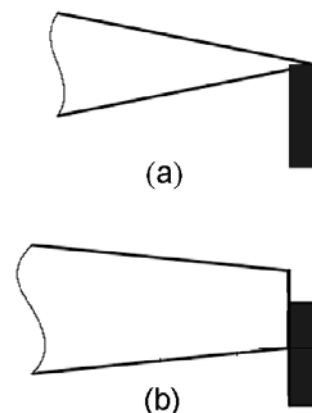
Fig. 3-18 Geometry of (a) Gurney flap and (b) MiTE attached to a sharp and blunt trailing edge airfoil. (Source: Lee and Kroo 63 )
