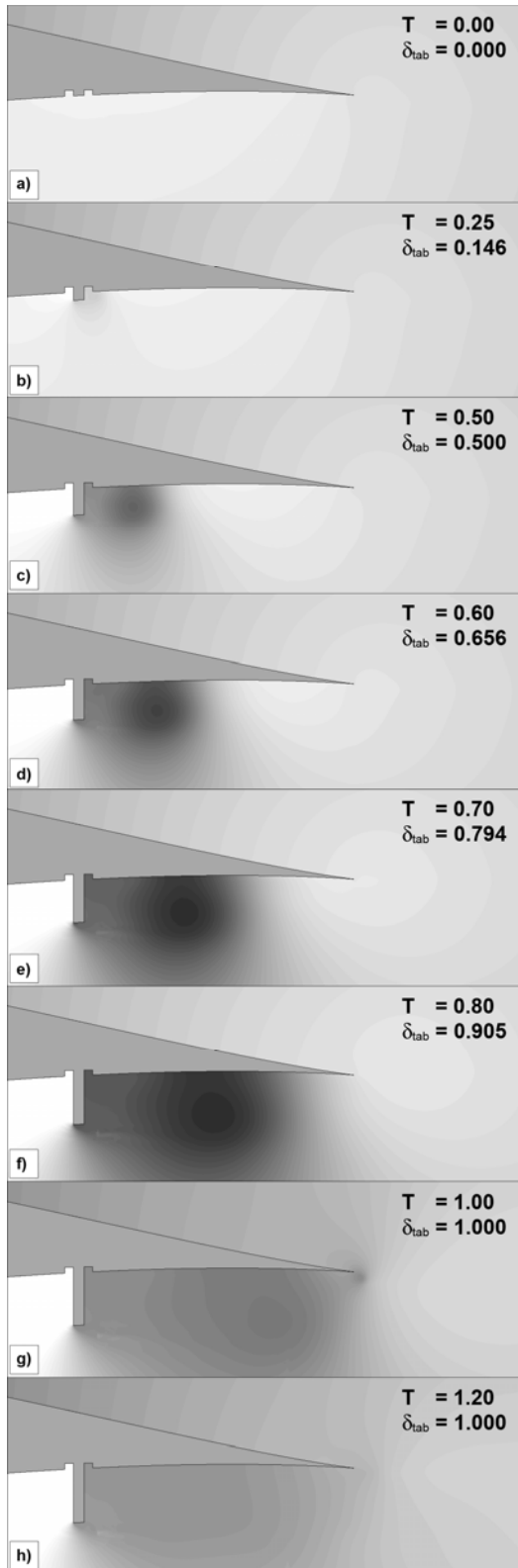
Fig. 3-14 C_p contours in tab region during deployment, ( T_{deployment} = 1 ). Darker regions indicate lower pressure. (Source: Chow and van Dam 57 )
