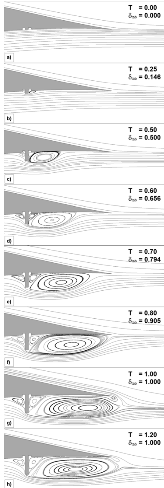
Fig. 3-15 Instantaneous streamlines in trailing-edge region of S809 airfoil during tab deployment, ( T_{deployment} = 1 ). (Source: Chow and van Dam 57 )
