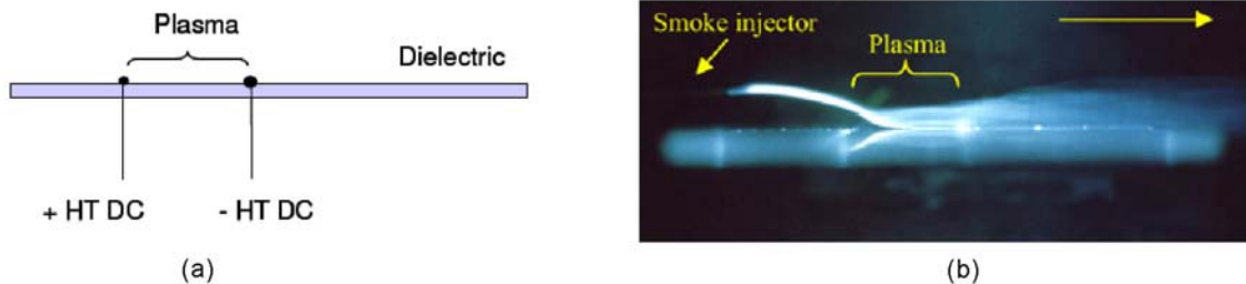
Fig. 3-30 a) Schematic side view of the DC corona discharge actuator, b) 2D visualization of manipulated airflow along a flat plate. (Source: Moreau et al. 93 )
