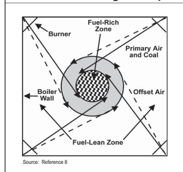
Exhibit 3-34 Concentric Firing Concept
