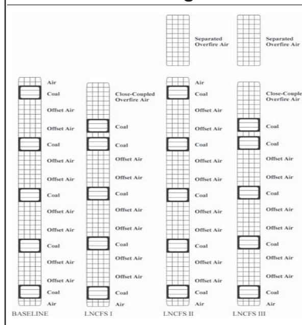
Exhibit 3-33 LNCFS™ Configurations
