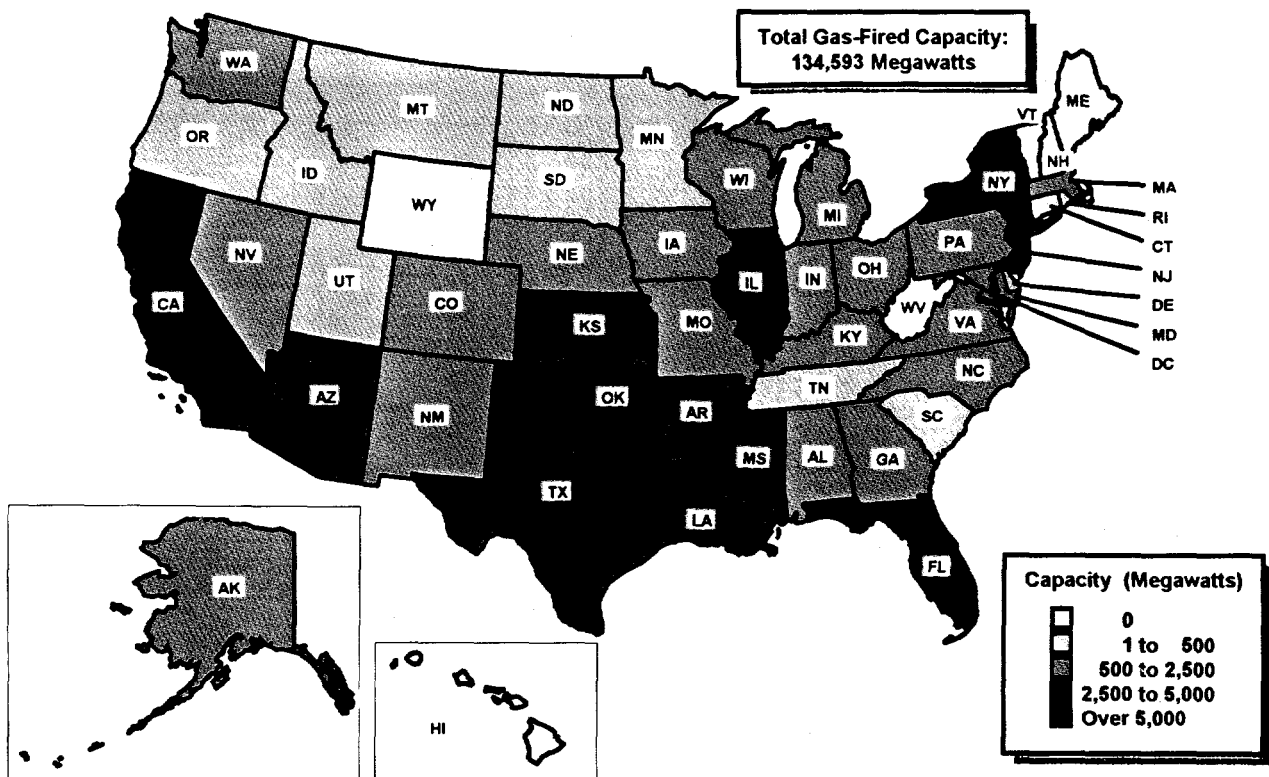
Figure 5. Gas-Fired Capacity at U.S. Electric Utilities by State, as of January 1, 1997
