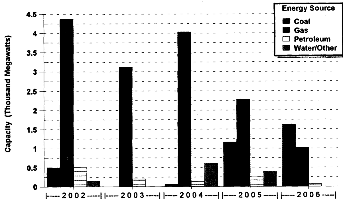
Figure 14. Planned Capacity Additions at U.S. Electric Utilities by Energy Source, 2002 Through 2006
