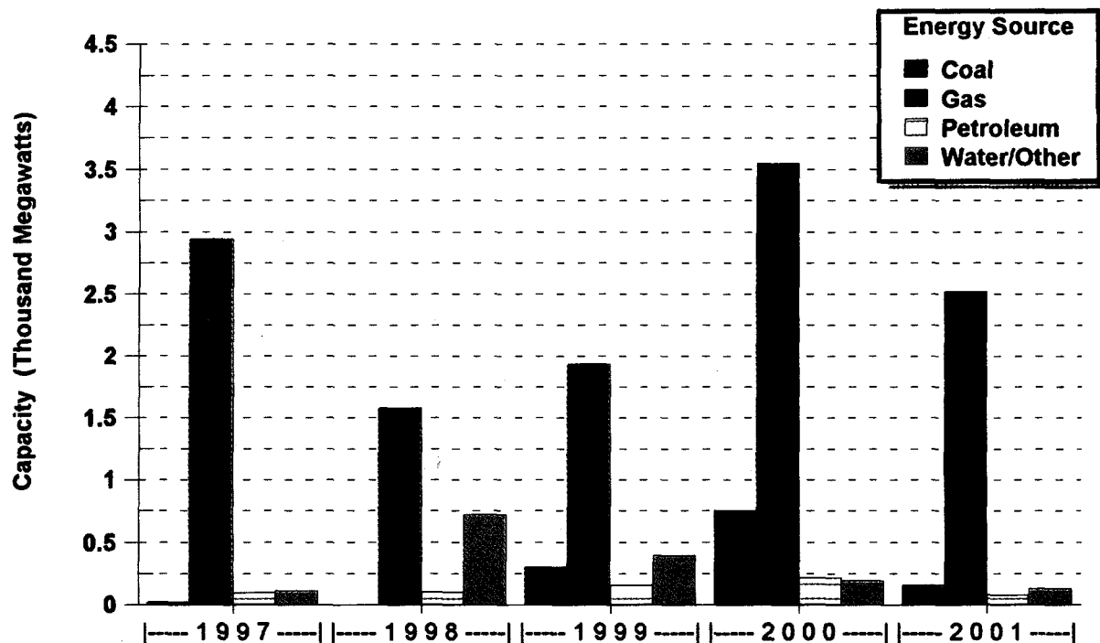
Figure 13. Planned Capacity Additions at U.S. Electric Utilities by Energy Source, 1997 Through 2001
