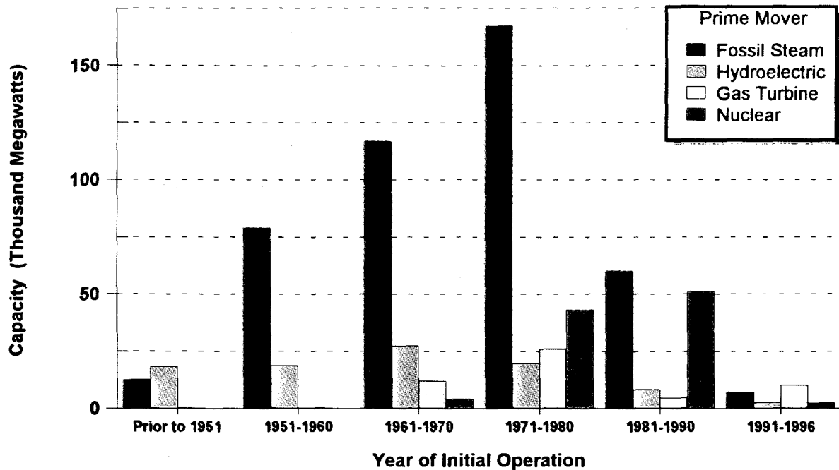
Figure 9. Existing Capacity at U.S. Electric Utilities by Prime Mover and Initial Year of Commercial Operation, as of January 1, 1997
