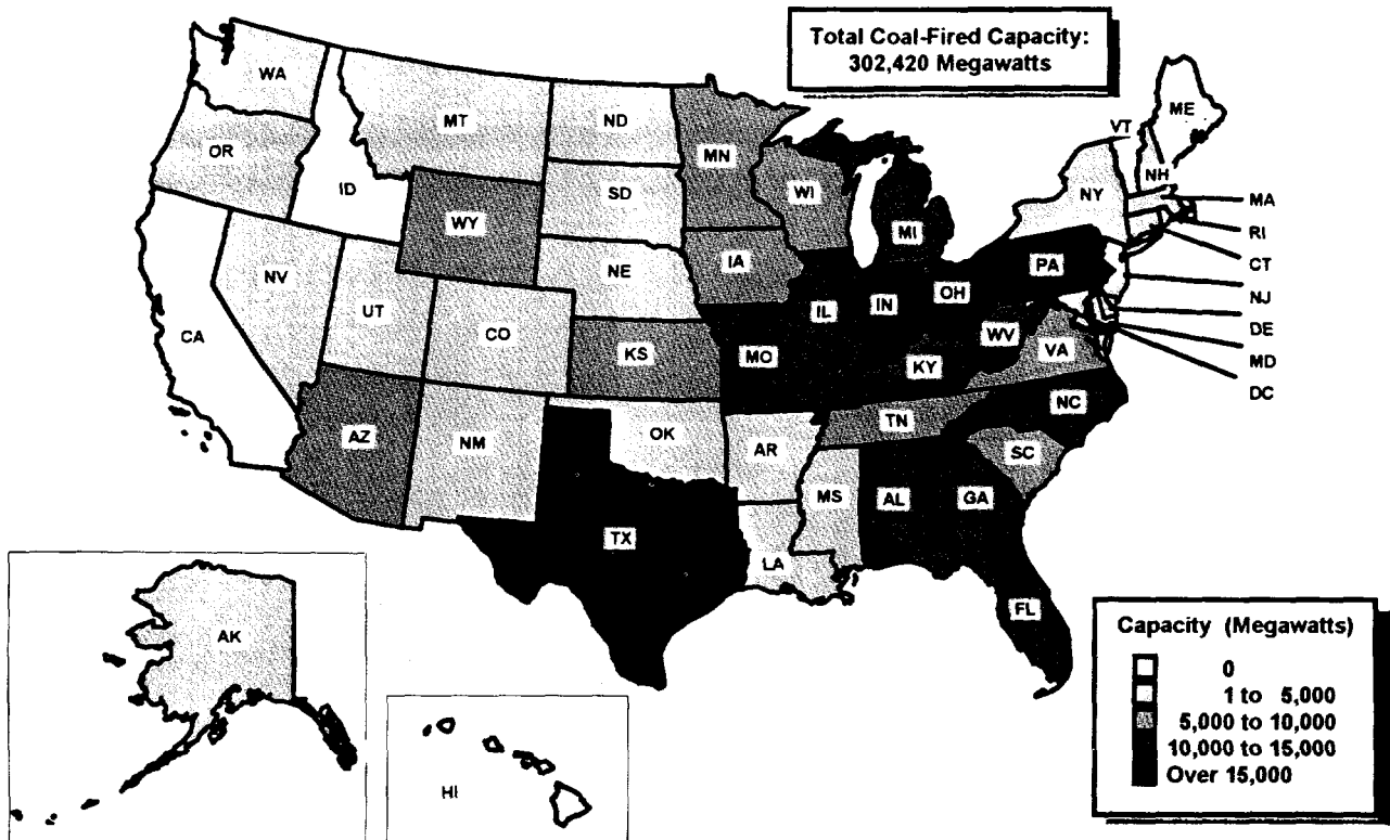
Figure 3. Coal-Fired Capacity at U.S. Electric Utilities by State, as of January 1, 1997
