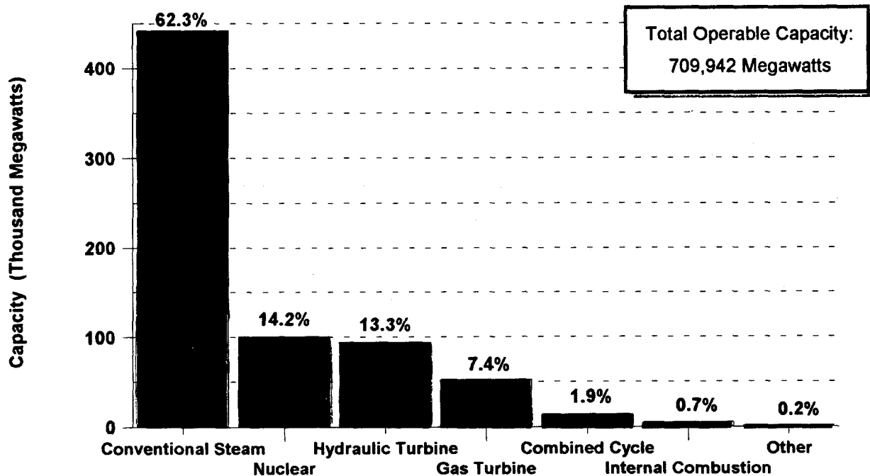
Figure 2. Share of Capacity at U.S. Electric Utilities by Prime Mover, as of January 1, 1997
