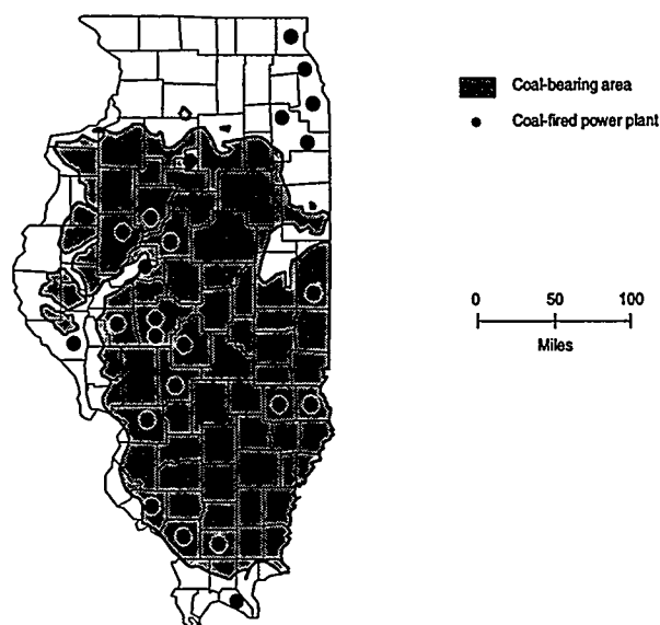
Figure 4. Coal-Bearing Areas of Illinois
