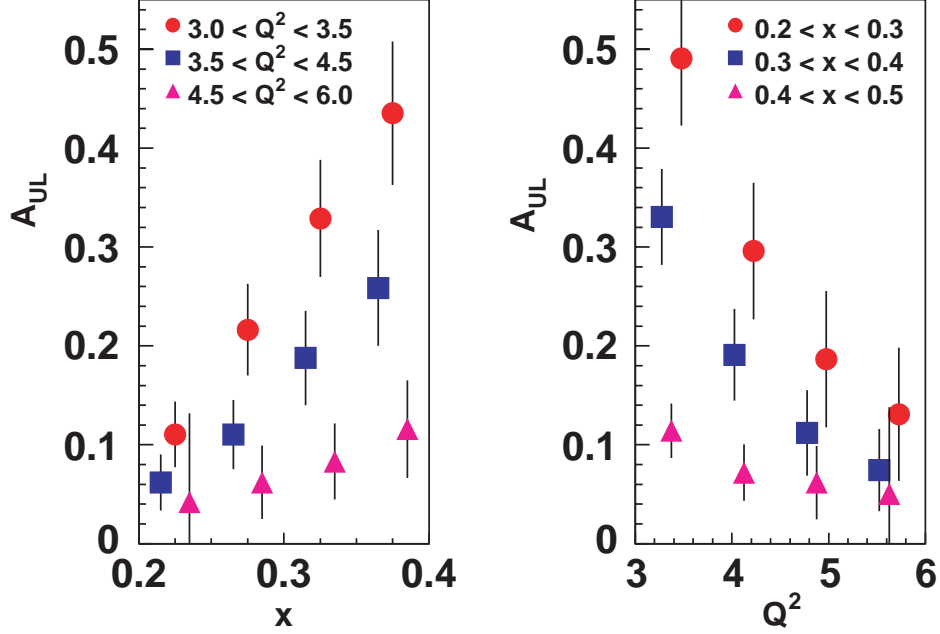
Figure 81: Projected data for longitudinal target asymmetry measured in CLAS ++ for a 2000 hrs run at a luminosity of 10^3 5\text{cm}^{-2}\text{sec}^{-1} . The t-dependences will be obtained simultaneously.
