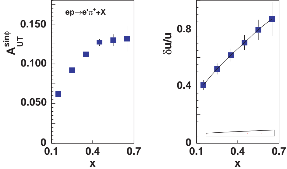
Figure 95: Projected transverse spin asymmetry ( A_{UT}^{\sin\phi} ) in single \pi^+ production with CLAS at 12 GeV (left plot) and expected precision of the extracted \delta u/u (right plot). The line is the Monte Carlo generated \delta u/u .
