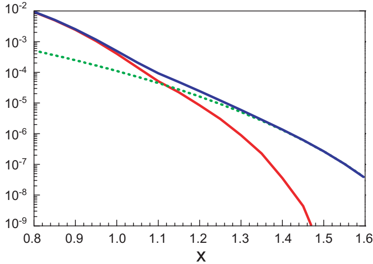
Figure 101: Distribution of super-fast quarks for deuteron assuming just two nucleons (red curve), or including a 5% contribution from a 6-quark bag (green dashed curve). The sum of the two contributions is shown as the blue curve. The expected uncertainties including a systematic uncertainty of 3-5% are smaller than the points shown. We expect that for x -values below 1.4 (black circles) the data should be in the DIS scaling regime.
