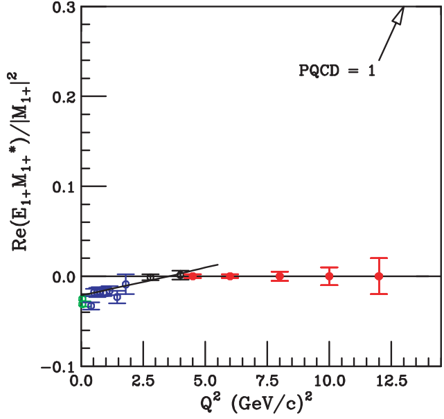
Figure 53: The E_{1+}/M_{1+} (or -G_E^*/G_M^* ) ratio for Delta excitation, including JLab data from Halls B (blue) and C (black) [Jo02, Fr98a], and projected Hall C 12 GeV upgrade data. The curve below 4 (\text{GeV}/c)^2 is the MAID dynamical model fit [Dr99]. In the pQCD limit G_M^*/G_D \rightarrow \text{const} and E_{1+}/M_{1+} \rightarrow 1 . The dashed curve is due to the soft Gaussian dependent part.
