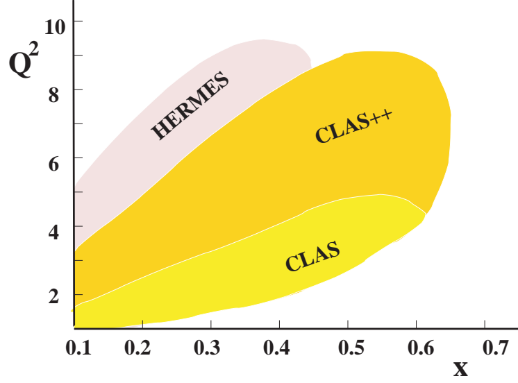
Figure 96: Kinematic coverage for single-spin asymmetry measurements at JLab at 12 GeV.
