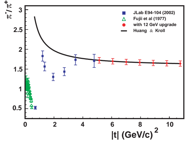
Figure 119: The charged pion photoproduction differential cross-section ratio at a C.M. angle of 90^\circ , as a function of |t| ( \text{GeV}/c ) ^2 from experiment E94-104 (blue) along with the projected measurements for JLab at 11 GeV (red). The solid curve is a prediction by Huang and Kroll [Hu00].
