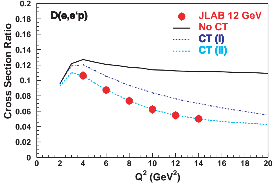
Figure 105: Ratio R = \sigma(p_m = 400 \text{ MeV}/c)/\sigma(p_m = 200 \text{ MeV}/c) for D(e,e'p) reaction. CT(I) and CT(II) corresponds to Color Transparency calculations with \Delta M^2 = 0.7 and 1.1 \text{ GeV}^2 respectively in the QDM Model [Fa88, Sape]
