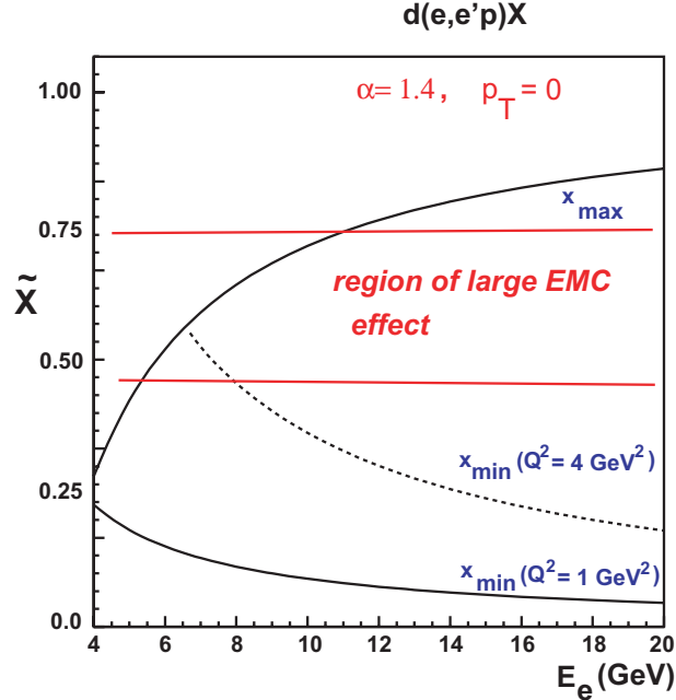
Figure 102: The scaling window for \alpha = 1.4 , where \alpha is the light-cone fraction of the knocked-out nucleon. The upper curve is defined by the requirement that the mass of the produced final hadronic state W \geq 2 GeV.
