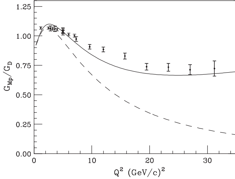
Figure 45: The proton magnetic form factor. The data [Si93], from SLAC, has been adjusted to account for the recent JLab measurements of G_E^p/G_M^p . The dashed curve is obtained [St02] by applying the phenomenological soft wave function of Ref. [Ra98a] of Eq. 10, and the solid curve results from the addition of a power law in k_\perp component to account for the quark high momentum tail.
