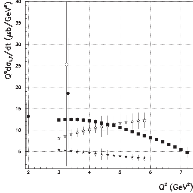
Figure 91: Projected CLAS ++ data for a Rosenbluth separation of ep \rightarrow en\pi^+ for x_B = 0.45 , -t = 0.5 \text{ GeV}^2 .
