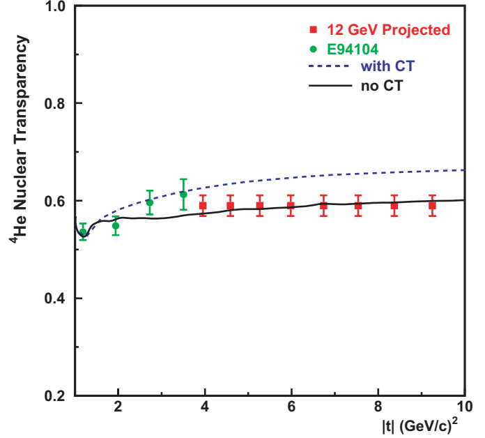
Figure 129: The projected results for nuclear transparency for photo-pion production from a ^4\text{He} target together with results from E94-104 [Du03]. The lines are color transparency calculations from Ref [Ga96].
