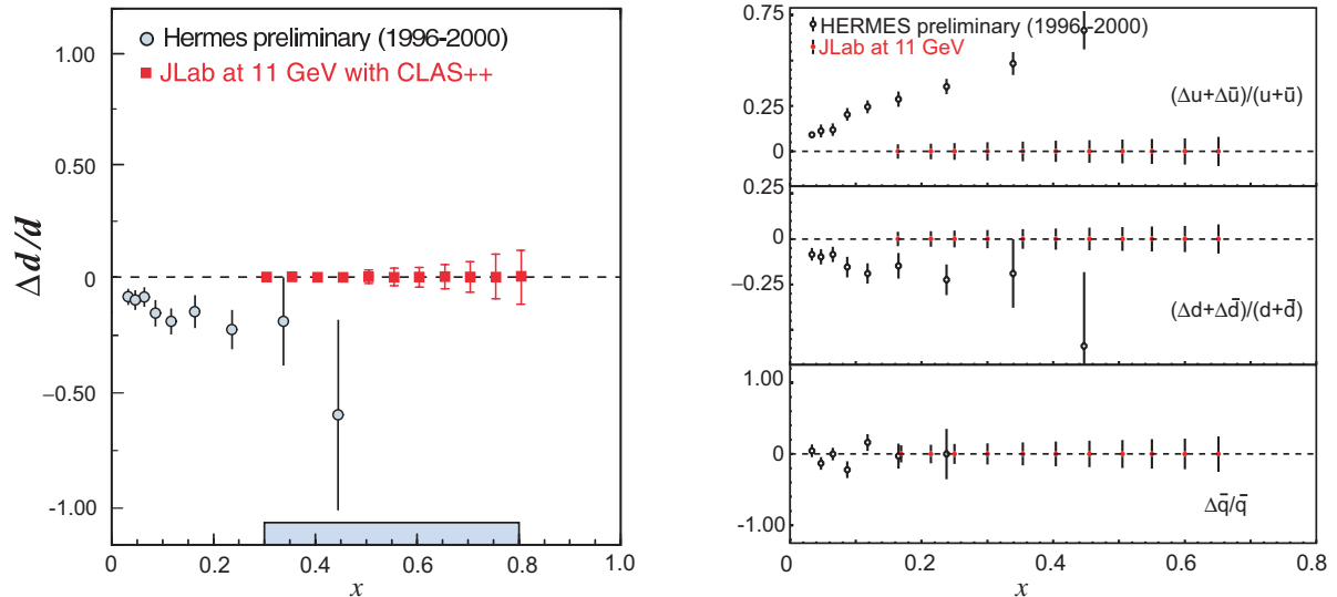
Figure 66: Projected errors for the ratio of polarized to unpolarized quark distribution functions compared with HERMES data. Left panel: d quark ratio from an 80 day measurement in Hall B. The solid curve uses constituent quark model wavefunctions, while the dashed uses pQCD-constrained fits to the world data. Right panel: Ratios for various flavors from 1000 hours of beam time on polarized \text{NH}_3 and ^3\text{He} targets in Hall A. Error bars are statistical only.
