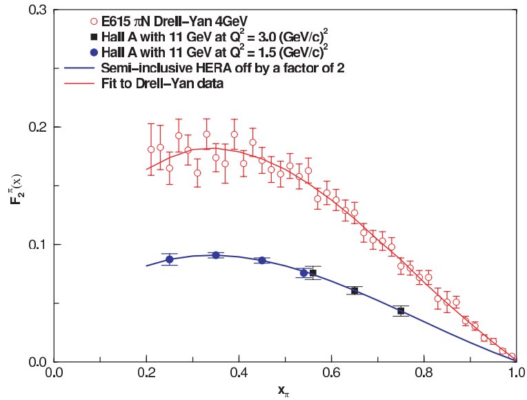
Figure 68: Simulated data for the pion structure function at Q^2 = 1.5 (filled circles) and 3.0 (\text{GeV}/c)^2 (squares) using the MAD spectrometer in coincidence with a low energy neutron detector at 11 GeV beam in Hall A, for a 25-day run period. Existing data from the Fermilab E615 experiment [Co89] are shown for comparison (open circles).
