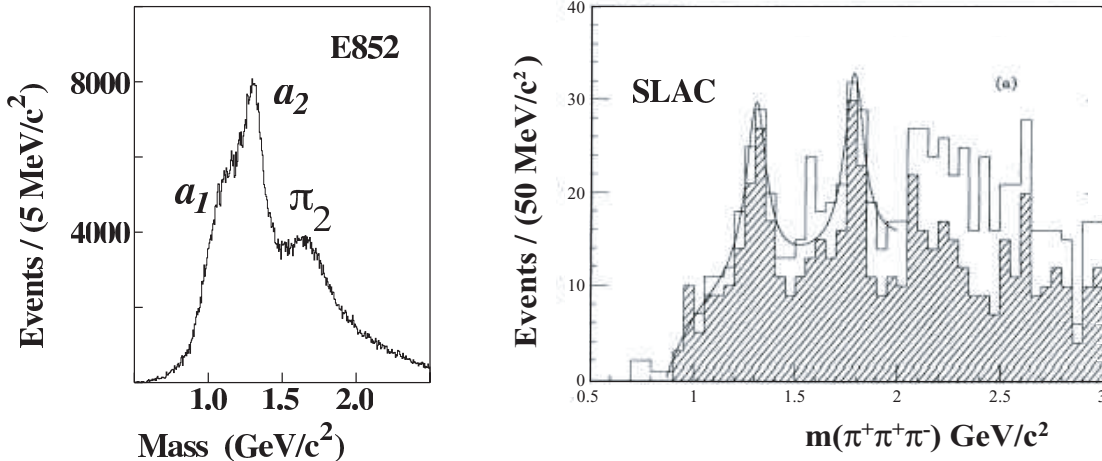
Figure 38: (left) The 3\pi mass spectrum from the reaction \pi^- p \rightarrow \pi^+ \pi^- \pi^- p at 18 GeV/c from E852 at Brookhaven. (right) The 3\pi mass spectrum from the reaction \gamma p \rightarrow \pi^+ \pi^+ \pi^- n at 19 GeV from SLAC. The shaded area identifies the portion of the 3\pi spectrum that included a \rho meson.
