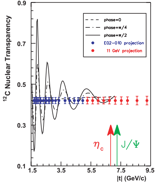
Figure 128: The projected results for nuclear transparency for photo-pion production from a ^{12}\text{C} target. The lines are calculations from Ref [Ja02].
