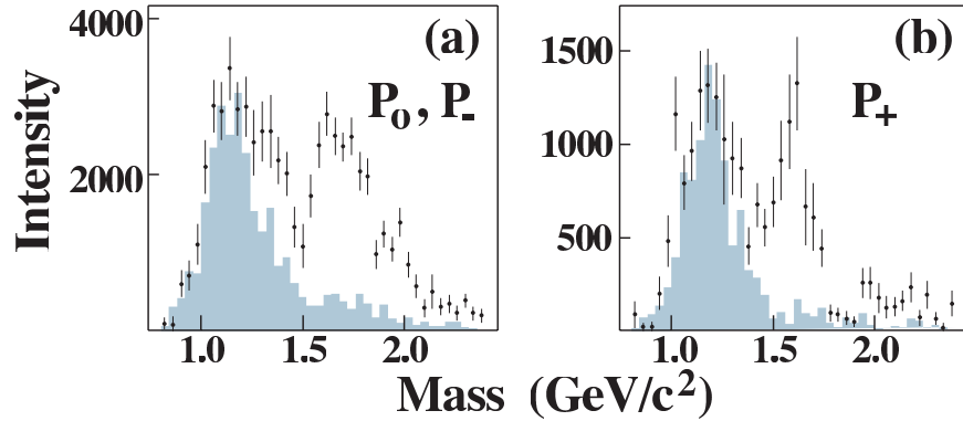
Figure 34: The intensities for the waves corresponding to 1^{-+} into \rho\pi . The shaded distributions are an estimate of leakage due to non-exotic waves (from E852 [Ad98]).
