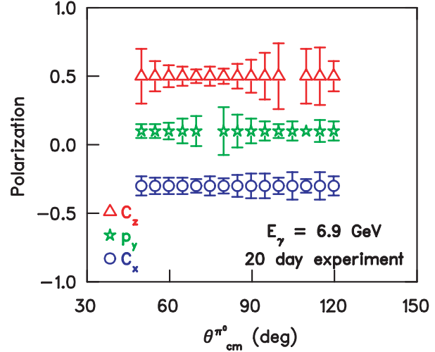
Figure 127: Estimated uncertainties for the induced polarization in \bar{\gamma}p \rightarrow \bar{p}\pi^0 for E_\gamma = 6.9 GeV, as a function of \pi^0 angle. The value chosen for the polarizations is arbitrary. Three weeks of beam time is assumed. Similar quality angular distributions would be obtained at the same time for several additional 200 MeV bins in photon energy. See text for further details.
