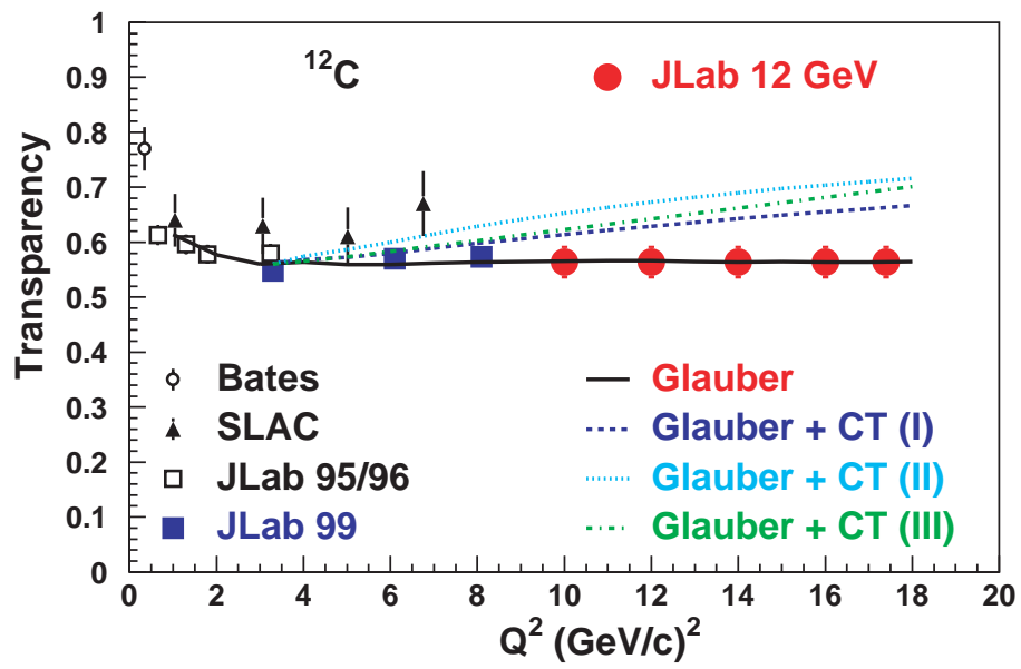
Figure 103: The Q^2 -dependence of nuclear transparency. The data are from Refs. [Ga92, Ne95, Ab98, Ga02], while the circles are projected uncertainties for a one week run at 12 GeV.
