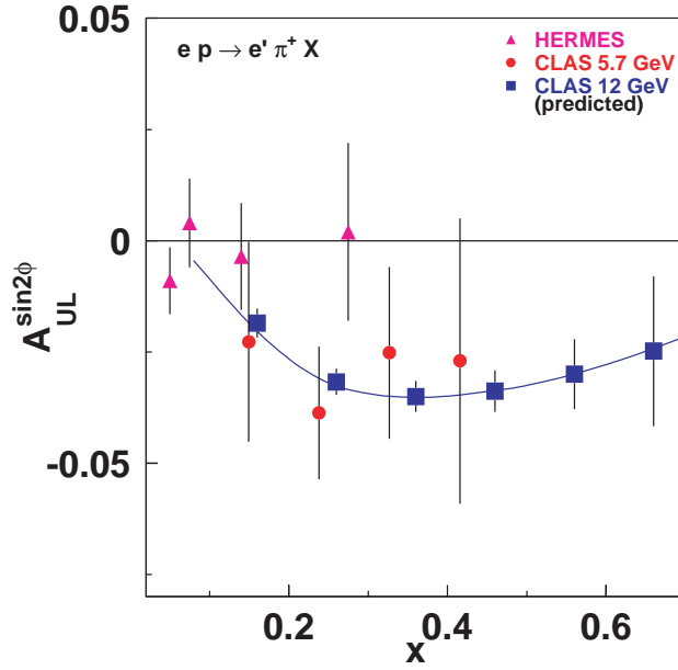
Figure 97: Target SSA: The shape of the A_{UL}^{\sin 2\phi}(x) measured with a longitudinally polarized target depends only on the ratio of the TMD distribution h_{1L}^{\perp} and f_1 , providing a direct access to h_{1L}^{\perp} . The curve is the theory prediction based on the Collins mechanism [Ef01]
