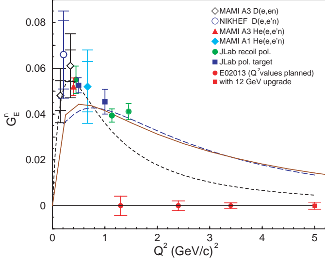
Figure 48: The neutron electric form factor G_{E_n}^n . Current data is plotted as open black circle [Pa99], open black diamond [Os99], filled red triangle [Zh01] and filled cyan diamond [Ro99]. The filled green circles [Ma93] are the Hall C JLab results employing recoil polarization, and the filled blue squares [Da93] are the Hall C results obtained using a polarized target. The filled red circles on the baseline are the projected Q^2 and errors for the approved experiment in Hall A [Ca02]. The filled red square at Q^2 = 5 (GeV/c) ^2 is the projection for Hall A with the 12 GeV upgrade. The curve denoted by black dashes is the Galster [Ga71] parameterization. The red solid curve is the result of a calculation due to Miller [Mi02]. The blue dashed curve is a result based on the GPD fit by Stoler [St03] to the proton form factors invoking isospin symmetry as in the previous figures.
