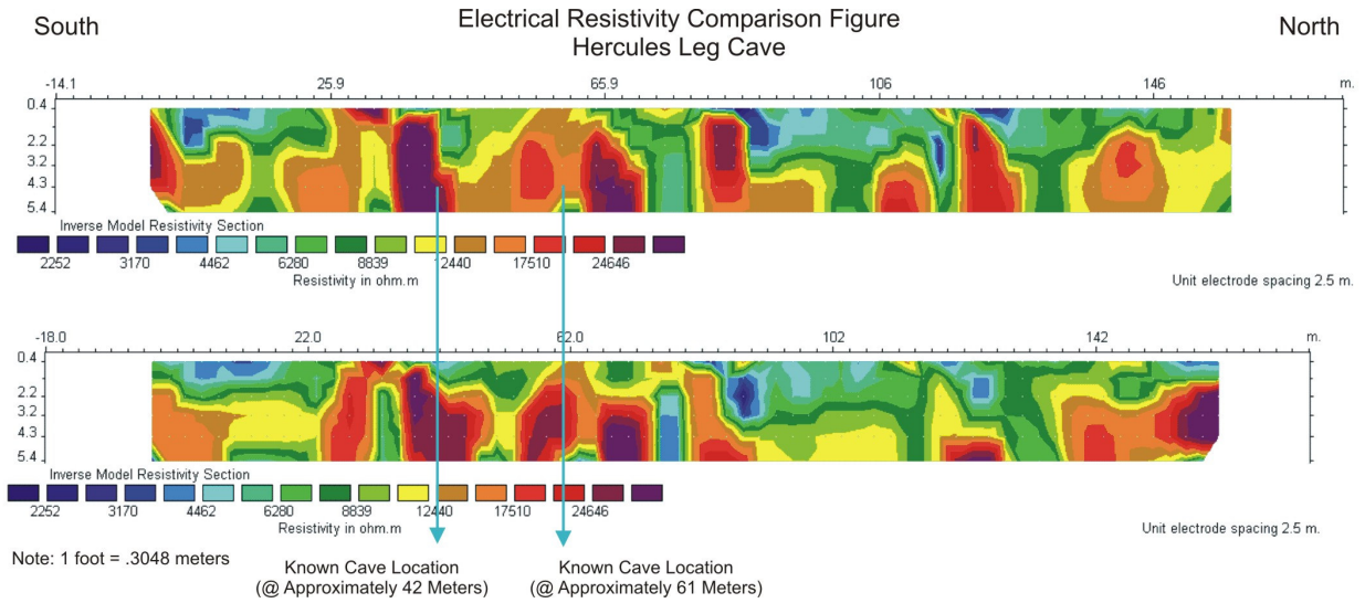
Figure 115. Cross Section. Electrical Resistivity Comparison.
