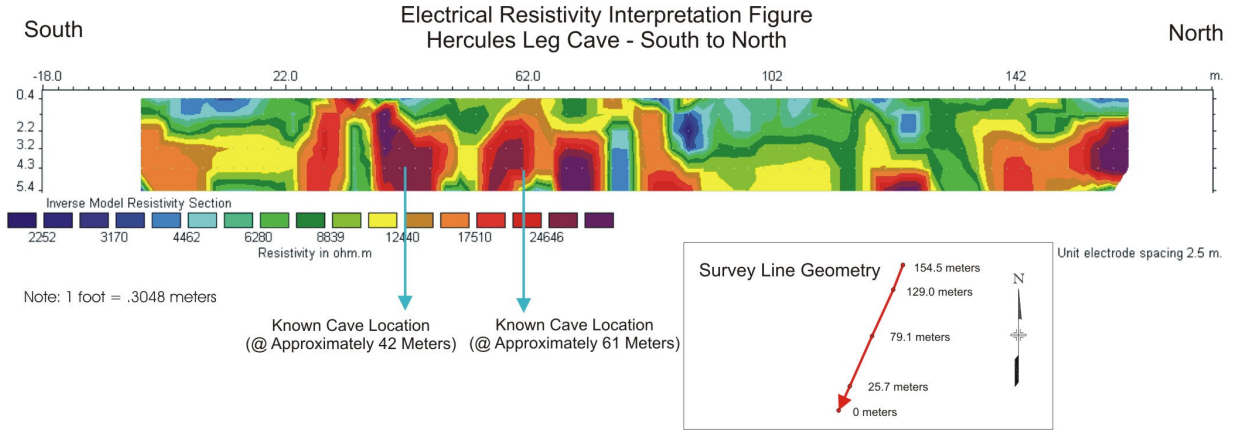
Figure 114. Cross Section. Electrical Resistivity Interpretation.
