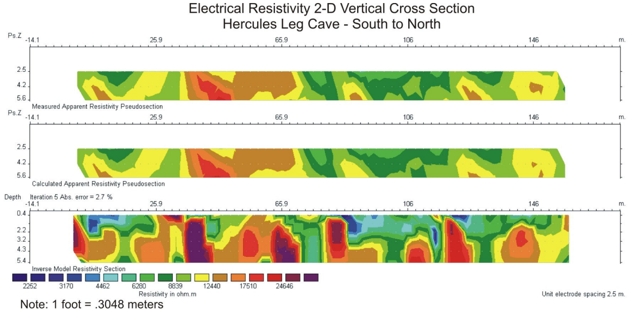
Figure 104. Cross Section. Electrical Resistivity Vertical 2-D.
