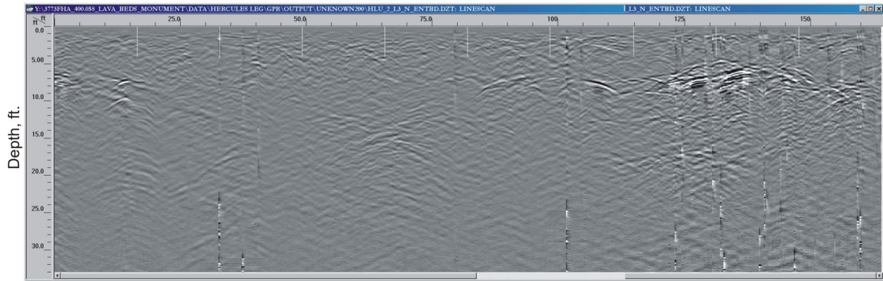
Processed GPR Data 200 MHz Antenna - Line 3 Hercules Leg Cave - Part 2
