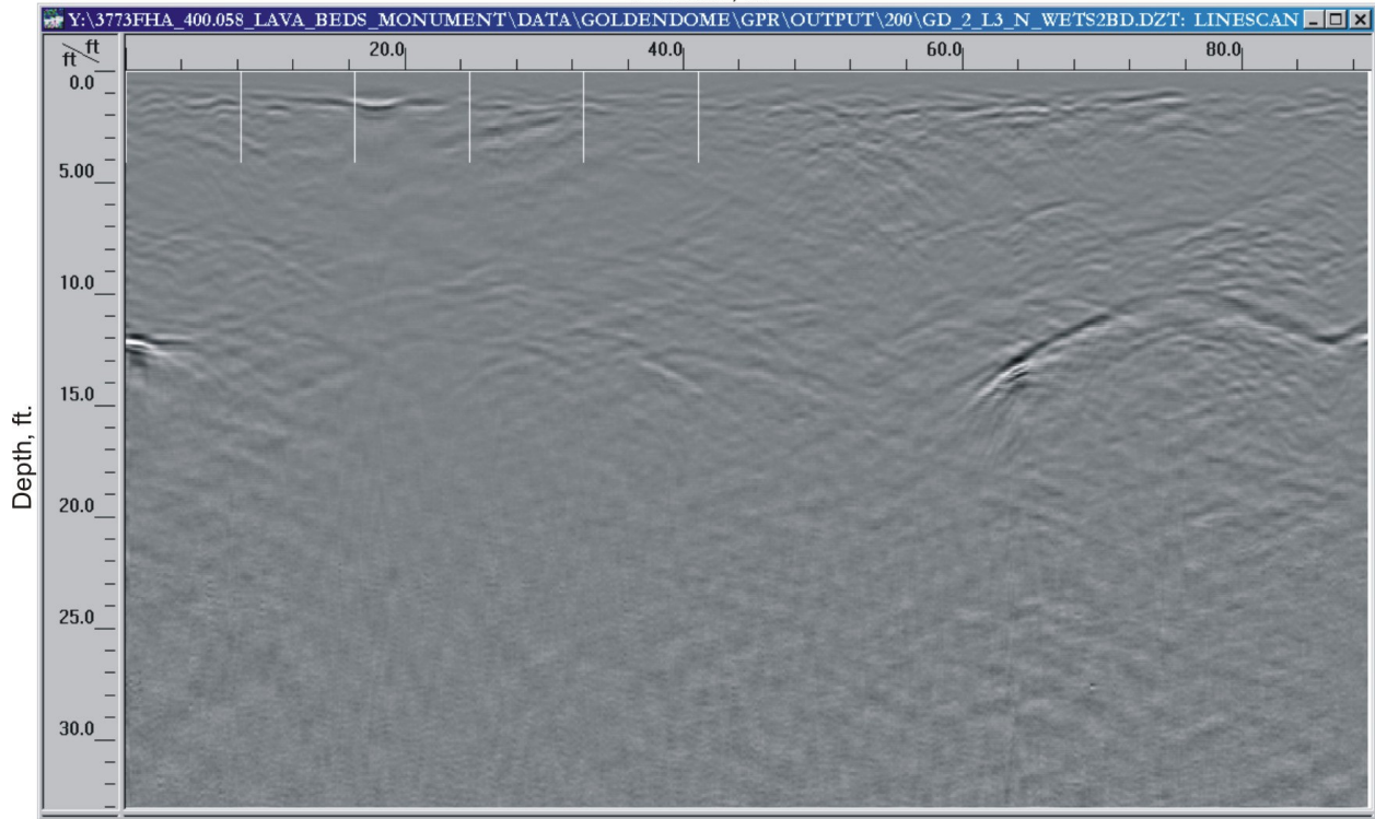
Processed GPR Data 200 MHz Antenna - Line 3 Golden Dome Cave Distance, ft.
