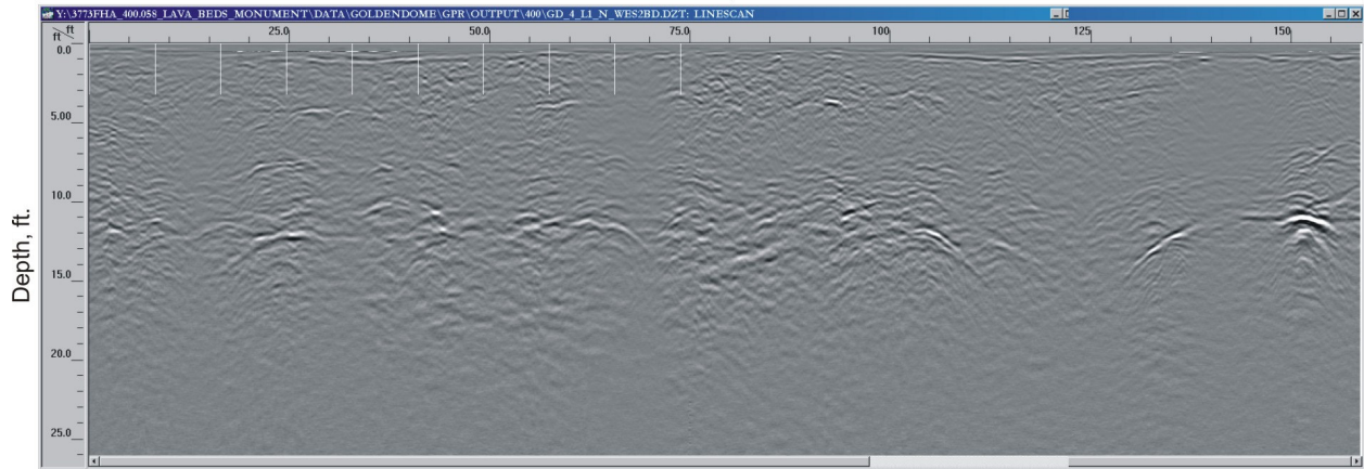
Processed GPR Data 400 MHz Antenna - Line 1 Golden Dome Cave Distance, ft.
