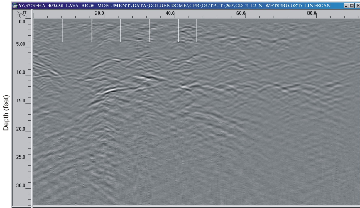
Figure 65. Cross Section. GPR data.
