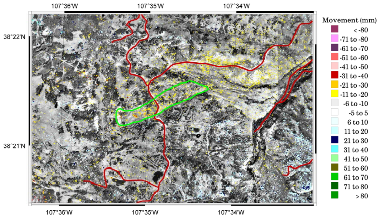
Figure 44. Graph. InSAR derived height change for June 17 to July 11, 2004.
