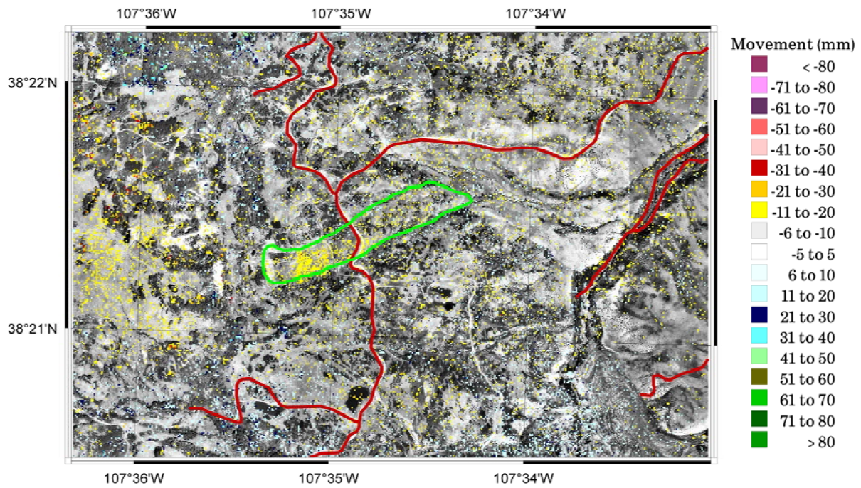
Figure 46. Graph. InSAR derived height change for September 21 to October 15, 2004.
