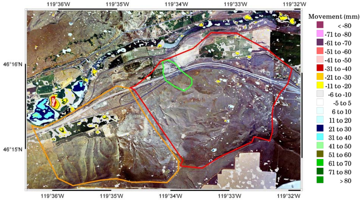
Figure 31. Graph. InSAR derived height change for October 24, 2004 to February 21, 2005.
