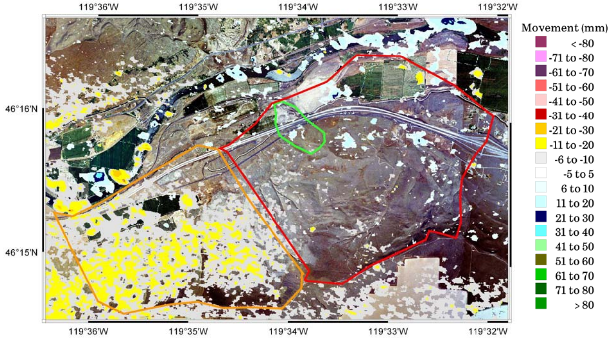
Figure 29. Graph. InSAR derived height change for June 26 to August 13, 2004.
