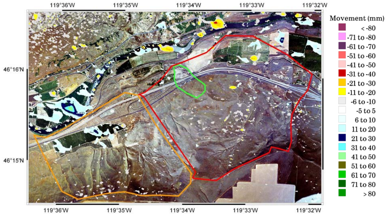
Figure 32. Graph. InSAR derived height change for February 21 to May 28, 2005.
