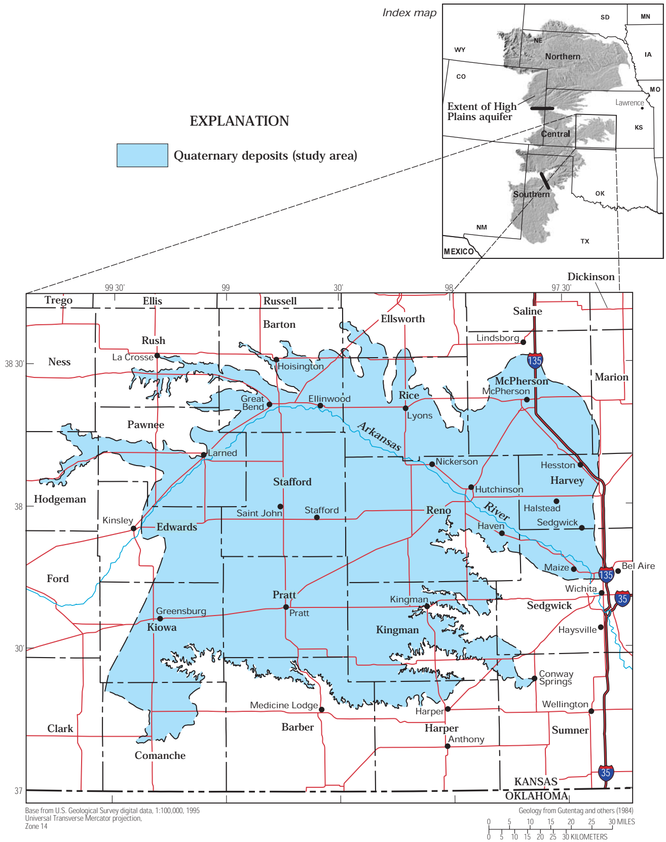
Figure 1. Location of High Plains aquifer and associated Quaternary deposits in south-central Kansas.
