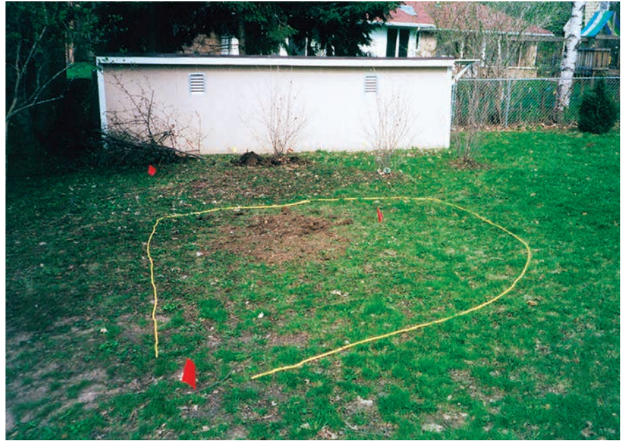
The perimeter of a rain garden is defined with string before digging.
