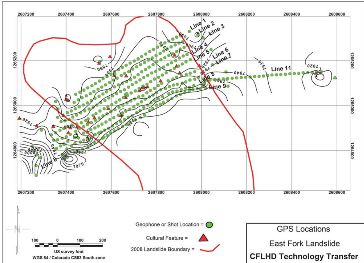
Figure 20. Map. GPS positions (culture, geophones and electrodes) and elevations for East Fork Landslide.
