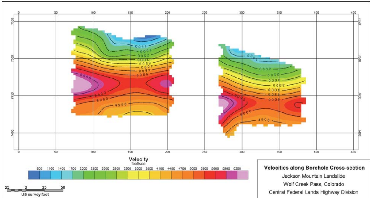
Figure 94. Model. Same cross-section as presented in Figure 92 showing only velocities below the surface where geophones were located.
