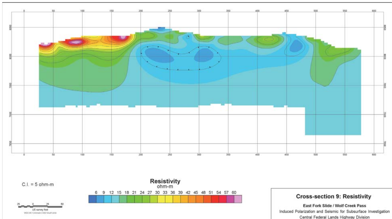
Figure 48. Plot. East Fork Landslide resistivity slice #9N.
