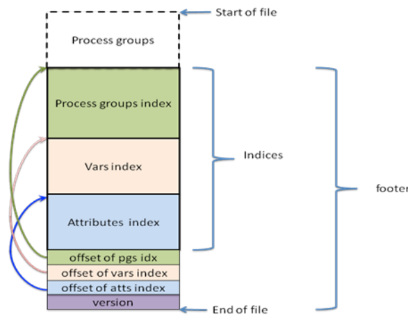
Figure 16. BP file structure
