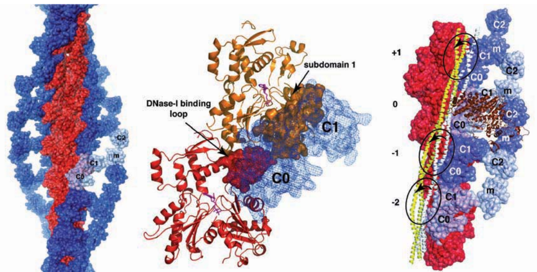
FIGURE 2: Left Model structure of C0C2 (blue) decorated actin (red) filaments based on the neutron scattering data. Middle Detailed view showing the C0 and C1 modules (blue) binding to neighbouring actin monomers (red and orange) in the filament. Right The actin filament (red) with a set of bound C0C2 molecules with the \text{Ca}^{2+} on (yellow) and off (white) positions of tropomyosin depicted. Note the strong steric clashes for the \text{Ca}^{2+} off tropomyosin position.
