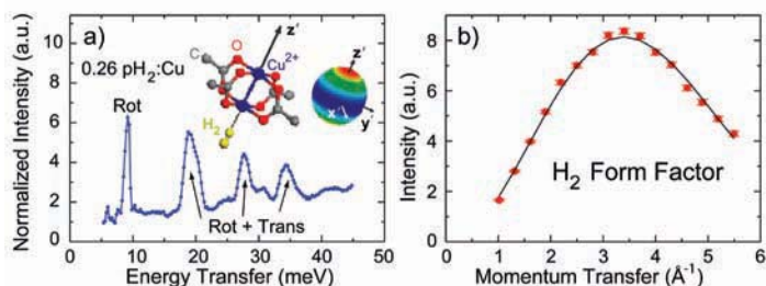
FIGURE 2: (a) Inelastic neutron scattering data for the H 2 adsorbed only at the Cu 2+ site in HKUST-1. Assignments of rotation (Rot) or translation (Trans) are made based both on experiment and with the aid of calculations. Inset: The local coordination for a classical DFT calculation as a function of the hydrogen rotation results in the orientational potential (perpendicular to the Cu-Cu axis (blue) is favorable; parallel orientation (red) is 78 meV less so). Solving for the rotational levels indicates that the transitions to the split first-level should appear around 9.6 meV and 37 meV. Calculated phonon energies x' = 9.56 meV, y' = 13.44 meV, and z' = 22.87 meV. (b) The assignment to a quantum rotational transition of the \approx 9.5 meV peak is determined from a separate measurement of the momentum transfer dependent intensity using the DCS spectrometer.
