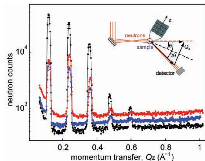
FIGURE 2: Neutron diffraction data collected at the AND/R (NCNR) for lipid multilayers samples with incorporated VSDs: Data displayed are for neat lipid (black), unlabeled VSD in lipid (blue) and deuterated VSD in lipid (red). The inset is a schematic illustration of the experimental setup.
