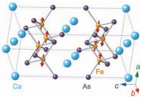
FIGURE 1: Illustration of the crystal structure of \text{CaFe}_2\text{As}_2 , and the antiferromagnetic structure below the structural/magnetic transition. The magnetic unit cell is the same as the orthorhombic chemical unit cell. The Fe moments are oriented along the orthorhombic a axis.
