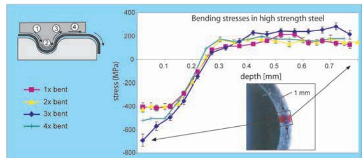
FIGURE 2: Stresses during a bending-backbending sequence on the high strength automotive steel HSLA50. Sheet thickness was 0.8 mm, the height of the measurement field was 1 mm (indicated) and the effective spatial resolution 0.05 mm.
