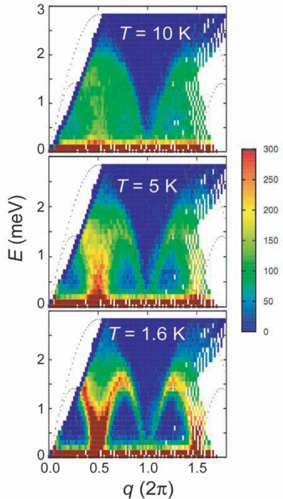
FIGURE 3: Maps of inelastic scattering from the quasi-one-dimensional spin-1/2 chain CuPzN [5] at three temperatures. Each data set required just 3.5 h of neutron counting.
