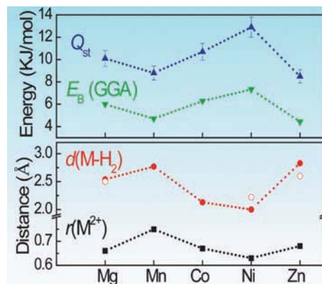
FIGURE 3: In the upper panel the experimental isosteric heat of adsorption ( Q_{st} , blue triangles) and the calculated GGA binding energy ( E_b (GGA) green triangles) of the isostructural series of MOF-74 compounds are found to behave similarly. In the lower panel the empirical transition metal ion radius ( r , black squares) and calculated M-H 2 distance ( d , red filled circles) correlate well with d (M-H 2 ) extracted from neutron powder diffraction data (red circles, filled white).
