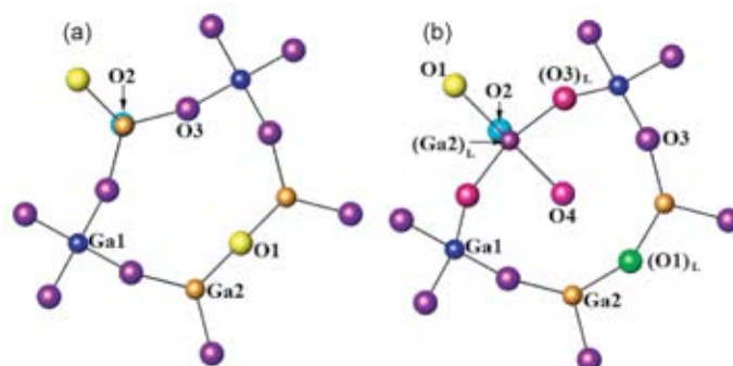
FIGURE 3: Structural relaxation around the interstitial oxide. The bulk structure (a) and local defect structure (b) around the oxygen interstitial O4. (\text{O}1)_L is, unlike (\text{O}3)_L , not directly bound to (\text{Ga}2)_L but relaxes away from interstitial O4, accommodated by a change in bond and bridging angles at Ga2. The O2 above the two Ga2 centers was omitted for clarity.
