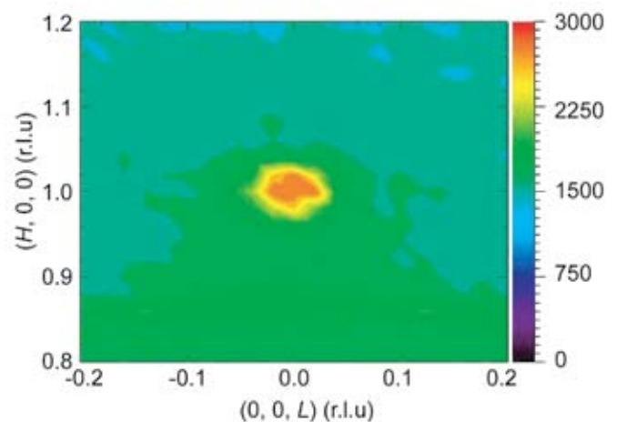
FIGURE 2: Neutron scattering intensity map measured at 300 K on a slow-cooled single crystal of \text{Fe}_{0.81}\text{Ga}_{0.19} . Under slow-cooled conditions, \text{Fe}_{0.81}\text{Ga}_{0.19} exhibits a long-range ordered structure with DO_3 symmetry, for which a (1,0,0) reflection is allowed. The diffuse scattering observed in the quenched crystal is absent. The diffuse scattering located below the line H = 1 and shown in green is believed to be size-effect scattering.
