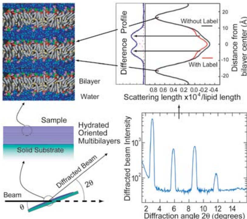
FIGURE 1: A lipid film containing 1 peptide per 25 lipids was deposited on a glass substrate and hydrated through the vapor phase to generate oriented fluid multibilayers, left . The oriented sample was placed in the AND/R beam, and Bragg diffraction peaks were collected in a \theta - 2\theta scan, bottom . The bilayer scattering length profiles, upper right , are generated from the diffraction peaks using a Fourier transform. Isomorphous replacement of lipids or peptides in the bilayer with specifically deuterated variants allows for the localization of the labels in the bilayer using difference profiles, top . Bilayer image courtesy of Dr. Scott Feller.
