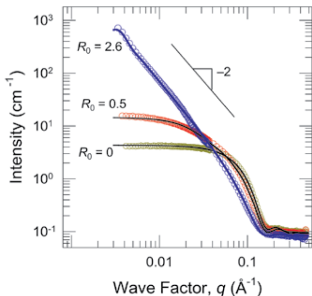
FIGURE 3: SANS spectra from lipid mixtures in deuterated cyclohexane for different C_4 -lecithin:lecithin molar ratios R_0 . The samples contain 20 mmol/L total lipid and 3.5 mmol/L NaCl.
