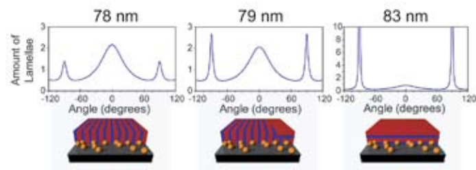
FIGURE 3: Best-fit orientational distribution of lamellae for the samples shown in Figure 2 (top row). The vertical peaks ( 0^\circ ) are broader than the horizontal peaks ( \pm 90^\circ ). Schematics of orientational order (bottom row) can be constructed from the distribution.
