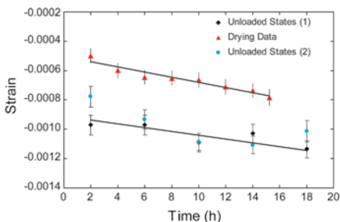
FIGURE 2: Comparison of strains from a drying test with the strains of the unloaded states. The measured \text{Ca}(\text{OH})_2 lattice strains characterize the behavior of a minority constituent; the behavior of the cement paste aggregate as a whole is better captured with surface attached strain gages. The comparison of suitably normalized lattice strains and macroscopic strains is shown in Fig. 3.
