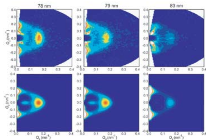
FIGURE 2: Rotational SANS reciprocal-space reconstructions for three different film thicknesses (top row) show varying intensity of the vertical peak. The associated best-fit models (bottom row) provide insight into the angular distribution of the lamellae.
