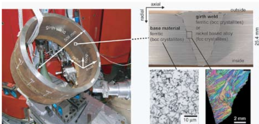
FIGURE 1: Neutron diffraction geometry for a large pipe section with girth weld in the tangential measurement direction. The right side shows the cross section of the fully austenitic girth weld and micrographs. Note the sharp boundary between the crystallographically different base metal and the weld metal (outlined by the dashed line). The micrograph for the ferritic weld metal is not shown, but grains sizes are of the same order of magnitude as the base metal.
