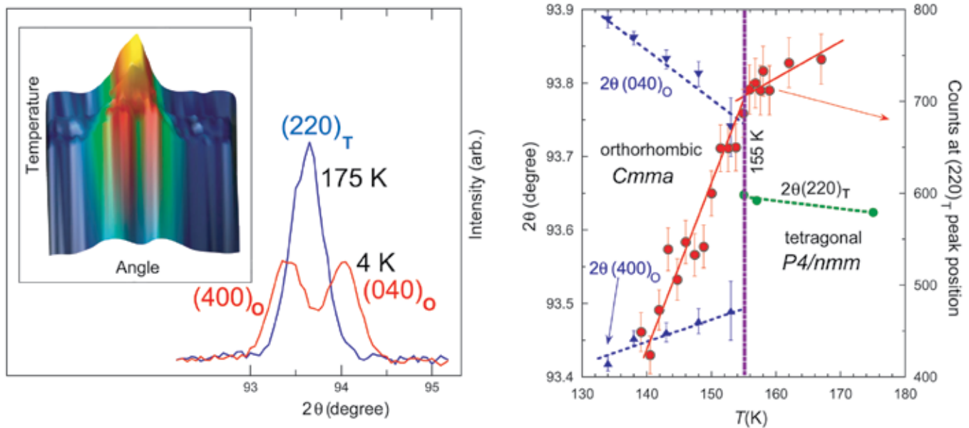
FIGURE 1: Temperature dependence of the [2,2,0] structure reflection. Left: The diffraction intensity profile in the inset shows that the angle dependence of the (2,2,0)_T reflection abruptly splits into two peaks [ [4,0,0]_O and [0,4,0]_O , [O] denotes orthorhombic] as a function of temperature. The graph shows the data at 175 K, and in the ground state at 4 K. A structural transition has occurred from the high temperature structure with tetragonal symmetry to orthorhombic symmetry [ Cmma ]. The right plot shows the intensity (red symbols) at the peak position for the tetragonal peak, which decreases rapidly below the transition at 155 K as the peak positions move apart. The fitted peak positions (blue and green symbols) are also shown, and indicate the abrupt nature of the transition.
