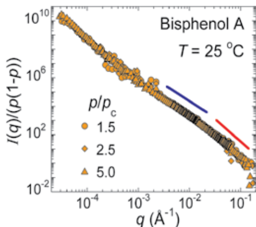
FIGURE 2: Concentration-effect corrected scattering data lead to a master curve indicating a hierarchical network structure over a wide range of length scales. The lines show slopes in two regions.
