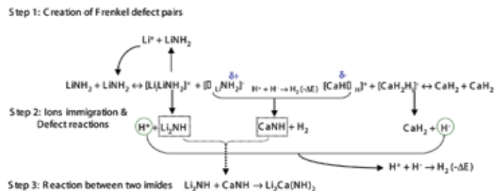
Scheme 1: Dehydrogenation of 2\text{LiNH}_2 + \text{CaH}_2 with a total of 2\text{H}_2 released and products of \text{CaNH} , \text{Li}_2\text{NH} and/or \text{Li}_2\text{Ca}(\text{NH})_2 observed at various desorption steps.
