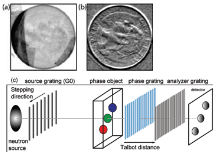
FIGURE 1: Comparison of the transmission image (a) to the neutron phase gradient image (b) of a U.S. quarter. The features of the quarter are not resolved in the transmission due to insufficient contrast. However, the eagle is clearly visible in the neutron phase gradient image. The setup is shown schematically in (c).
