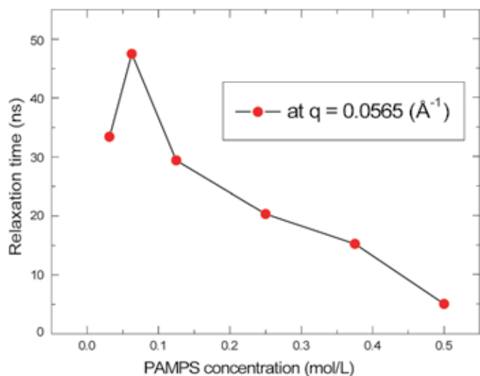
FIGURE 2: A maximum in the relaxation time of PAMPS ( \tau_{\text{agg}} ) is observed to locate at a PAMPS/ PAAm molar ratio of 1 to 7. [The line is a guide to the eye.]
