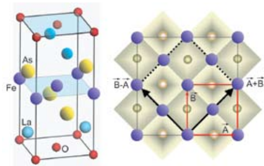
FIGURE 1: The crystal structure of LaOFeAs (left) and the top view of the FeAs-plane and the relations between primitive and \sqrt{2} \times \sqrt{2} -supercell used in our calculations. The dark and light shaded areas indicate the As atoms below and above the Fe-square lattice, respectively.
