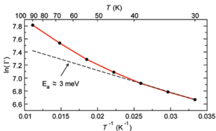
FIGURE 3: A plot of \ln(\Gamma) vs. T^{-1} for ZIF8 between 30 K and 90 K, where \Gamma (in \mu\text{eV} ) is the full-width-at-half-maximum quasielastic linewidth.
