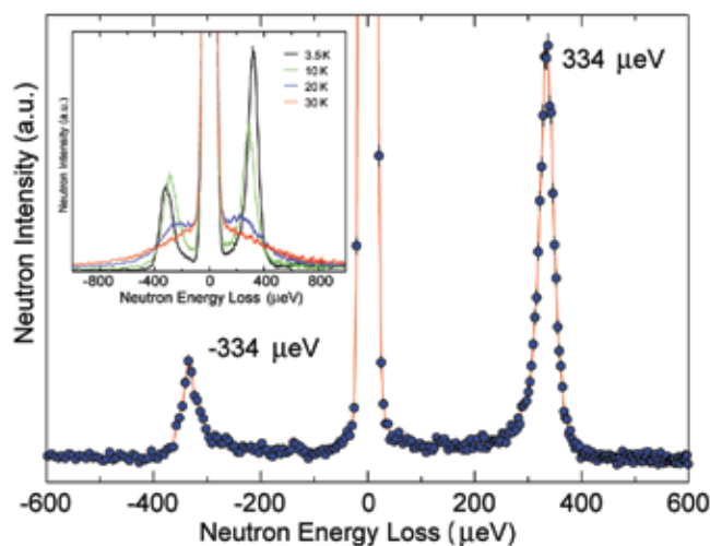
FIGURE 2: ZIF8 tunneling spectrum at 1.4 K using the DCS spectrometer with 7 Å neutrons ( \approx 18 \mu\text{eV} resolution). [inset] Evolution of the tunneling spectrum with temperature using the FCS spectrometer with 6 Å neutrons ( \approx 70 \mu\text{eV} resolution).
