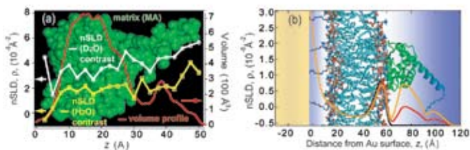
FIGURE 2: (a) Matrix (MA) domain oriented with membrane binding region on the left hand side. Volumetric profile and nSLD profiles were calculated using 2.5 Å slabs of MA along z taking into account exchangeable hydrogens on the protein. (b) Best fit nSLD profile of the tBLM system with no MA protein (black line), and bound MA protein at 1 mmol/L (red line) and 10 mmol/L (orange line) concentrations.
