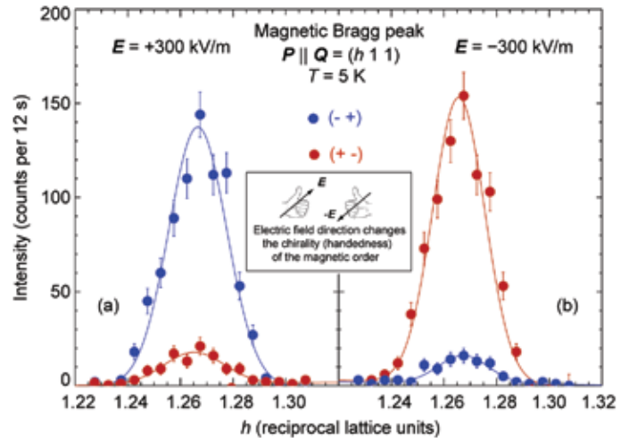
FIGURE 2: Full polarized neutron magnetic diffraction. The neutron polarization \mathbf{P} is parallel to \mathbf{Q} , [ \mathbf{P} \parallel \mathbf{Q} ], so that all the magnetic scattering is spin-flip. (a) A +300 kV/m electric field selects one chiral domain, and then the magnetic peak is only observed in the (- +) configuration; the small peak in the (+ -) configuration is due to the imperfect instrumental polarization. (b) With the ferroelectric polarization reversed by applying -300 kV/m, the magnetic Bragg peak is only observed in the (+ -) configuration.
