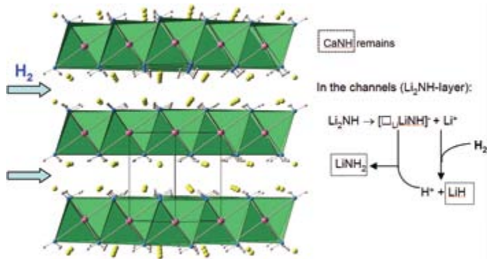
FIGURE 2: Structure of \text{Li}_2\text{Ca}(\text{NH})_2 viewed as an “intercalated” layered structure consisting of 2D slabs of \text{Ca}(\text{NH})_6 -octahedra separated by Li ion motifs. Ca, Li, N and H atoms are colored as in Fig. 1. The facile motion of Li assists the hydrogenation process with totally 1 \text{H}_2 absorbed and final products of \text{CaNH} , \text{LiNH}_2 and \text{LiH} .
