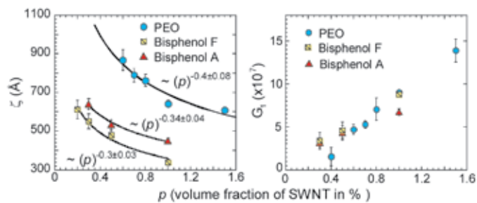
FIGURE 3: Concentration dependence of the network mesh size ( \zeta ) and G_1 in different matrices. The scaling of \zeta is consistent with diffusion limited floc formation while the nearly linear dependence of G_1 , roughly measuring floc number, suggests that the network primarily grows through new floc formation. Error bars are \pm 1 standard deviation.
