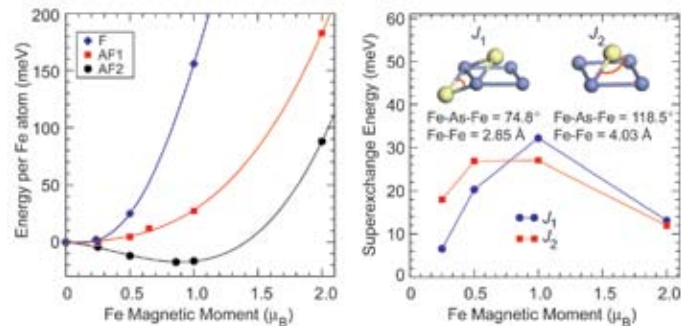
FIGURE 3: Left: The total energy per Fe atom versus magnetic moment for F, AF1 and AF2 spin-configuration, indicating AF2 is the only ground state of the system. Right: The magnetic interactions for nn and nnn Fe ions obtained from the energies of F, AF, and AF2 configurations.
