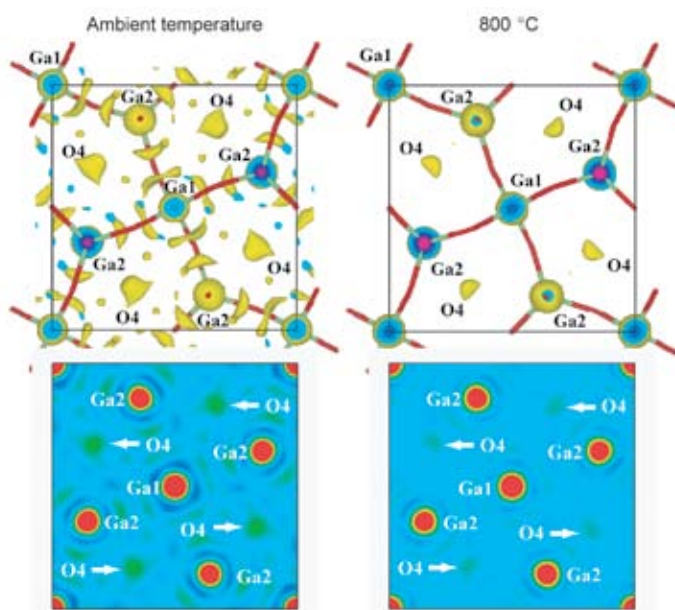
FIGURE 2: Comparison of the nuclear scattering density of \text{La}_{1.54}\text{Sr}_{0.46}\text{Ga}_3\text{O}_{7.27} as obtained from maximum entropy analysis maps. The [001] projections (top) and corresponding scattering density at z = 0 (below) are shown at ambient (left) and 800 °C (right).
