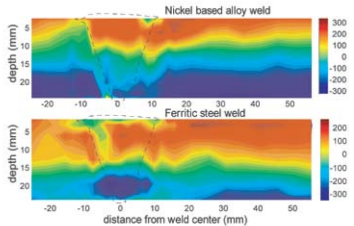
FIGURE 3: Comparison of axial stresses between the nickel-based alloy (top) and the ferritic weld (bottom). Stress levels are given in MPa. The dashed line corresponds to the girth weld region.
