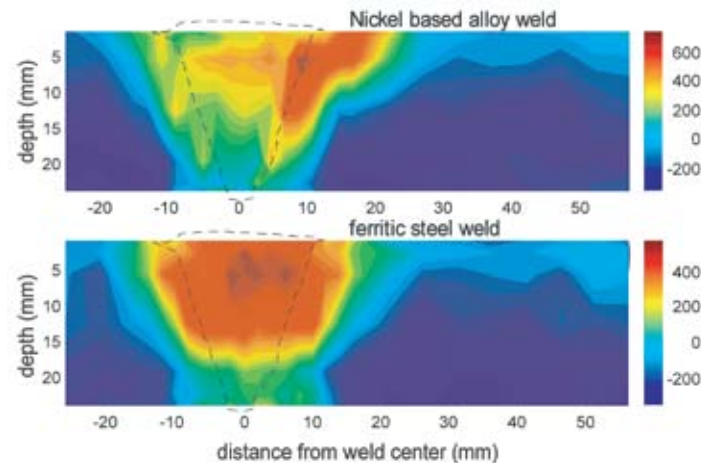
FIGURE 2: Comparison of hoop stresses between the nickel-based alloy (top) and the ferritic weld (bottom). Stress levels are given in MPa. The dashed line corresponds to the girth weld region.
