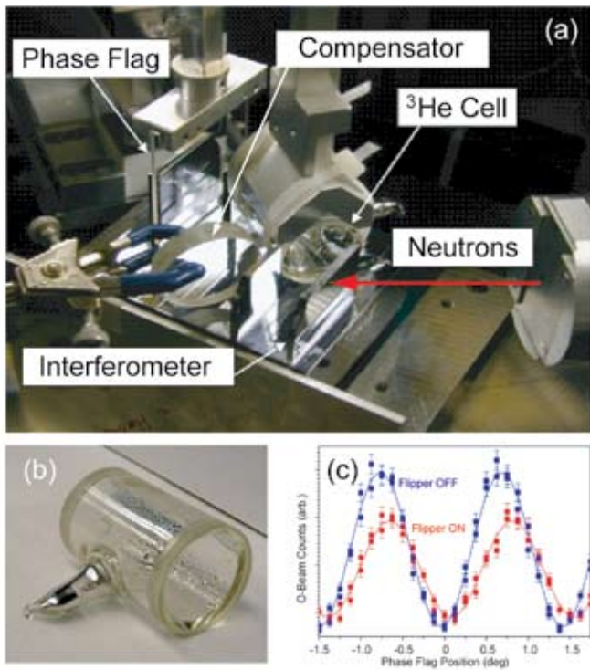
FIGURE 2: Experimental setup. (a) Neutrons enter from the right of the picture. One can see the compensation glass, the target cell, and the quartz phase flag. (b) One of the target cells used. Solid rubidium which is heated and used in Spin-Exchange Optical Pumping can be seen in the picture as dark spots along the cell walls. (c) A typical interferogram. The blue curve (lines are fits) is the O-beam intensity for when the neutron and ^3\text{He} spins are aligned parallel. The red curve is for when the neutron spin has undergone a spin flip. Lower intensity in the red curve is due to increased neutron absorption in that case. A phase shift around 30^\circ can be seen by comparing the two curves.
