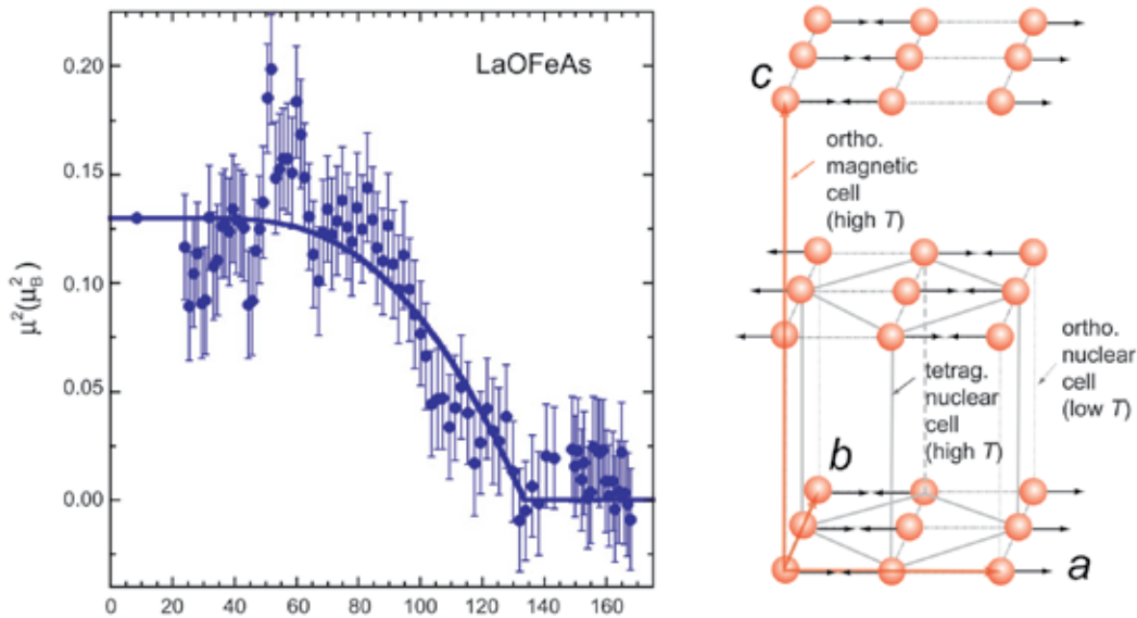
FIGURE 2: Temperature dependence of the order parameter for the strongest (1,0,3) magnetic reflection. Data were obtained in diffraction mode using the position-sensitive detector. The solid curve is a simple fit to mean field theory, which indicates that the order develops at a Néel temperature of T_N = 137(3) K. The figure on the right shows the antiferromagnetic structure of the system, giving a \sqrt{2}a_T \times \sqrt{2}a_T \times 2c_T magnetic unit cell. All the magnetic structures for this class of materials have antiparallel spins along the a direction and parallel spins along the b direction, with a > b and the spin direction along a . Both the magnetic and structural transitions are absent in superconducting \text{La}(\text{O}_{1-x}\text{F}_x)\text{FeAs} ( T_c = 26 K).
