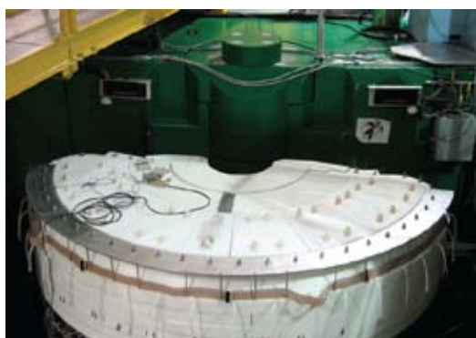
FIGURE 1: MACS in place at the cold neutron beam port NG-O.
