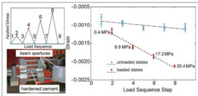
FIGURE 1: Compressive tests of cement paste prisms (10 mm × 10 mm × 15 mm) in loading-unloading cycles. The strain follows the applied load in linear dependence. However, with increasing time and water evaporation the strains in the unloaded states (0.43 MPa) become more compressive. A subsequent drying measurement of an unloaded sample during water evaporation revealed that the strains in the unloaded states exhibit a similar rate as the shrinkage strains originating from dehydration/evaporation only (Fig.2).
