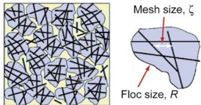
FIGURE 1: A schematic diagram of the hierarchical network structure showing two different length scales; we note that there can be quite a range of mesh sizes, \zeta , and floc sizes, R .
