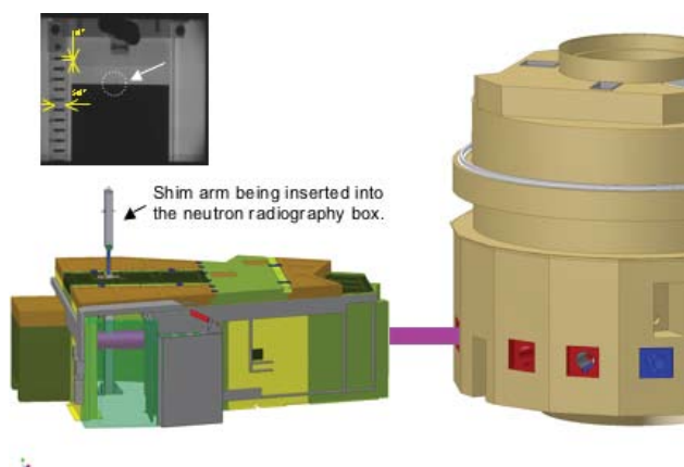
FIGURE 1: Shim arm Cadmium burnup monitored by neutron radiography. As an example of resolution, the inset radiogram shows an edge of the Cd layer.
