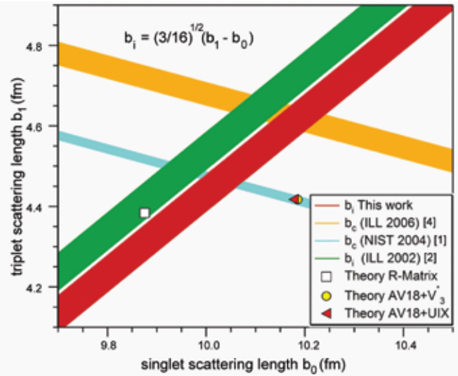
FIGURE 3: Experimental results found in [1], [2], and [4] compared with predicted values of some NN+3NI theoretical models [5]. The coherent scattering length measured in Refs. 1 and 4 is given by b_c = 3/4 b_1 + 1/4 b_0 . The results are shown as bands representing the result \pm one standard deviation, \sigma .
