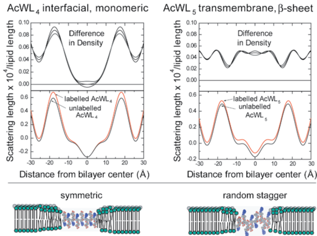
FIGURE 2: Transbilayer scattering length profiles of fluid bilayers containing either the monomeric, interfacial peptide AcWL 4 , left , or the oligomeric, transmembrane \beta -sheet peptide AcWL 5 , right . Experiments were done with 1 peptide per 25 lipids. Isomorphous replacement was achieved by substituting protonated peptide with peptide containing two consecutive deuterated leucine residues. The difference profiles, top , show the average location of deuterium labeled leucines in the bilayer \pm experimental uncertainty. While AcWL 4 shows the expected interfacial localization, the oligomeric AcWL 5 deuterons are present all across the membrane. Thus the transbilayer disposition of the peptide \beta -sheets must be randomly staggered rather than regular and symmetric as in existing models, bottom
