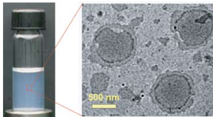
FIGURE 2: Photograph of sample vial and TEM micrograph of structures present in a C_4 -lecithin + lecithin sample at R_0 = 2.6 (total lipids = 20 mmol/L, [NaCl] = 3.5 mmol/L).
