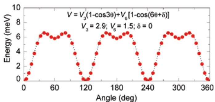
FIGURE 4: Rotational potential of the methyl group in ZIF8, obtained from DFT calculations. Dotted lines are the fit to a 3-fold/6-fold mixed potential.
