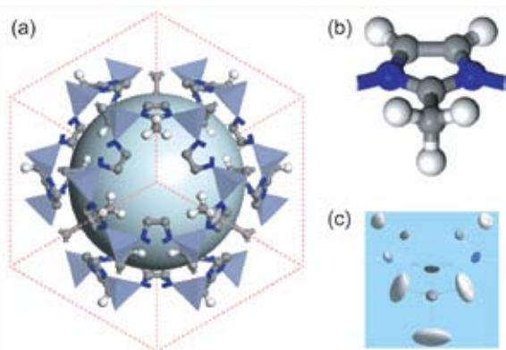
FIGURE 1: [a] ZIF8 crystal structure of [space group I4\bar{3}m ]. The 3-D open framework consists of ZnN_4 clusters (the tetrahedra) connected by 2-methylimidazolate [MeIM] linkers. The central space-filling sphere denotes the pore structure. For clarity, only the H atoms associated with the methyl groups are shown. [b] The structure of the MeIM linker. [c] The ellipsoids of the MeIM linker obtained from ZIF8 neutron-diffraction data at 3.5 K.
