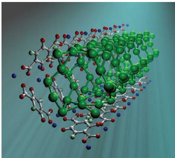
FIGURE 2: One dimensional nanoscale tube-like structure formed from adsorbed D_2 . D_2 molecules [large green spheres] adsorbed in the hexagonal pores of MOF-74 [partial cross-section shown for clarity. Zn : blue, C : grey, O : red, H : pale green] form a one-dimensional nanoscale tube-like structure from the first three adsorption sites. Deuterium molecules are connected if the distance between D_2 molecules is less than 3.65 Å.
