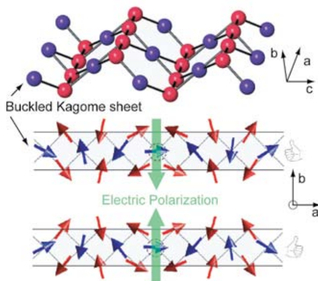
FIGURE 1: [top] Single layers of a \text{Ni}^{2+} Kagome lattice that are buckled along the c -axis, and that in \text{Ni}_3\text{V}_2\text{O}_8 are stacked along the b -axis. [Center/Bottom] spiral magnetic structure that is only possible because of a crystal distortion that also leads to macroscopic electric polarization, either up or down depending on the sense of rotation of the spiral.
