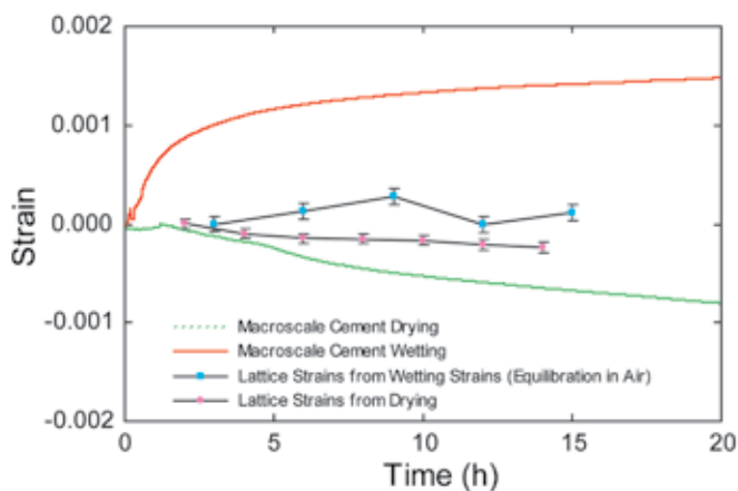
FIGURE 3: Comparison between macro-strain and lattice strain measurements for in both the wetting and drying environment. The lattice strains from wetting are for a dry sample being equilibrated in room air.
