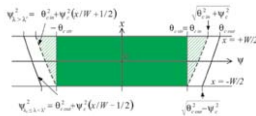
FIGURE 1: The acceptance diagram (transverse position x vs trajectory angle \psi ) of a curved/straight guide system that is constrained by \vartheta_{cin} = \vartheta_{cstr} .
