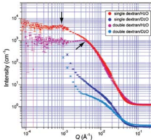
FIGURE 3: – SANS/USANS data showing the interaction peak in the double dextran sample with a concentration of 25.6 mg/ml at Q. 4H10^{-3} \text{ \AA}^{-1} (radius = 157 nm), and the possible interaction peak in the single dextran layer sample with a concentration of 21.8 mg/ml at Q. 9H10^{-4} \text{ \AA}^{-1} (radius = 698 nm).
