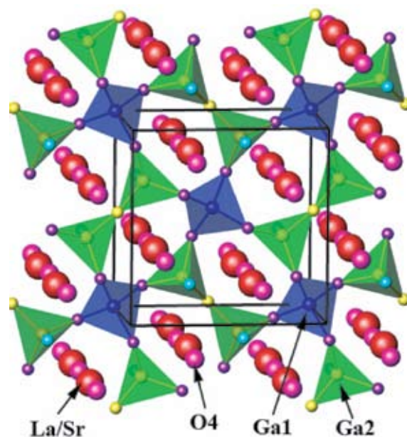
FIGURE 1: Structure of \text{La}_{1.54}\text{Sr}_{0.46}\text{Ga}_3\text{O}_{7.27} which stabilizes in the melilite structure. The O4 positions indicate additional interstitial oxygen ions, not found in the parent structure.
