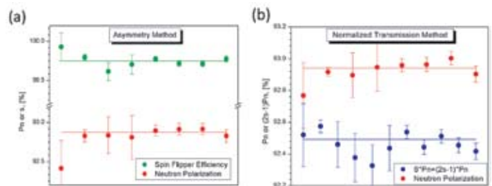
FIGURE 1: Polarization analysis using two different techniques. (a) The results from the Asymmetry Method for both the neutron polarization, P_n , and the spin flipper efficiency, s in percent versus measurement instance. (b) The polarization results using the Normalized Transmission Method. Here the spin flipper efficiency is not directly measured but instead the product (2s-1) \cdot P_n is. In both cases drawn lines are fit to the data. Both techniques agree with each other with a relative uncertainty of less than 0.001.
