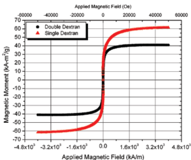
FIGURE 2: – Magnetization vs. field loops show the same shape except for a 33 % difference in saturation magnetization between the double and single dextran samples.
