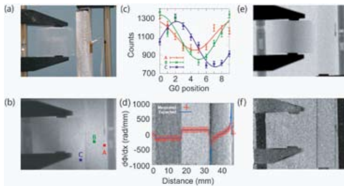
FIGURE 2: Talbot optics measurement. (a) A sapphire wedge and single crystal aluminum cylinder are a simple model system. (b) The raw image with the source grating (G0) stepped to the 4th position. (c) The interference pattern of points A, B, and C labeled in (b). (d) The neutron phase gradient image, and a plot of the average gradient and the expected phase gradient for the wedge and cylinder. (e) The transmission radiograph. (f) The dark-field image, which clearly shows the rough edges of the aluminum cylinder.
