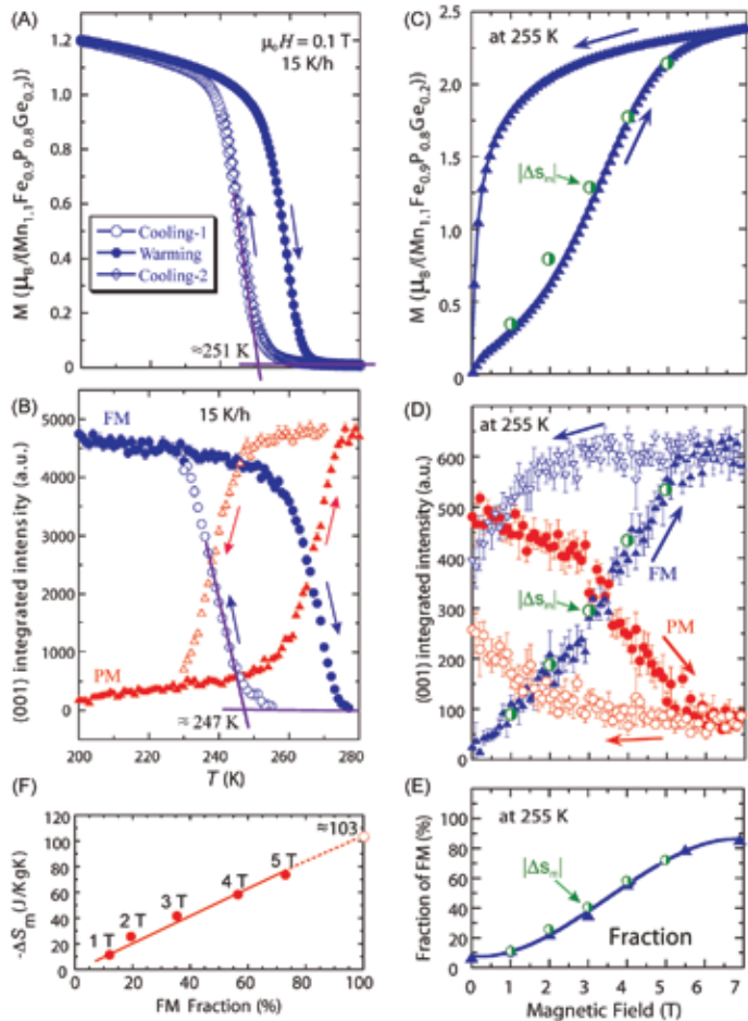
FIGURE 1: Comparison of the diffraction and magnetization measurements. (A) Temperature dependence of the magnetization in an applied field of 0.1 T. (B) Integrated intensities of the (001) reflections for the PM- and FM- phases as a function of temperature on cooling and warming. (C) Field-dependent magnetization at 255 K. The magnetic entropy change |\Delta S_M| , normalized to the magnetization, is shown for comparison. (D) Field dependence of the integrated intensities of the (001) reflections for the PM-phase and FM-phase at 255 K, showing that the FM-phase fraction tracks the magnetization data and normalized magnetic entropy change |\Delta S_M| . (E) Fraction of the FM-phase at 255 K as the field increases. The FM-phase fraction increases smoothly to \approx 86\% . Data normalized from |\Delta S_M| are shown for comparison. (F) |\Delta S_M| increases linearly with the FM-phase fraction. |\Delta S_M| is projected to be \approx 103 J/Kg K if the transition went to completion for this sample.
