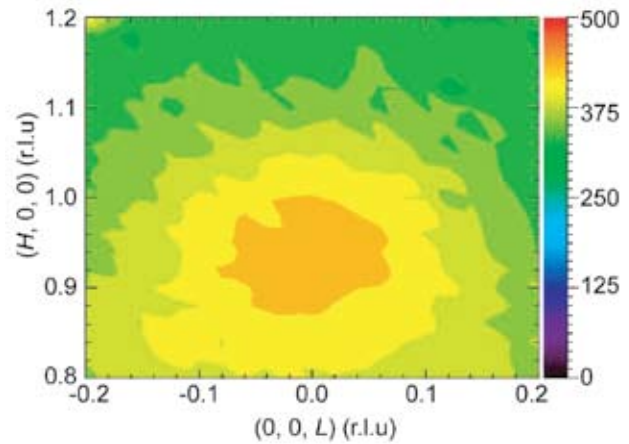
FIGURE 1: Neutron scattering intensity map measured at 300 K on a furnace-cooled single crystal of \text{Fe}_{0.81}\text{Ga}_{0.19} . The symmetry of the underlying matrix allows no (1,0,0) reflection. The broad diffuse scattering that peaks near (0.95,0,0) thus indicates the presence of a short-range ordered structure having a different symmetry and lattice spacing.
