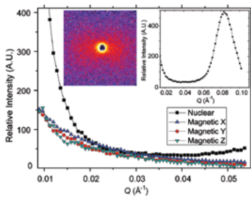
FIGURE 1: Magnetic and nuclear separation in a remanent magnetic field. The left inset is an asymmetric spin-flip scattering SANS pattern. The right inset shows nuclear scattering at larger Q . In the main plot nuclear scattering [black] is distinct from magnetic scattering [red and green: perpendicular to neutron polarization, blue: parallel].
