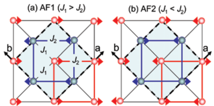
FIGURE 2: Two antiferromagnetic configurations considered in this study.
