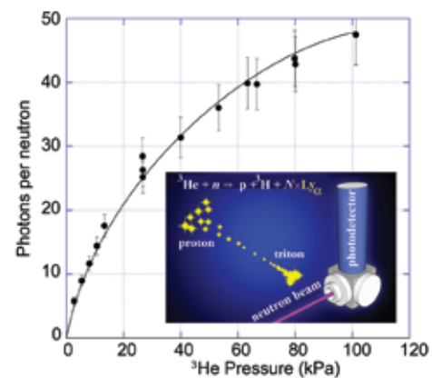
FIGURE 1: Lyman alpha photon yield per reacted neutron as a function of 3 He pressure. The inset states the nuclear reaction and the cartoon indicates photon production and the experimental setup.
