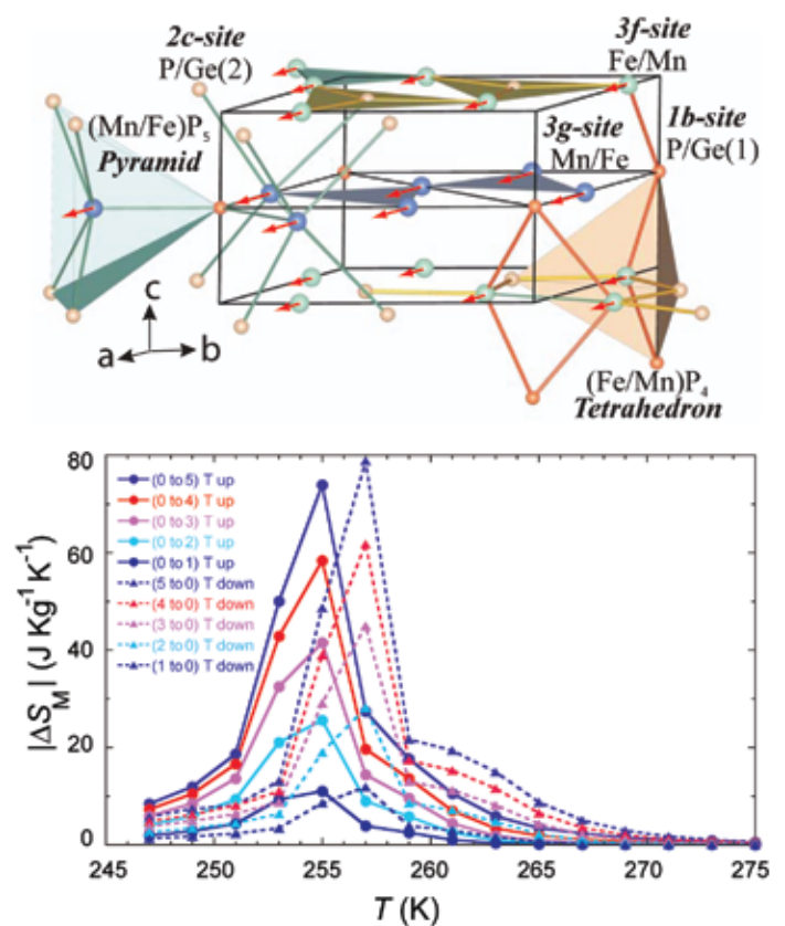
FIGURE 2: The Magnetocaloric Effect. Temperature dependence of the entropy change of the bulk Mn_{1.1}Fe_{0.9}P_{0.8}Ge_{0.2} compound as a function of applied magnetic field up to 5 T. The upper panel shows the crystal structure for the FM-phase which differs from that in the PM-phase in the ordering of the spins and the lengths of a , b , and c .
