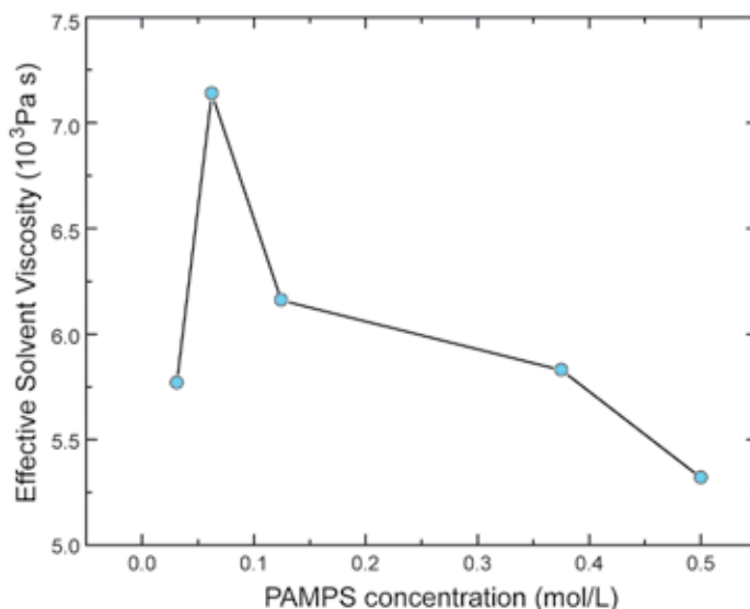
FIGURE 3: Effective solvent viscosity seen by PAMPS segment within PAMPS/PAAm solution blends. A maximum is also located at a PAMPS/ PAAm molar ratio of 1/ 7. [The line is a guide to the eye.]
