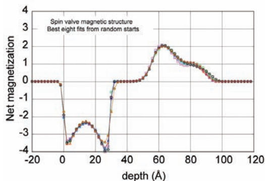
FIGURE 4: Freeform fits to the subsurface magnetic structure of a spin valve. Since the reflectometry inverse problem is not uniquely solvable, it is important to see the variety of solutions which fit the data. That these profiles are consistent gives us confidence that we have found the best solution within the constraints of the model.
