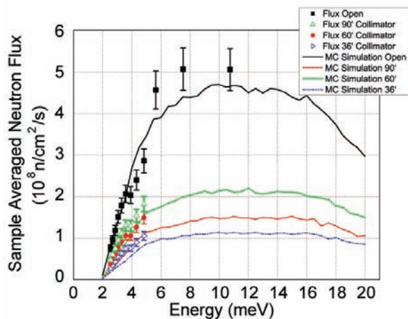
FIGURE 1: MACS flux on sample versus energy. The sample cross section was a rectangle 2 cm wide and 4 cm tall. The neutron flux for E < 5 meV were measured with a Be filter placed after the source. Measurements for E > 5 meV were taken without the Be filter and were corrected for \lambda/2 contamination. The solid lines are Monte Carlo Simulations. All beam line components from source to the sample position were simulated, excluding the filters. The error bars represent a conservative estimate of systematic errors.
