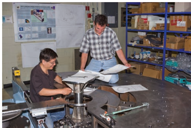
FIGURE 3: Mechanical Engineers Zheng Huang (University of Maryland) and Jim Moyer (NCNR) perform a dimensional check during assembly of the 6-axis sample positioning stage and 20-channel crystal analyzer/detector system for the MACS Spectrometer. Following complete assembly and testing, the system will be deployed at NG-0.
