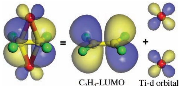
FIGURE 2: Optimized structure of an ethylene-Ti complex, C_2H_4Ti_2 , showing that Ti- C_2H_4 bonding orbital results from the hybridization of the LUMO of the C_2H_4 and the Ti- d orbital, in accord with Dewar coordination.
