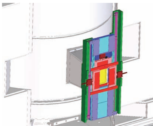
FIGURE 2: CAD Representation of the design for the MACS Pre-Sample Optics system to be installed between the Supermirror Guide and the Sample Position. The Pre-Sample Optics system will provide the capability to monitor the neutron flux exiting the supermirror guide, insert attenuators in the incident beam, and define the size of the beam to better match the size of the sample. The selection of attenuator and size of the aperture are remotely controlled by computer.
