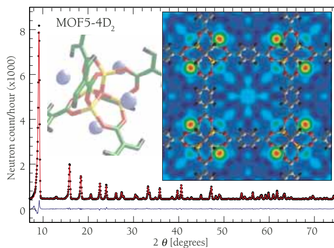
FIGURE 1: The neutron powder diffraction pattern ( \lambda = 2.08 Å) of the MOF5-4D 2 at 3.5 K (dots) plus the Rietveld refinement (solid red line) with space group Fm3m and a = 25.91 Å, and difference plot (solid blue line). The inset shows the real-space difference-Fourier scattering-length density superimposed on the MOF5 structure, indicating the location of cup-sites for the first hydrogen adsorption (red-yellow-green region).
