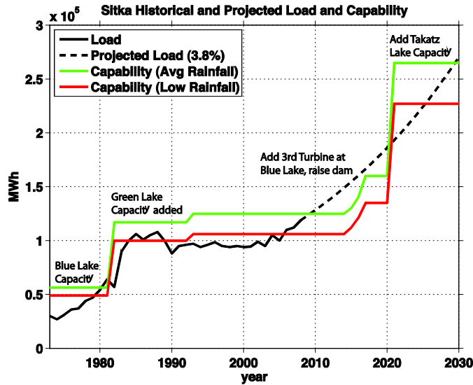
FIGURE 12: Historical and proposed capacity and generation in the Sitka, Alaska hydropower facility. Figure courtesy of Chris Brewton, Utility Director, City of Sitka.
