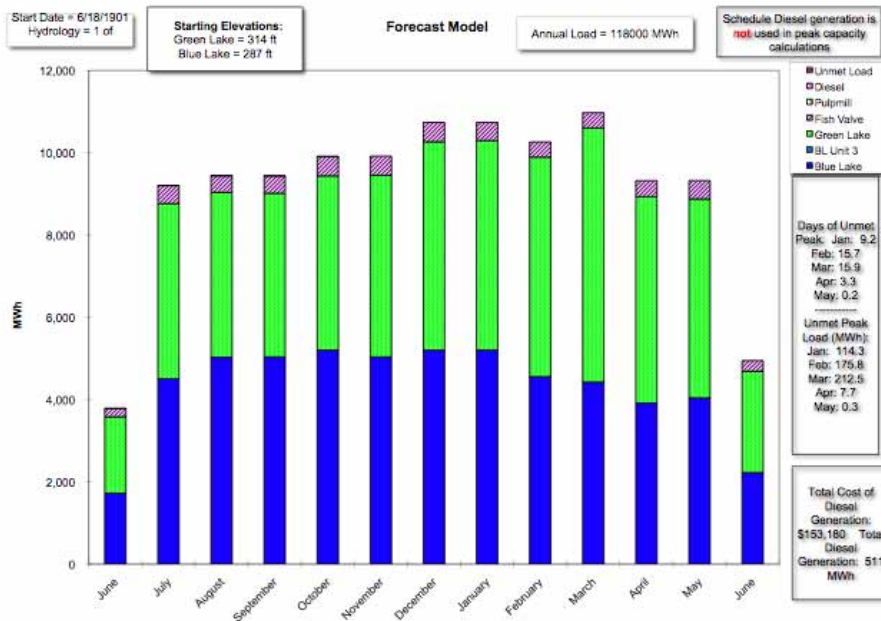
FIGURE 14: Example of a management year at the Sitka facility as modeled by the CHEOPS management software. Diesel generation is shown as a hatched purple bar. Blue and Green bars are MW-hr generated by the Blue and Green reservoirs, respectively.
