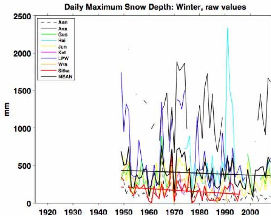
FIGURE 4: raw values for maximum winter snow depth at the stations typically located at sea-level airports. Multi-station means and trends lines are like those in the preceding figures.
