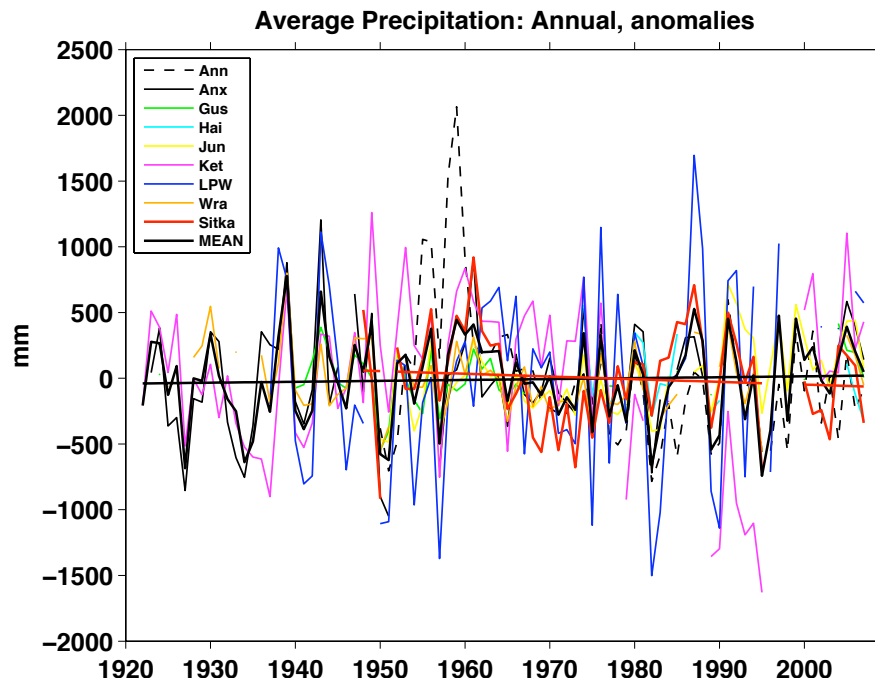
FIGURE 5: (a) raw values for annual means of monthly precipitation totals and (b) the corresponding anomalies. Multi-station means and trends lines are like those in the preceding figures.
