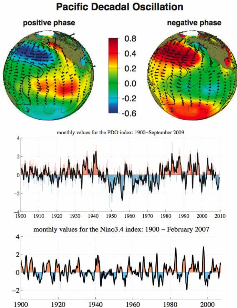
FIGURE 8: the Pacific Decadal Oscillation's pattern in space (a, b) and time (c), as well as the El Niño Southern Oscillation's pattern in time (d). The PDO index is defined using the principal component of North Pacific monthly sea surface temperature variability, as described in the text. The units in the top panel are anomalies in degrees C. Figures are reproduced from JISAO, 2010.
