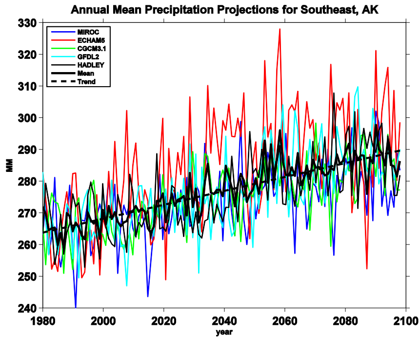
FIGURE 11: projected trends in precipitation from downscaled output of five climate models.
