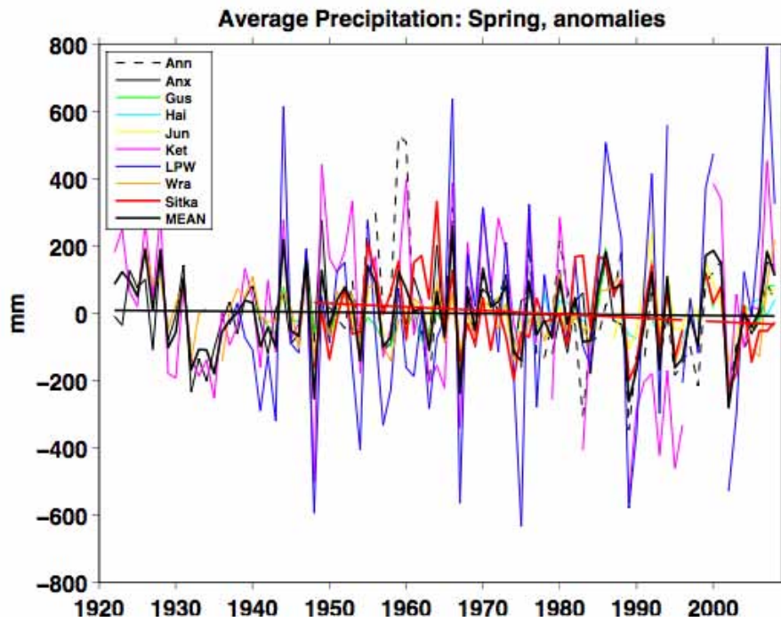
FIGURE 6: (a) raw values for spring means of monthly precipitation totals and (b) the corresponding anomalies. Multi-station means and trends lines are like those in the preceding figures.
