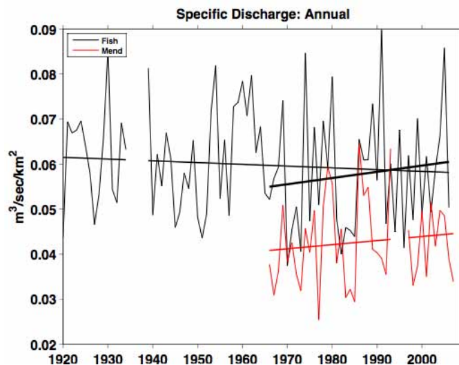
FIGURE 7: Annual specific discharge for two continuous records in Southeast Alaska. Trends are shown for Fish Creek for the whole period, as well as for the period for which that record overlaps with the record at Mendenhall.
