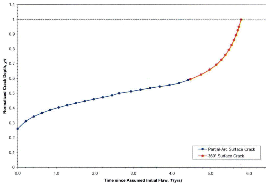
Figure 4-24 Phase I Surface Crack Depth as a Function of Time since Assumed Initial 26% Through-Wall Flaw
