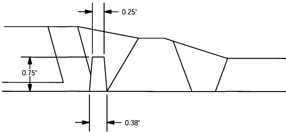
Figure 3-1 Type 1a Safety/Relief Nozzle Model Geometry
