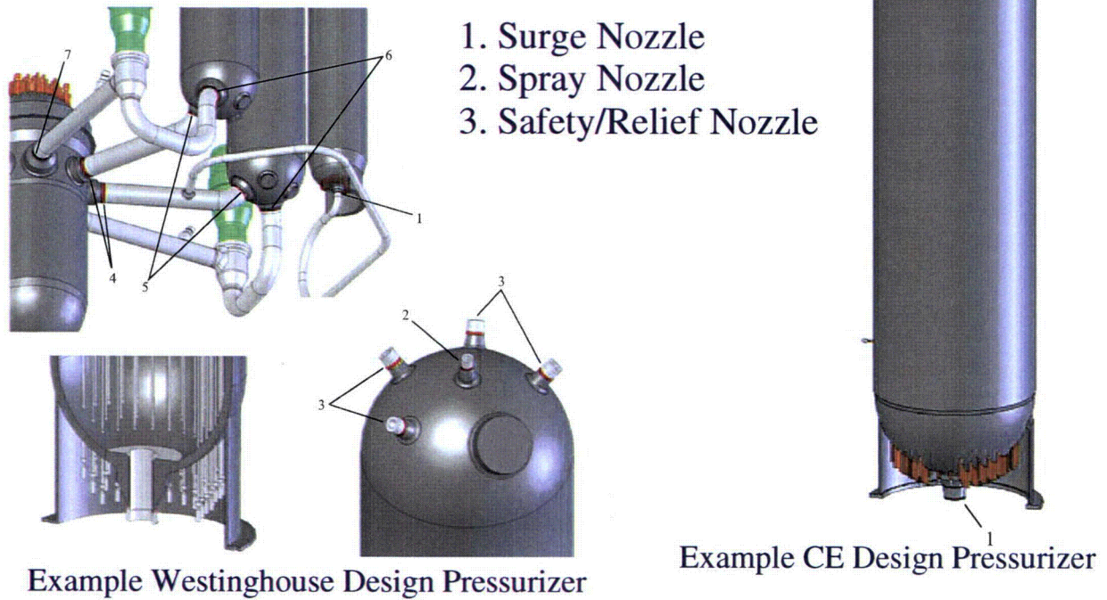
Figure 1-1 Pressurizer Nozzle Locations for Westinghouse and CE Design Plants
