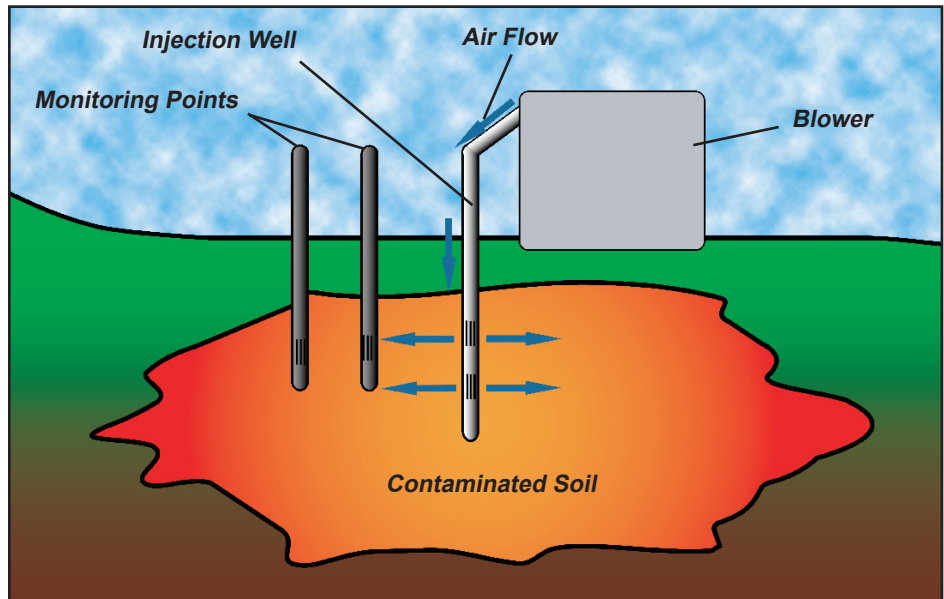
A conceptual model of a bioventing system.
