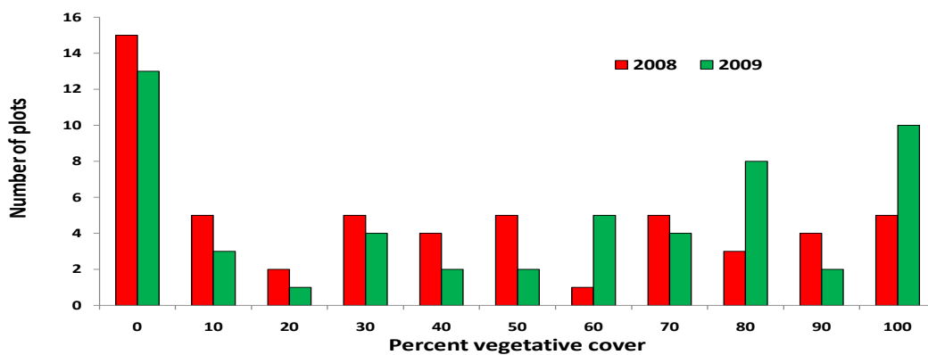
Figure 4.5.12 Comparison of distributions of percent cover for 54 fixed ½ m 2 plots along the Monie Bay transect in 2008 and 2009 (Haramis 2011, unpublished data).
