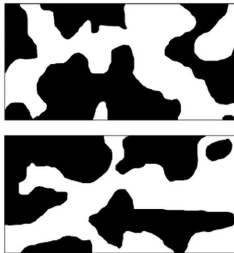
Figure 4.4.5 Digitized image of two 2 m 2 interior-marsh sites (dominated by Spartina alterniflora ), showing the hummocks in black and the hollows in white. Source: Stribling et al. (2006).
