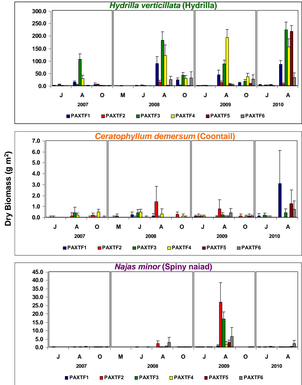
Figure 3.4.7 Hydrilla verticillata , Ceratophyllum demersum , and Najas minor dry biomass for six transects at Jug Bay sampled during June, August, and October from 2007-2010. Source: Delgado and Carroll (2010, unpublished data).
