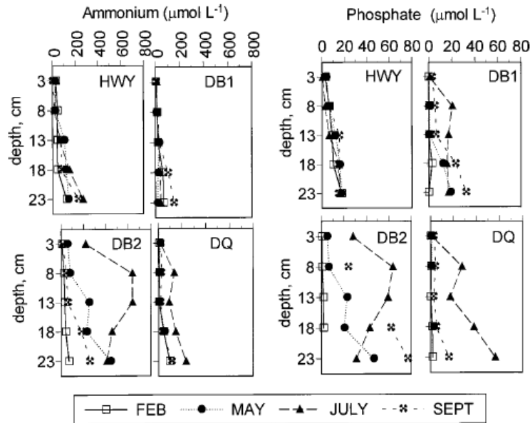
Figure 4.4.9 Vertical profiles of porewater ammonium and phosphate in Monie Creek tidal marsh sediments during the growing season. Stations are as noted in Table 4.4.3, except DQ, which is from the Dames Quarter marsh at the SW edge of Monie Bay. Source: Stribling and Cornwell (2001).
