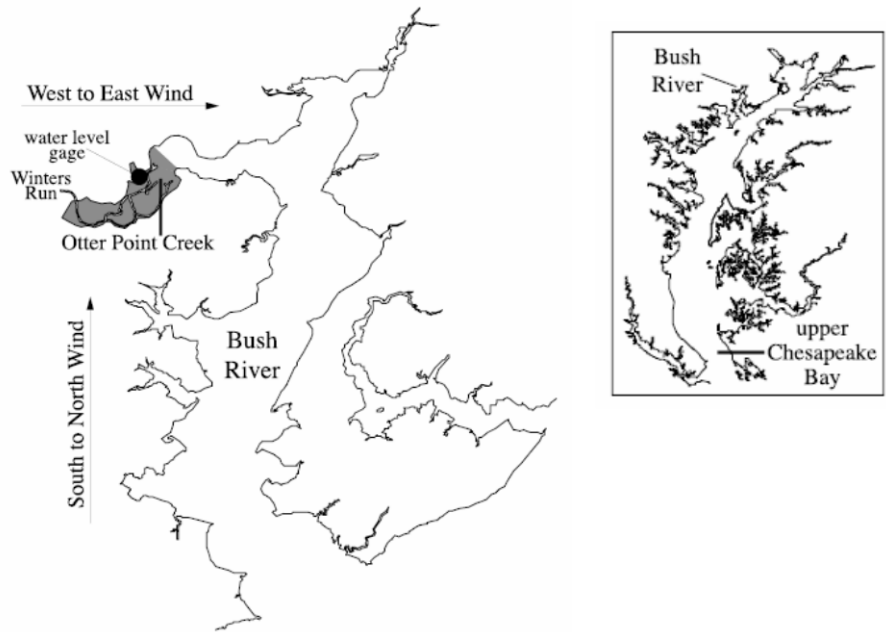
Figure 2.3.12 Main wind components affecting water levels in and around the OPC tidal freshwater marsh. Source: Pasternack and Hinnov (2003).
