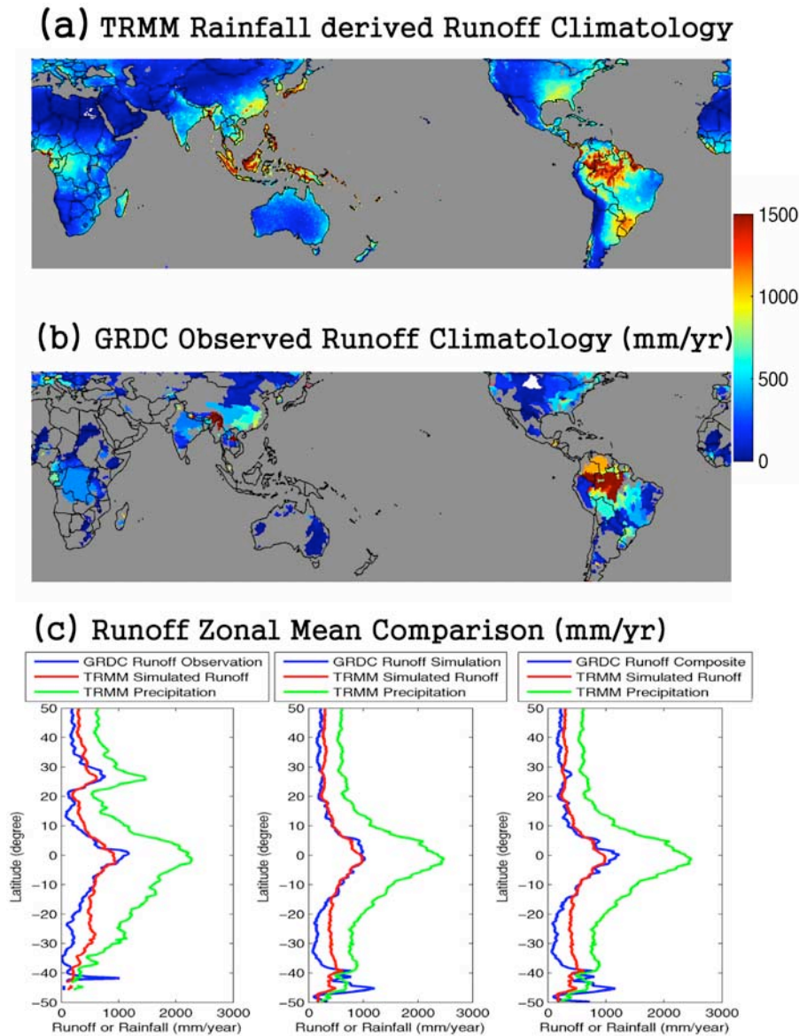
Figure 3. (a) Annual mean runoff (mm/yr) simulated using NRCS-CN methods from TRMM estimates for the period 1998–2006. (b) GRDC-observed runoff (mm/yr). (c) Runoff zonal mean profiles comparing TRMM precipitation (green) and simulated runoff (red) to GRDC runoff (blue) from the (left) observed, (middle) WBGs, and (right) composite data sets. Note the gray areas in Figures 3a and 3b indicate no data or water surface.
