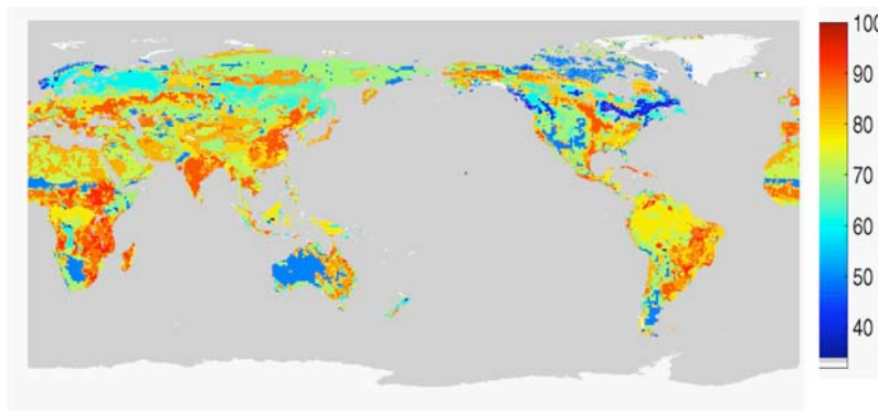
Figure 1. Global NRCS runoff curve number map derived from U.S. Department of Agriculture hydrological soil groups and land cover classification for fair hydrological conditions.
