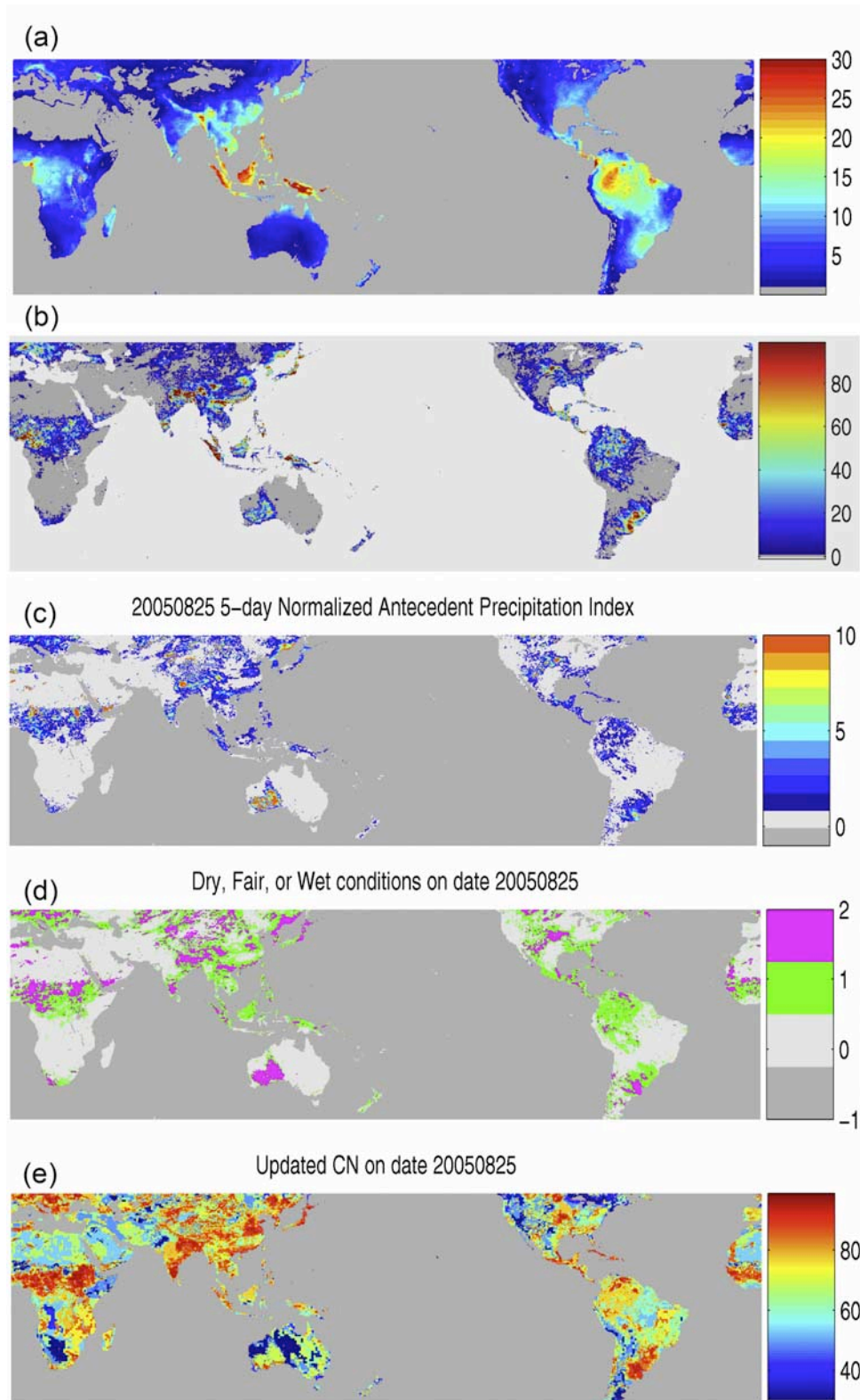
Figure 2. (a) Climatological pentad antecedent precipitation index (API) averaged over 9 years (1998–2006). (b) Pentad antecedent rainfall accumulation (mm) ending on 25 August 2005. (c) Pentad-normalized API (NAPI) on 25 August 2005. (d) Hydrological condition, with -1 , 0 , 1 , and 2 corresponding to no data, dry, fair, and wet conditions, respectively, determined by NAPI as of 25 August 2005. (e) Updated CN on 25 August 2005.
