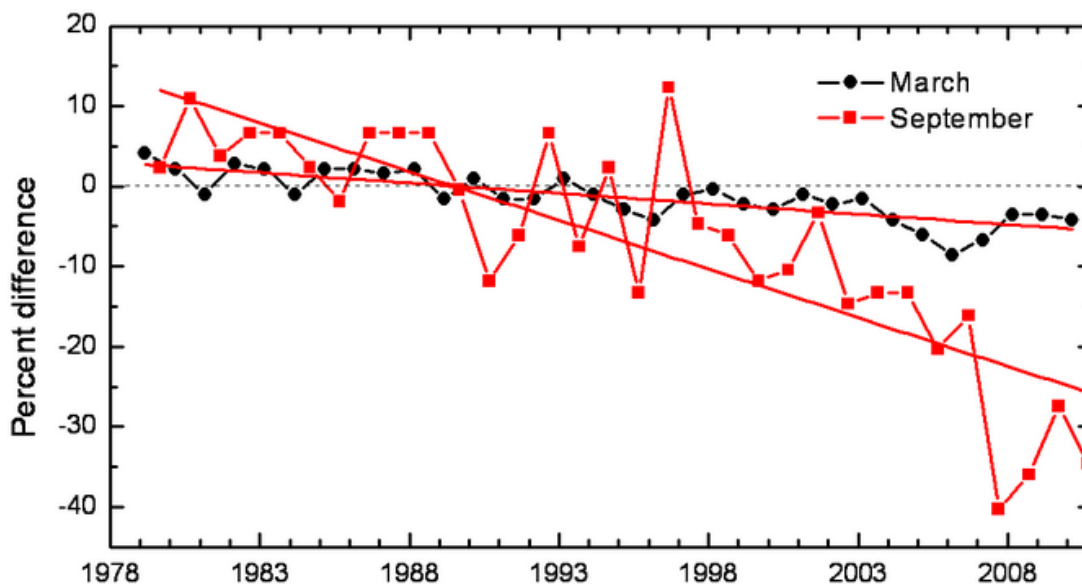
Figure I2. Time series of the percent difference in ice extent in March (the month of ice extent maximum) and September (the month of ice extent minimum) relative to the mean values for the period 1979–2000. Based on a least squares linear regression for the period 1979-2010, the rate of decrease for the March and September ice extents is -2.7\% and -11.6\% per decade, respectively.
