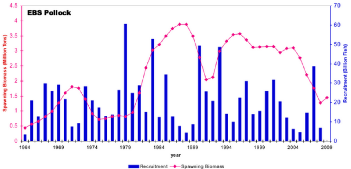
Figure F3. Bering Sea Pollock. Diamonds indicate biomass, and vertical bars indicate recruits to the population each year. From the NOAA/NMFS SAFE report .
