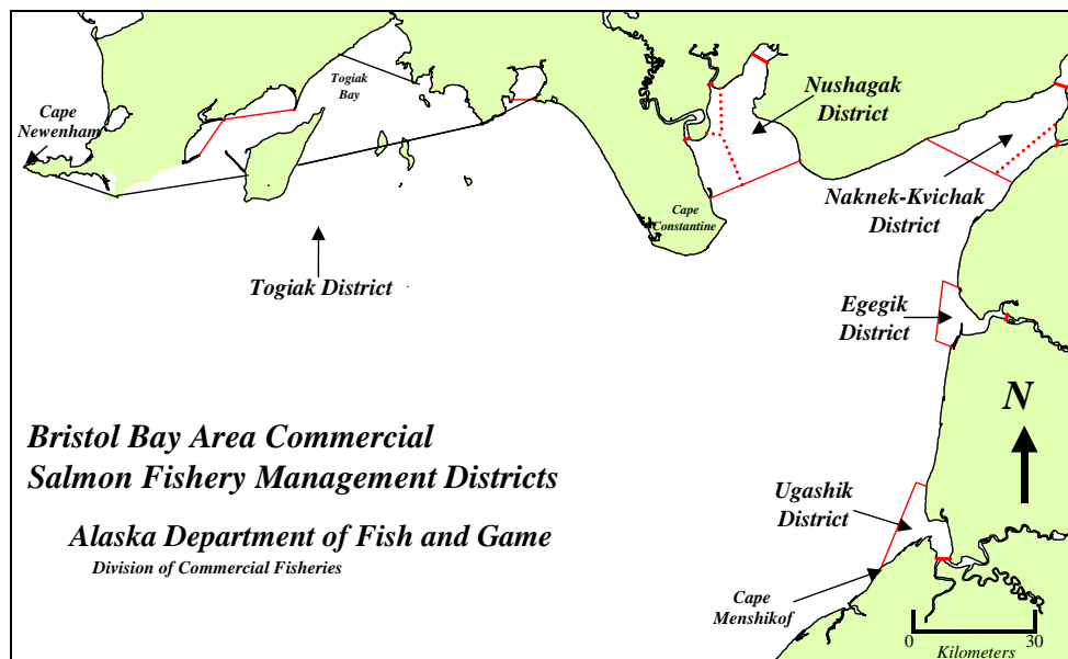
Figure 3-49 Bristol Bay area commercial fisheries salmon management districts.
