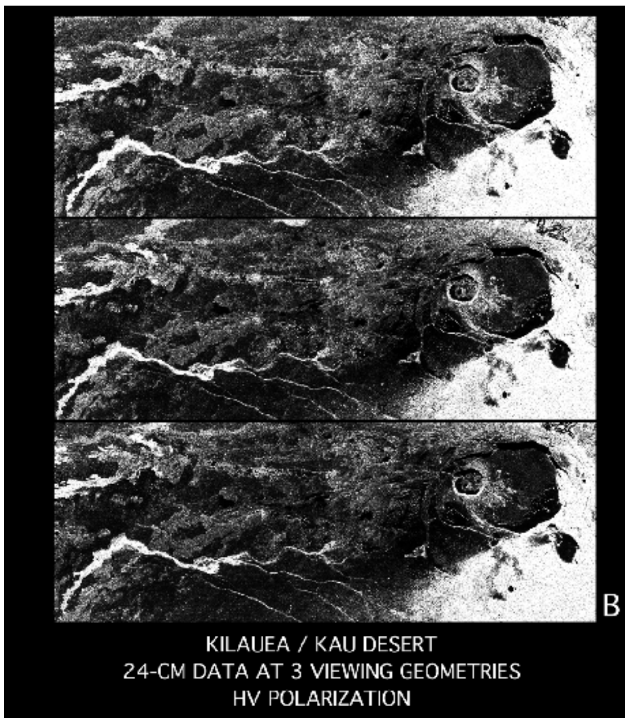
Figure 3. L-band (24-cm) HH- and HV-polarization radar images of Kilauea and the Kau desert.
