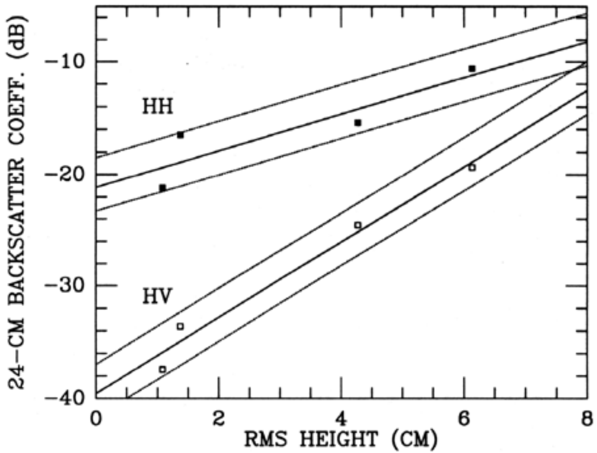
Figure 2. HH (horizontal transmit, horizontal receive) and HV (horizontal transmit, vertical receive) radar backscatter coefficients versus rms height for four lava flows in Hawaii.
