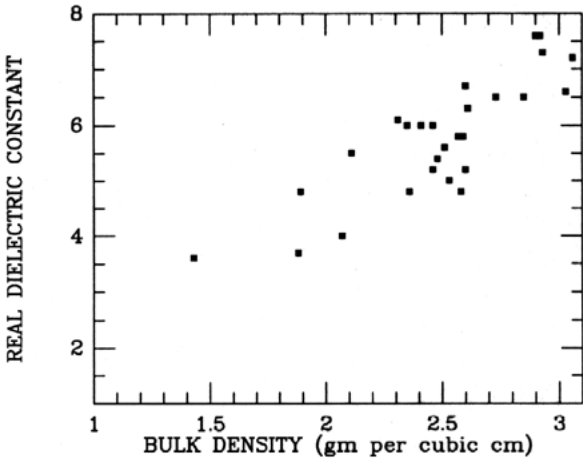
Figure 5. Plot of real dielectric constant ( ) versus bulk density for terrestrial volcanic rocks.
