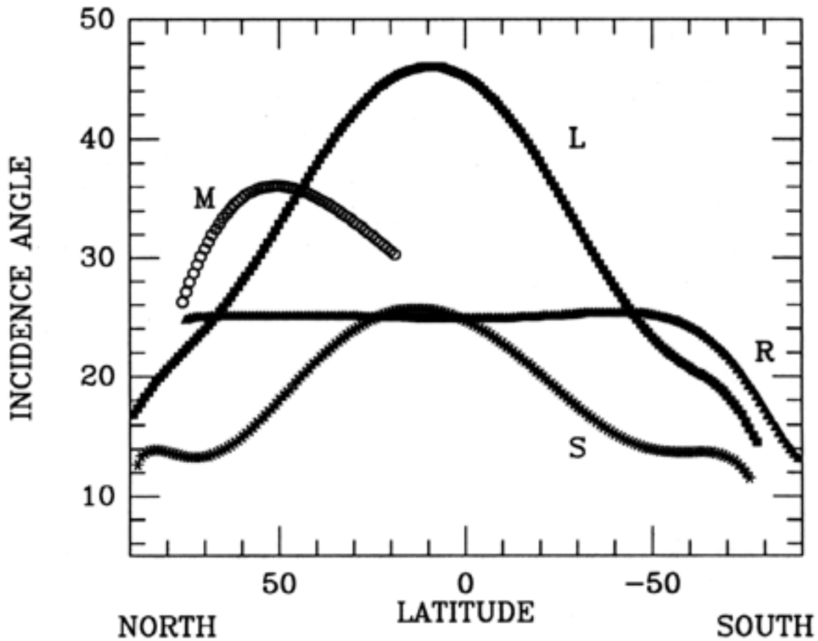
Figure 1. Plot of Magellan radar incidence angle versus latitude for four viewing geometry profiles used during the Magellan mission.
