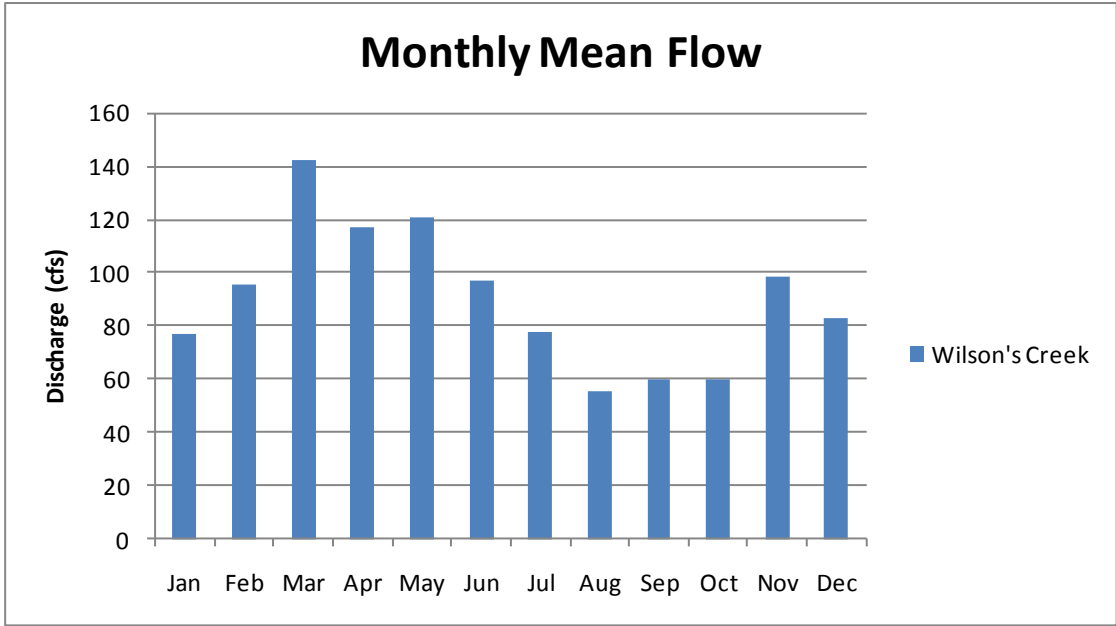
Figure 5-30. Mean monthly discharge (cubic feet per second) for monitoring station on Wilson's Creek.
