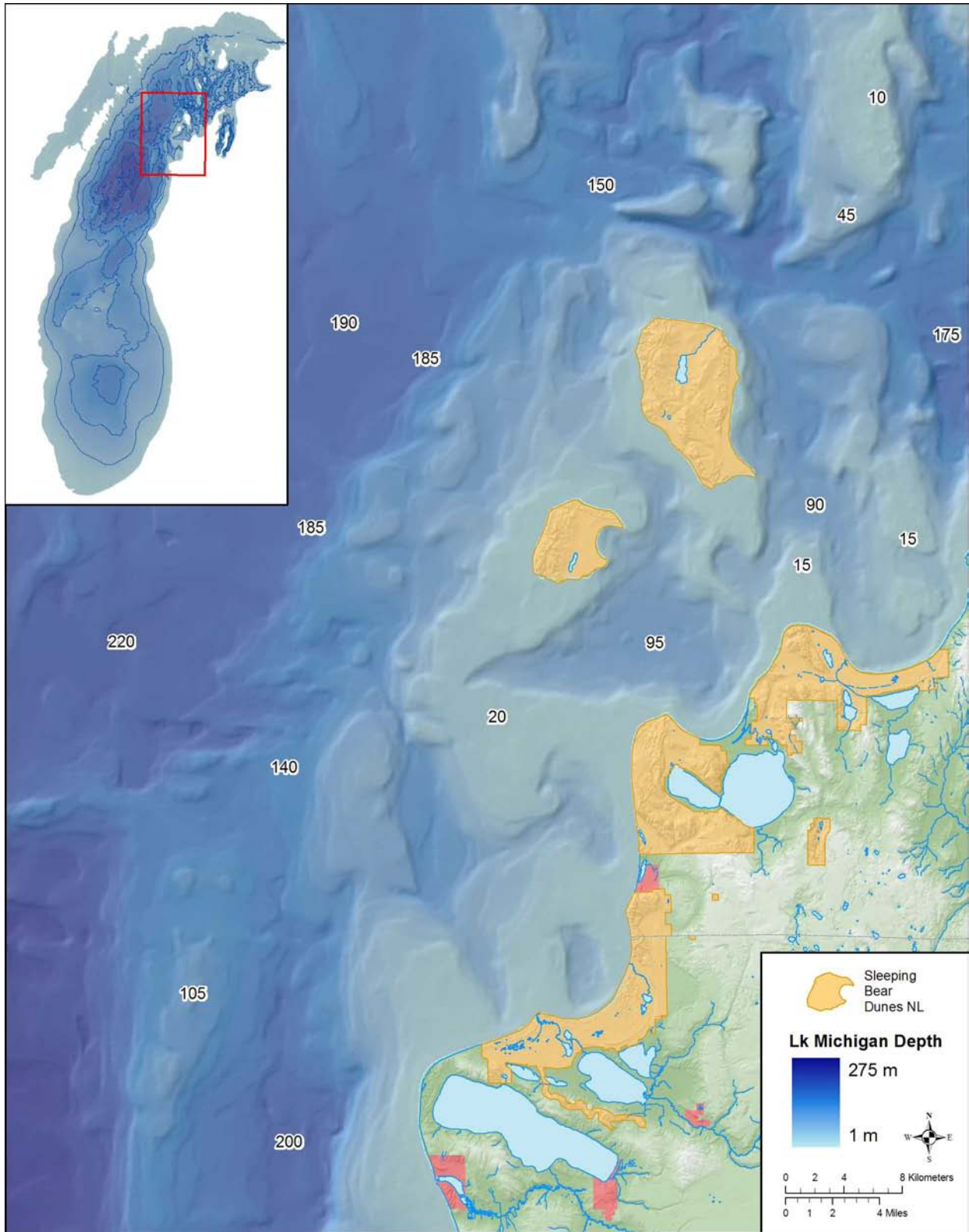
Figure 11. Lake Michigan bathymetry in the vicinity of Sleeping Bear Dunes National Lakeshore (MCGI n.d.; NGDC and GLERL 2006).
