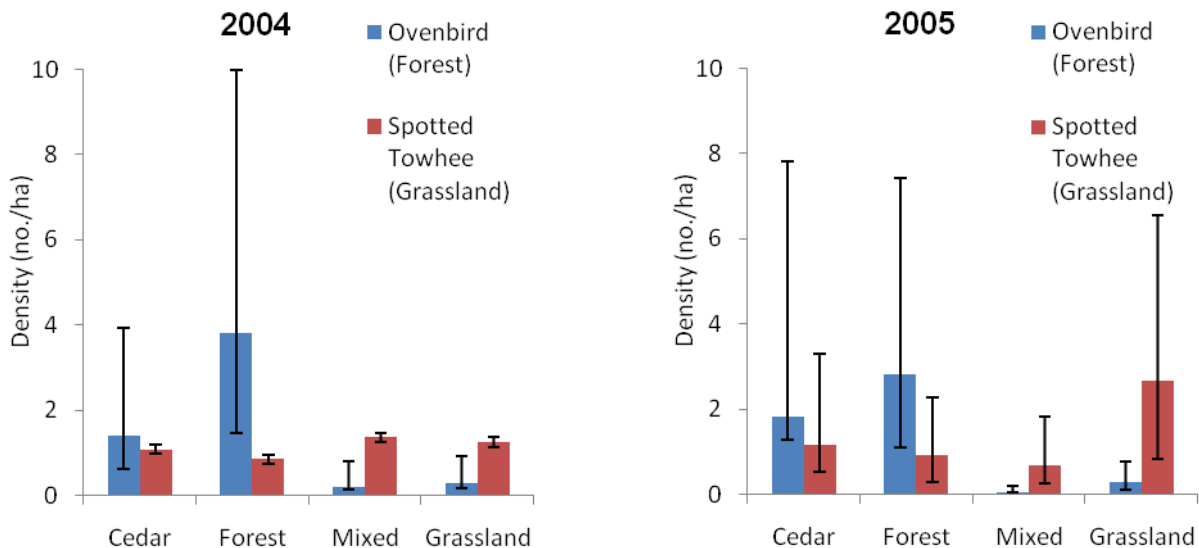
Figure 29. Mean density (no./ha) and 95 percent confidence interval during 2004 and 2005 for two songbird species in four habitat types in the Niobrara Valley Preserve ( Source: Frost 2007 ).
