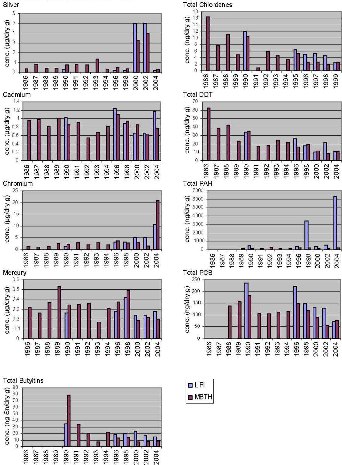
Figure 17. Temporal trends in total PAHs, PCBs, DDTs, Chlordanes, Butyl tins, Hg, Ag, Cd, and Cr (from NOAA Status and Trends Moriches Bay (MBTH) and Fire Island Inlet (LIFI) sites 1986 to 2004).
