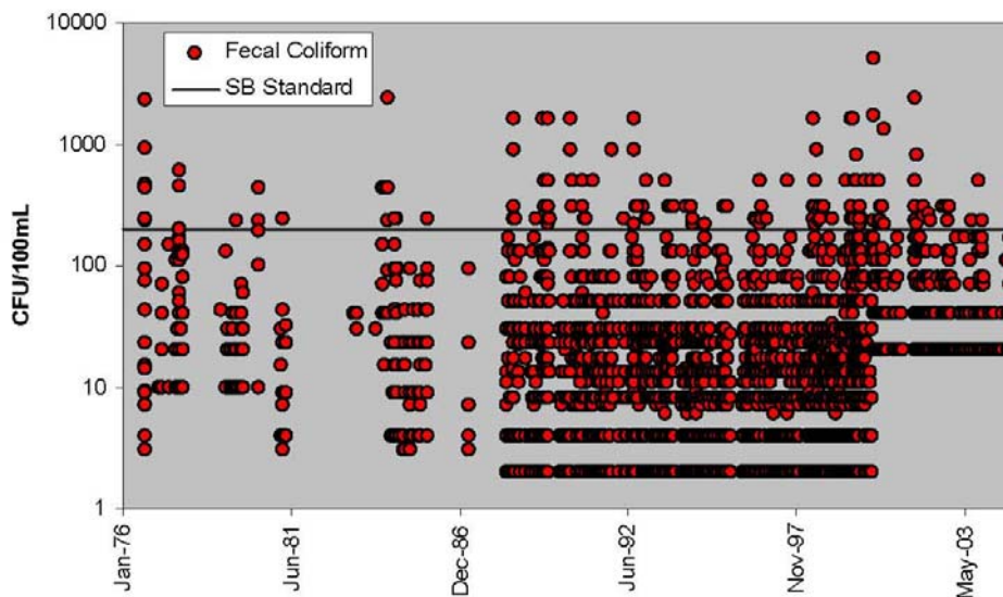
Figure 15. All fecal coliform data from SCDHS between 1976 and 2004.
