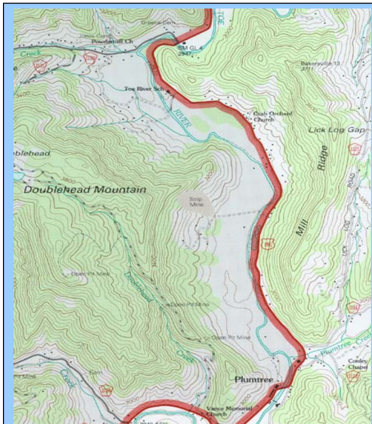
Fig. D.3-10 Natural Stream Dynamics Site, Plumtree, North Carolina EWP Program Site Map
